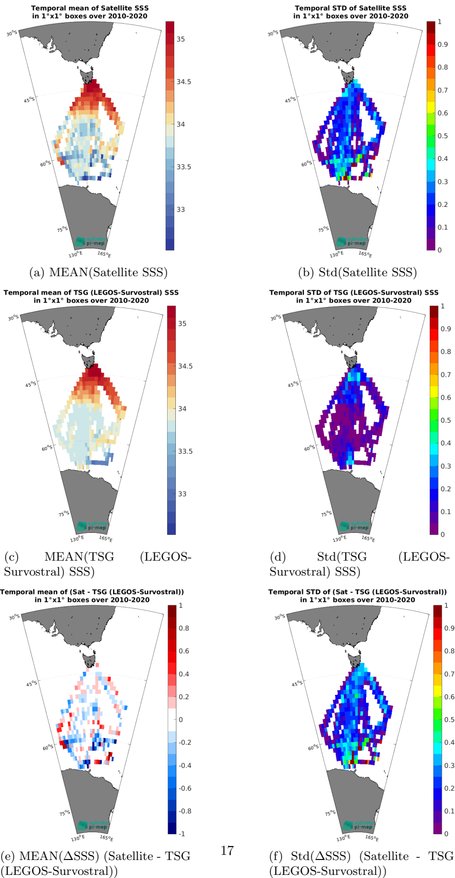
Figure 7: Temporal mean (left) and Std (right) of SSS from SMOS SSS L3 v9 - 9 Days (CATDS-CEC-LOCEAN) (top), TSG (LEGOS-Survostral) (middle), and of \Delta SSS (Satellite - TSG (LEGOS-Survostral)). Only match-up pairs are used to generate these maps.
