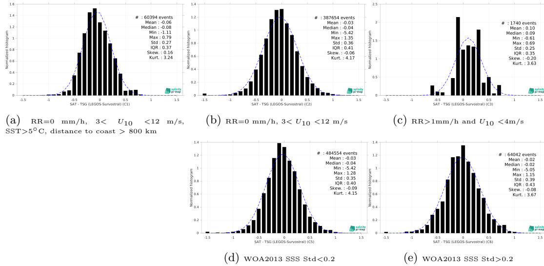
Figure 15: Normalized histogram of \Delta SSS (SMOS SSS L3 v9 - 9 Days (CATDS-CEC-LOCEAN) - TSG (LEGOS-Survostral)) for 5 different subdatasets corresponding to: RR=0 mm/h, 3 < U_{10} < 12 m/s, SST>5°C, distance to coast > 800 km (a), RR=0 mm/h, 3 < U_{10} < 12 m/s (b), RR>1mm/h and U_{10} < 4 m/s (c), WOA2013 SSS Std<0.2 (d), WOA2013 SSS Std>0.2 (e).
