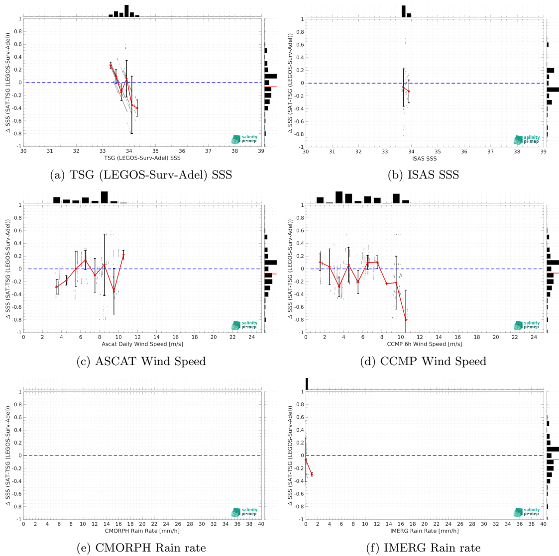
Figure 12: \Delta SSS (Satellite - TSG (LEGOS-Surv-Adel)) sorted as function of TSG (LEGOS-Surv-Adel) SSS values (a), ISAS SSS (b), ASCAT Wind speed (c), CCMP Wind speed (d), CMORPH rain rate (e) and IMERG rain rate (f). In all plots the median and Std of \Delta SSS for each bin is indicated by the red curves and black vertical thick bars ( \pm 1 Std).
