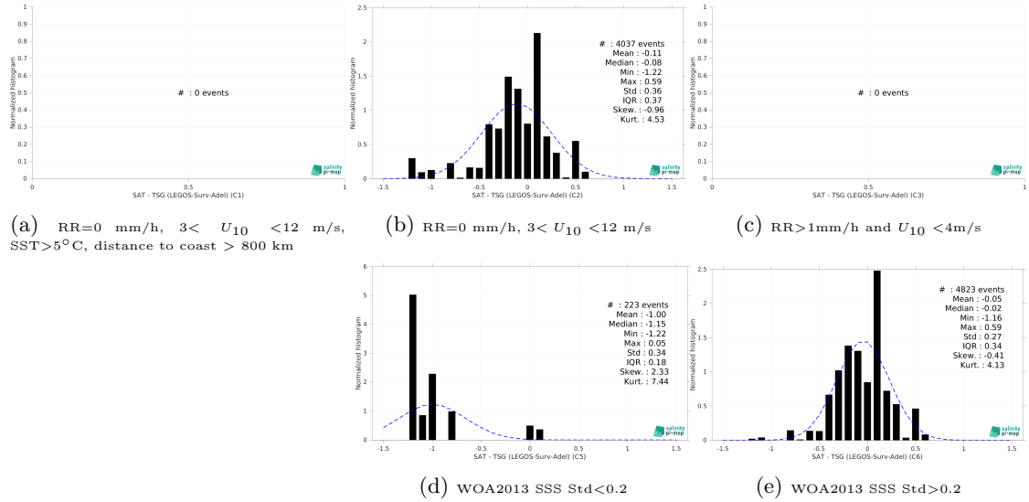
Figure 15: Normalized histogram of \Delta SSS (SMOS SSS L3 v9 - 9 Days (CATDS-CEC-LOCEAN) - TSG (LEGOS-Surv-Adel)) for 5 different subdatasets corresponding to: RR=0 mm/h, 3 < U_{10} < 12 m/s, SST > 5°C, distance to coast > 800 km (a), RR=0 mm/h, 3 < U_{10} < 12 m/s (b), RR > 1mm/h and U_{10} < 4 m/s (c), WOA2013 SSS Std < 0.2 (d), WOA2013 SSS Std > 0.2 (e).
