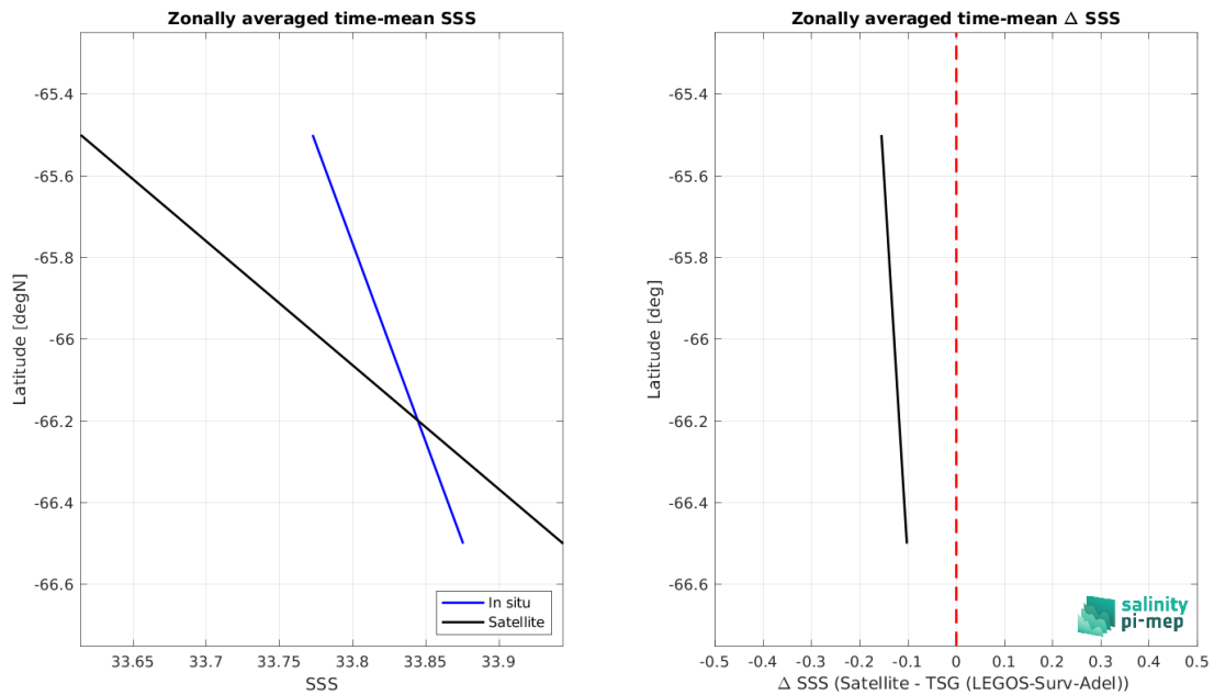
Figure 9: Left panel: Zonal mean SSS from SMOS SSS L3 v9 - 9 Days (CATDS-CEC-LOCEAN) satellite product (black) and from TSG (LEGOS-Surv-Adel) (blue). Right panel: Zonal mean of \Delta SSS (Satellite - TSG (LEGOS-Surv-Adel)) for all the collected Pi-MEP match-up pairs estimated over the full satellite product period.
