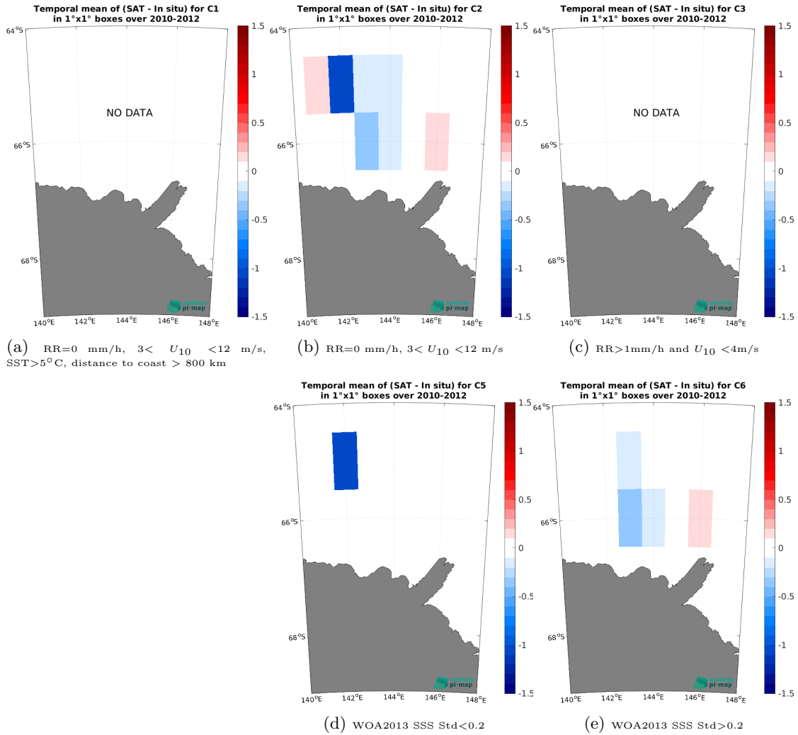
Figure 14: Temporal mean gridded over spatial boxes of size 1^\circ \times 1^\circ of \Delta\text{SSS} (SMOS SSS L3 v9 - 9 Days (CATDS-CEC-LOCEAN) - TSG (LEGOS-Surv-Adel)) for 5 different subdatasets corresponding to: RR=0 mm/h, 3 < U_{10} < 12 m/s, SST >5^\circ\text{C} , distance to coast > 800 km (a), RR=0 mm/h, 3 < U_{10} < 12 m/s (b), RR >1 mm/h and U_{10} < 4 m/s (c), WOA2013 SSS Std <0.2 (d), WOA2013 SSS Std >0.2 (e).
