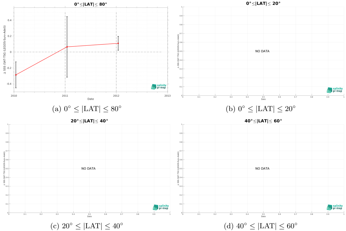
Figure 11: Monthly median (red curves) of \Delta SSS (Satellite - TSG (LEGOS-Surv-Adel)) and \pm 1 Std (black vertical thick bars) as function of time for all the collected Pi-MEP match-up pairs estimated over the Global Ocean Pi-MEP region and for the full satellite product period are shown for different latitude bands: (a) 80^\circ\text{S}-80^\circ\text{N} , (b) 20^\circ\text{S}-20^\circ\text{N} , (c) 40^\circ\text{S}-20^\circ\text{S} and 20^\circ\text{N}-40^\circ\text{N} and (d) 60^\circ\text{S}-40^\circ\text{S} and 40^\circ\text{N}-60^\circ\text{N} .
