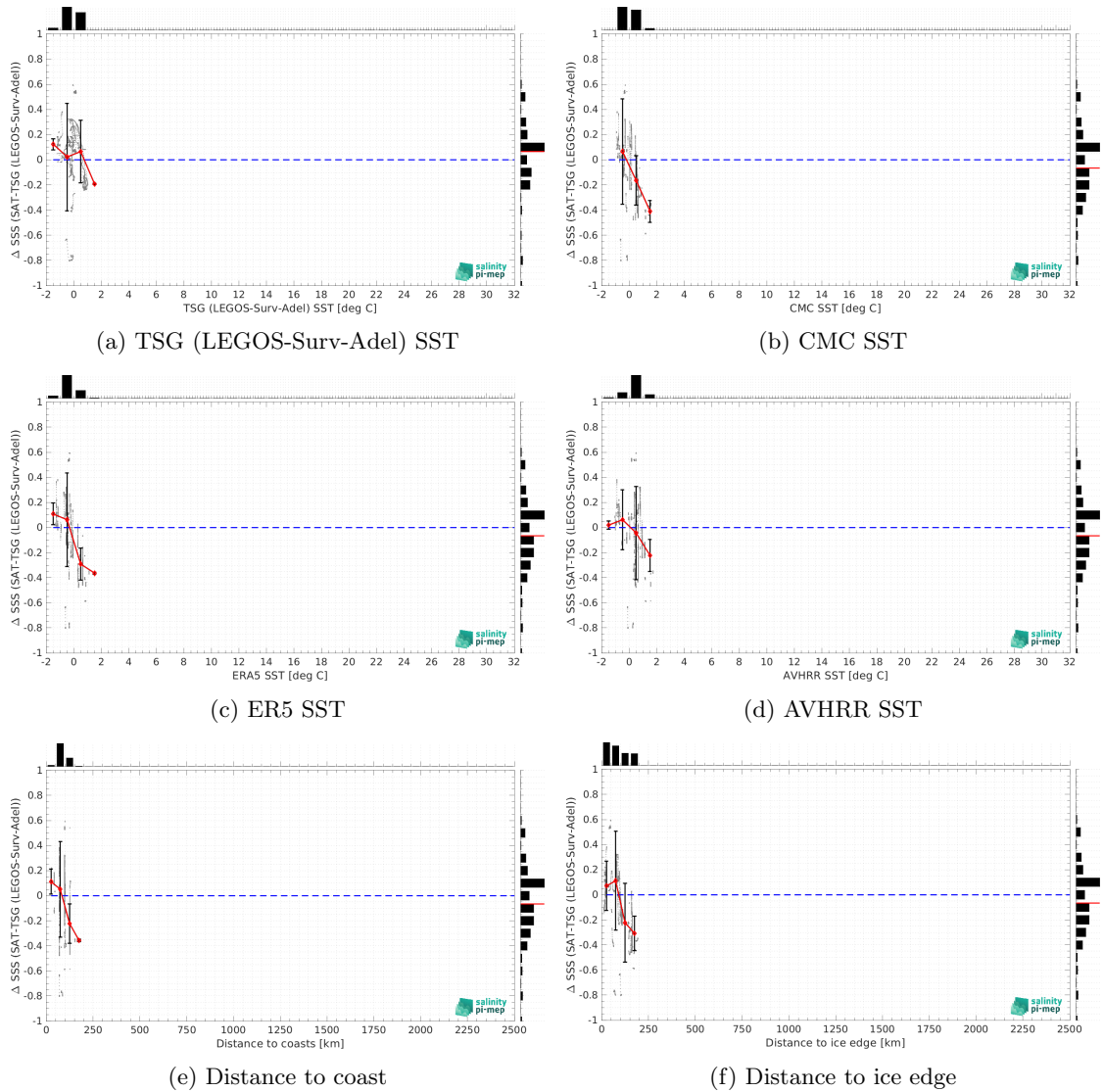
Figure 13: \Delta SSS (Satellite - TSG (LEGOS-Surv-Adel)) sorted as function of TSG (LEGOS-Surv-Adel) SST values (a), CMC SST (b), ERA5 SST (c), AVHRR SST (d), distance to coast (e) and distance to ice edge (f). In all plots the median and Std of \Delta SSS for each bin is indicated by the red curves and black vertical thick bars ( \pm 1 Std). Links to similar figures sorted as function of Sea ice fraction and in situ measurement depth .
