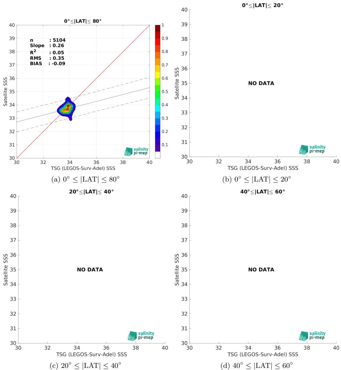
Figure 10: Contour maps of the concentration of SMOS SSS L3 v9 - 9 Days (CATDS-CEC-LOCEAN) SSS (y-axis) versus TSG (LEGOS-Surv-Adel) SSS (x-axis) at match-up pairs for different latitude bands. For each plot, the red line shows x=y . The black thin and dashed lines indicate a linear fit through the data cloud and the \pm 95\% confidence levels, respectively. The number match-up pairs n , the slope and R^2 coefficient of the linear fit, the root mean square (RMS) and the mean bias between satellite and in situ data are indicated for each latitude band in each plots.
