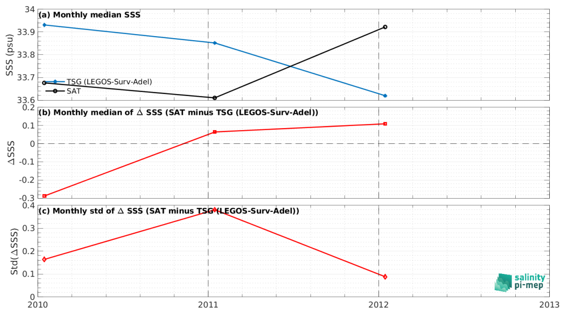
Figure 8: Time series of the monthly median SSS (top), median of \Delta SSS (Satellite - TSG (LEGOS-Surv-Adel)) and Std of \Delta SSS (Satellite - TSG (LEGOS-Surv-Adel)) over the Global Ocean Pi-MEP region considering all match-ups collected by the Pi-MEP.
