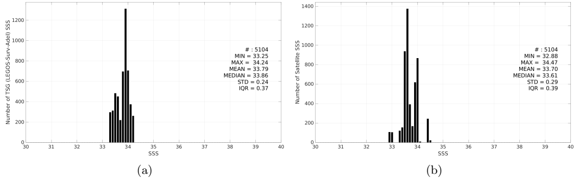
Figure 2: Histograms of SSS from TSG (LEGOS-Surv-Adel) (a) and SMOS SSS L3 v9 - 9 Days (CATDS-CEC-LOCEAN) (b) considering all match-up pairs per bins of 0.1 over the Global Ocean Pi-MEP region and for the full satellite product period.
