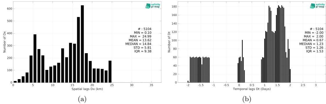
Figure 5: Histograms of the spatial (a) and temporal (b) lags between the location/time of the TSG (LEGOS-Surv-Adel) measurement and the date of the corresponding SMOS SSS L3 v9 - 9 Days (CATDS-CEC-LOCEAN) SSS pixel.
