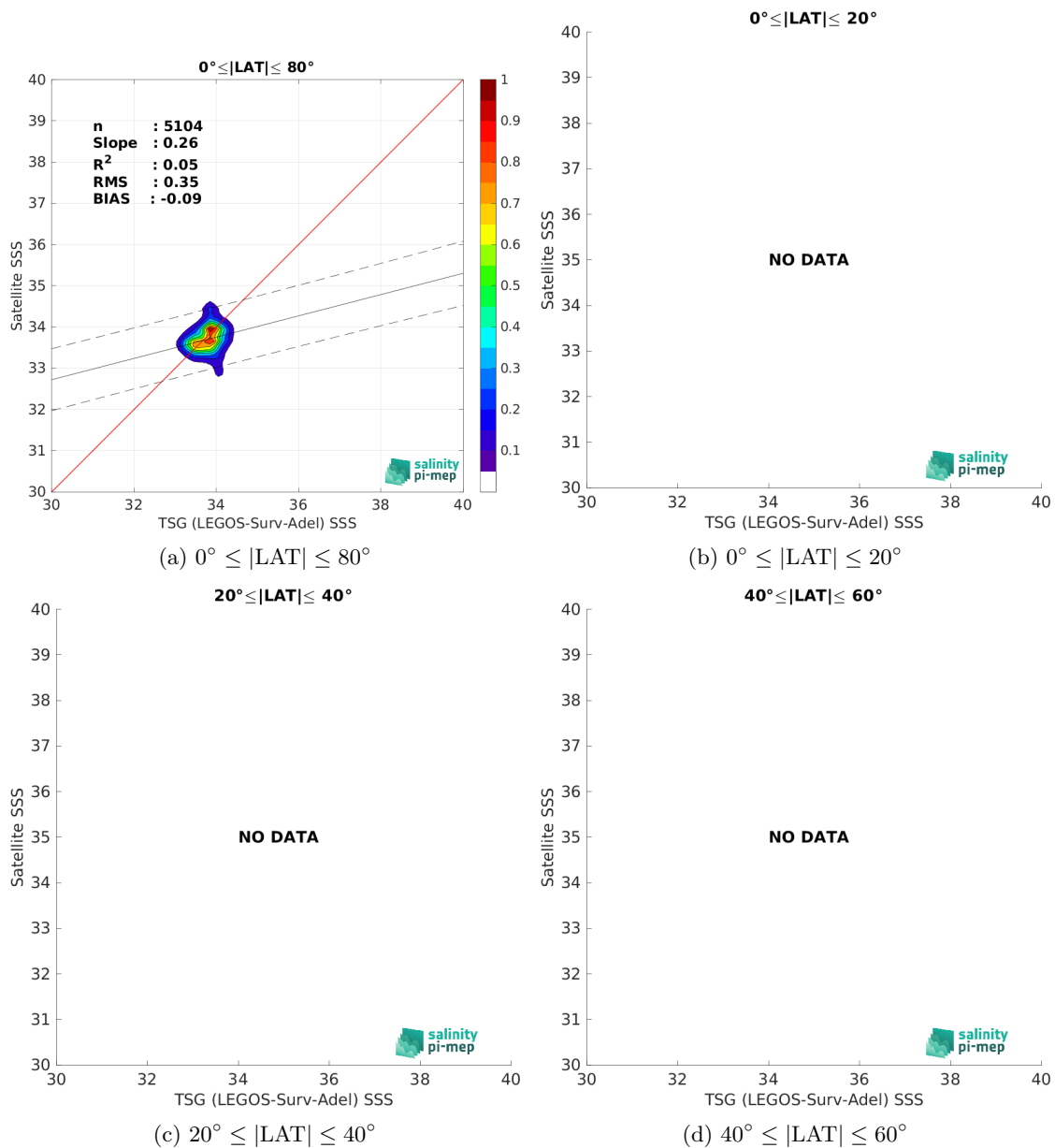
Figure 9: Contour maps of the concentration of SMOS SSS L3 v9 - 9 Days (CATDS-CEC-LOCEAN) SSS (y-axis) versus TSG (LEGOS-Surv-Adel) SSS (x-axis) at match-up pairs for different latitude bands. For each plot, the red line shows x=y . The black thin and dashed lines indicate a linear fit through the data cloud and the \pm 95\% confidence levels, respectively. The number match-up pairs n , the slope and R^2 coefficient of the linear fit, the root mean square (RMS) and the mean bias between satellite and in situ data are indicated for each latitude band in each plots.
