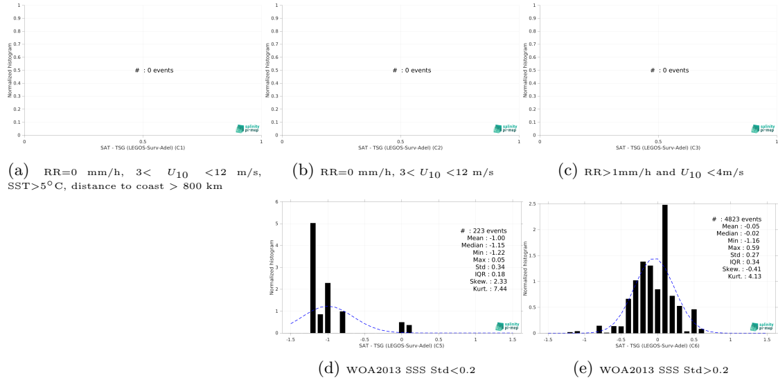
Figure 13: Normalized histogram of \Delta SSS (SMOS SSS L3 v9 - 9 Days (CATDS-CEC-LOCEAN) - TSG (LEGOS-Surv-Adel)) for 5 different subdatasets corresponding to: RR=0 mm/h, 3 < U_{10} < 12 m/s, SST > 5°C, distance to coast > 800 km (a), RR=0 mm/h, 3 < U_{10} < 12 m/s (b), RR > 1mm/h and U_{10} < 4 m/s (c), WOA2013 SSS Std < 0.2 (d), WOA2013 SSS Std > 0.2 (e).
