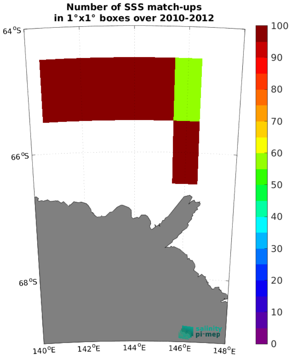
Figure 4: Number of SSS match-ups between TSG (LEGOS-Surv-Adel) SSS and the SMOS SSS L3 v9 - 9 Days (CATDS-CEC-LOCEAN) SSS product for the Global Ocean Pi-MEP region over 1°×1° boxes and for the full satellite product period.
