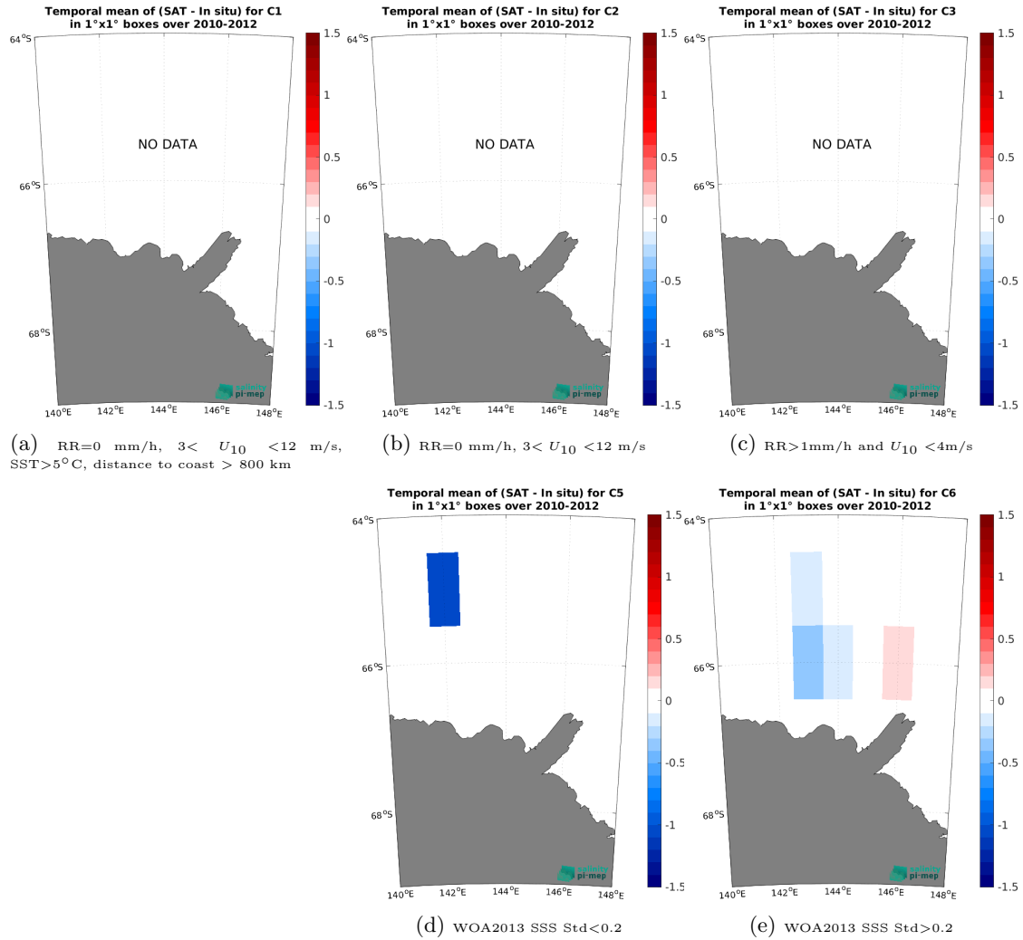
Figure 12: Temporal mean gridded over spatial boxes of size 1^\circ \times 1^\circ of \Delta SSS (SMOS SSS L3 v9 - 9 Days (CATDS-CEC-LOCEAN) - TSG (LEGOS-Surv-Adel)) for 5 different subdatasets corresponding to: RR=0 mm/h, 3 < U_{10} < 12 m/s, SST>5°C, distance to coast > 800 km (a), RR=0 mm/h, 3 < U_{10} < 12 m/s (b), RR>1mm/h and U_{10} < 4 m/s (c), WOA2013 SSS Std<0.2 (d), WOA2013 SSS Std>0.2 (e).
