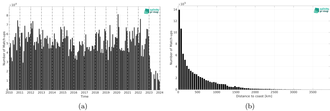
Figure 2: Number of match-ups between TSG (LEGOS-DM) and SMOS SSS L3 v9 - 9 Days (CATDS-CEC-LOCEAN) SSS as a function of time (a) and as function of the distance to coast (b) over the Global Ocean Pi-MEP region and for the full satellite product period.
