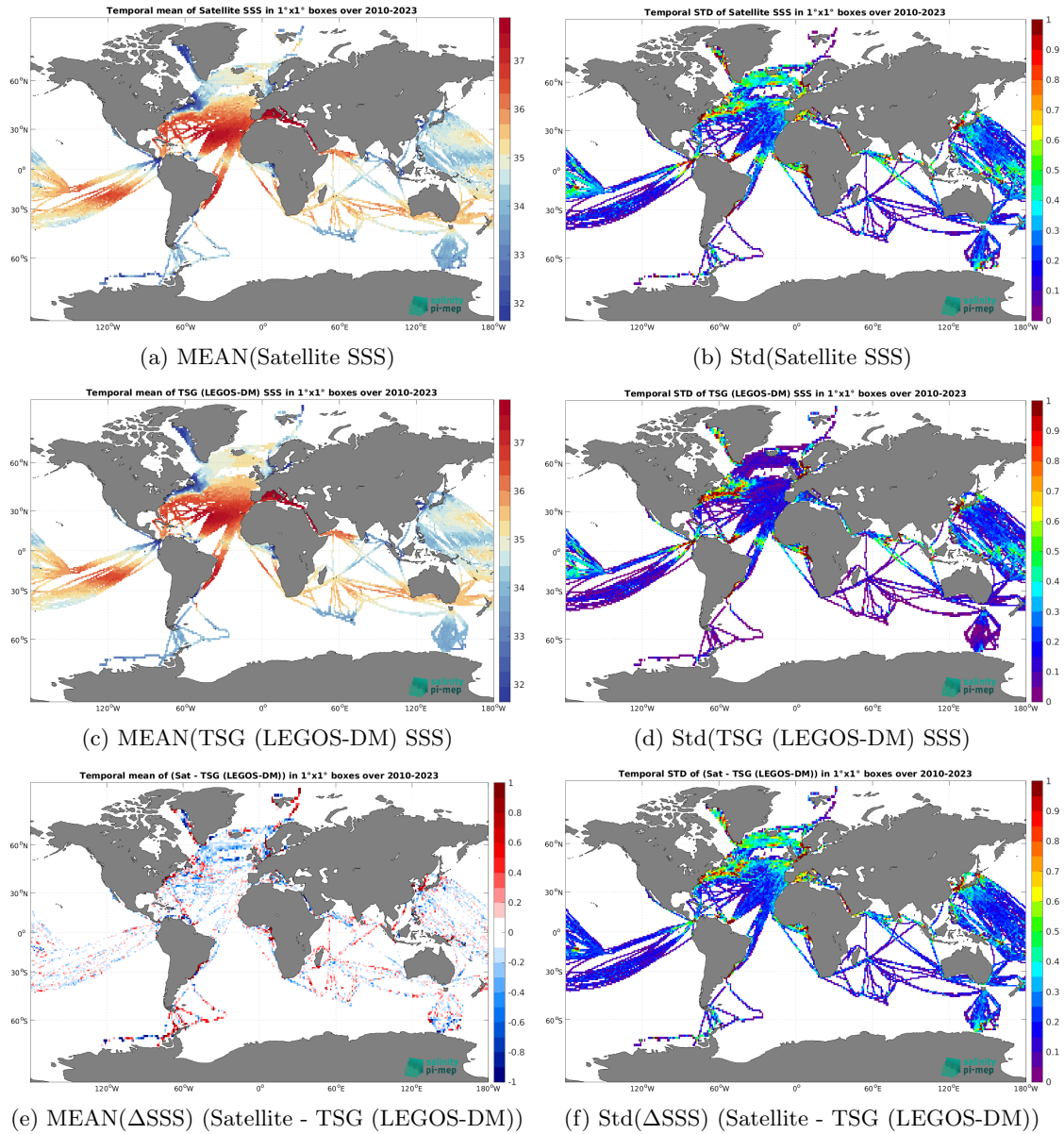
Figure 7: Temporal mean (left) and Std (right) of SSS from SMOS SSS L3 v9 - 9 Days (CATDS-CEC-LOCEAN) (top), TSG (LEGOS-DM) (middle), and of \Delta SSS (Satellite - TSG (LEGOS-DM)). Only match-up pairs are used to generate these maps.
