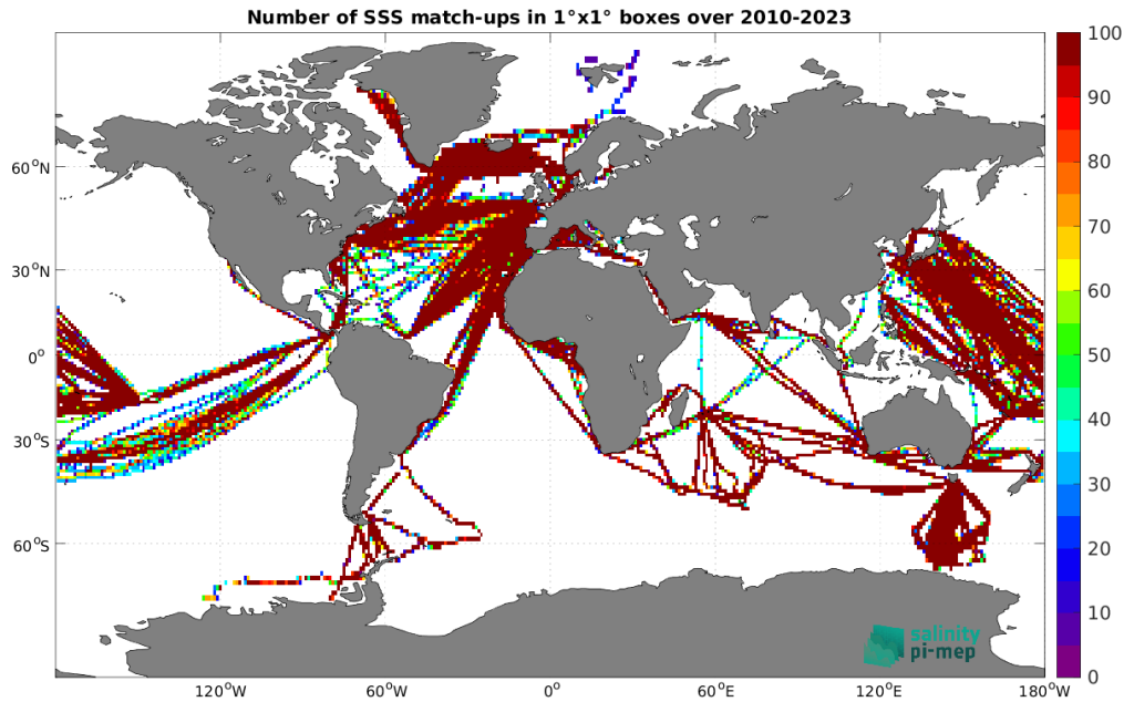
Figure 5: Number of SSS match-ups between TSG (LEGOS-DM) SSS and the SMOS SSS L3 v9 - 9 Days (CATDS-CEC-LOCEAN) SSS product for the Global Ocean Pi-MEP region over 1^\circ \times 1^\circ boxes and for the full satellite product period.
