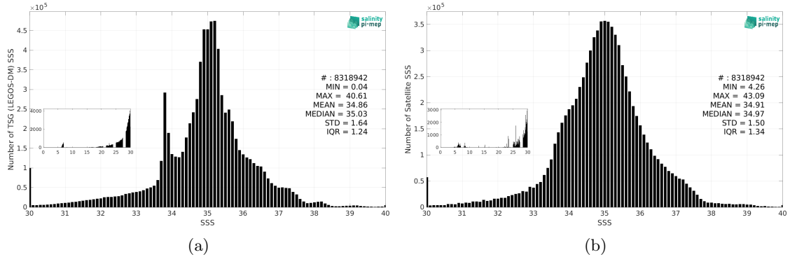
Figure 3: Histograms of SSS from TSG (LEGOS-DM) (a) and SMOS SSS L3 v9 - 9 Days (CATDS-CEC-LOCEAN) (b) considering all match-up pairs per bins of 0.1 over the Global Ocean Pi-MEP region and for the full satellite product period.
