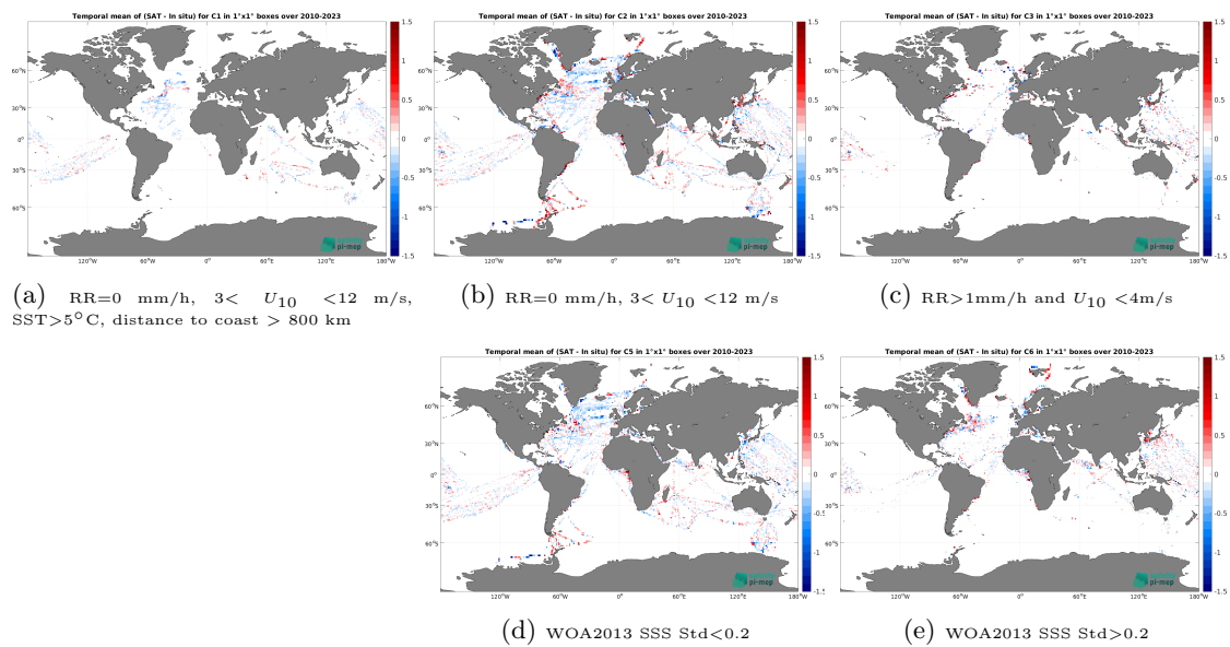
Figure 14: Temporal mean gridded over spatial boxes of size 1^\circ \times 1^\circ of \Delta SSS (SMOS SSS L3 v9 - 9 Days (CATDS-CEC-LOCEAN) - TSG (LEGOS-DM)) for 5 different subdatasets corresponding to:RR=0 mm/h, 3 < U_{10} < 12 m/s, SST >5^\circ C, distance to coast > 800 km (a), RR=0 mm/h, 3 < U_{10} < 12 m/s (b), RR >1 mm/h and U_{10} < 4 m/s (c), WOA2013 SSS Std <0.2 (d), WOA2013 SSS Std >0.2 (e).
