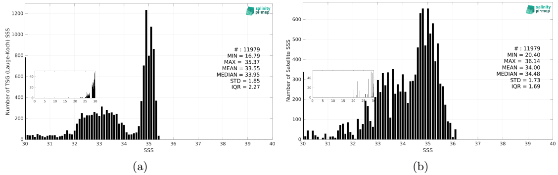
Figure 3: Histograms of SSS from TSG (Lauge-Koch) (a) and SMOS SSS L3 v9 - 9 Days (CATDS-CEC-LOCEAN) (b) considering all match-up pairs per bins of 0.1 over the Global Ocean Pi-MEP region and for the full satellite product period.
