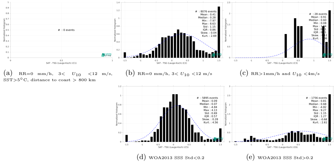
Figure 15: Normalized histogram of \Delta SSS (SMOS SSS L3 v9 - 9 Days (CATDS-CEC-LOCEAN) - TSG (Lauge-Koch)) for 5 different subdatasets corresponding to: RR=0 mm/h, 3 < U_{10} < 12 m/s, SST>5°C, distance to coast > 800 km (a), RR=0 mm/h, 3 < U_{10} < 12 m/s (b), RR>1mm/h and U_{10} < 4 m/s (c), WOA2013 SSS Std<0.2 (d), WOA2013 SSS Std>0.2 (e).
