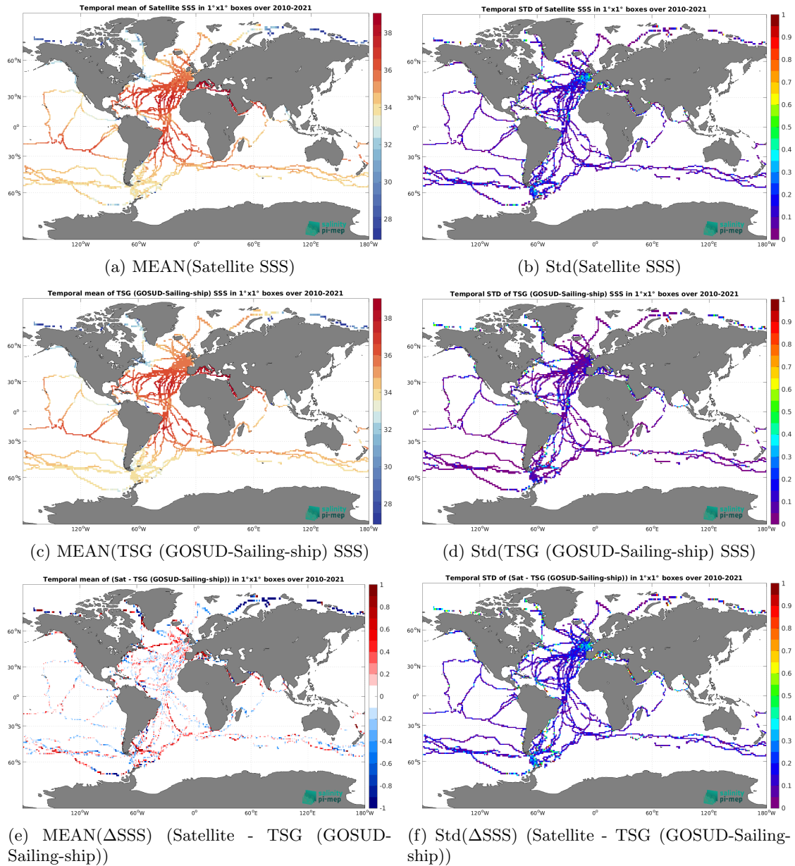
Figure 7: Temporal mean (left) and Std (right) of SSS from SMOS SSS L3 v9 - 9 Days (CATDS-CEC-LOCEAN) (top), TSG (GOSUD-Sailing-ship) (middle), and of \Delta SSS (Satellite - TSG (GOSUD-Sailing-ship)). Only match-up pairs are used to generate these maps.
