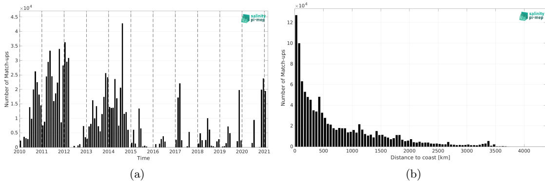
Figure 2: Number of match-ups between TSG (GOSUD-Sailing-ship) and SMOS SSS L3 v9 - 9 Days (CATDS-CEC-LOCEAN) SSS as a function of time (a) and as function of the distance to coast (b) over the Global Ocean Pi-MEP region and for the full satellite product period.
