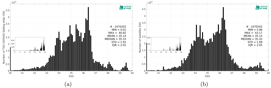
Figure 3: Histograms of SSS from TSG (GOSUD-Sailing-ship) (a) and SMOS SSS L3 v9 - 9 Days (CATDS-CEC-LOCEAN) (b) considering all match-up pairs per bins of 0.1 over the Global Ocean Pi-MEP region and for the full satellite product period.
