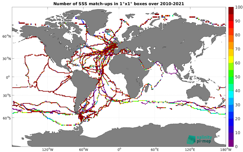
Figure 5: Number of SSS match-ups between TSG (GOSUD-Sailing-ship) SSS and the SMOS SSS L3 v9 - 9 Days (CATDS-CEC-LOCEAN) SSS product for the Global Ocean Pi-MEP region over 1^\circ \times 1^\circ boxes and for the full satellite product period.
