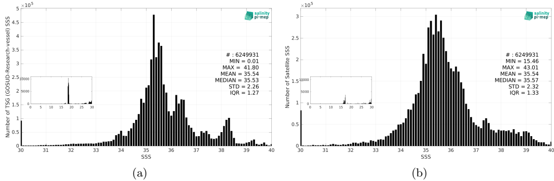
Figure 3: Histograms of SSS from TSG (GOSUD-Research-vessel) (a) and SMOS SSS L3 v9 - 9 Days (CATDS-CEC-LOCEAN) (b) considering all match-up pairs per bins of 0.1 over the Global Ocean Pi-MEP region and for the full satellite product period.
