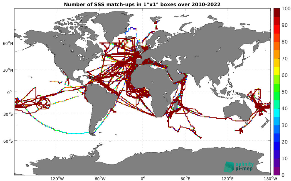
Figure 5: Number of SSS match-ups between TSG (GOSUD-Research-vessel) SSS and the SMOS SSS L3 v9 - 9 Days (CATDS-CEC-LOCEAN) SSS product for the Global Ocean Pi-MEP region over 1^\circ \times 1^\circ boxes and for the full satellite product period.
