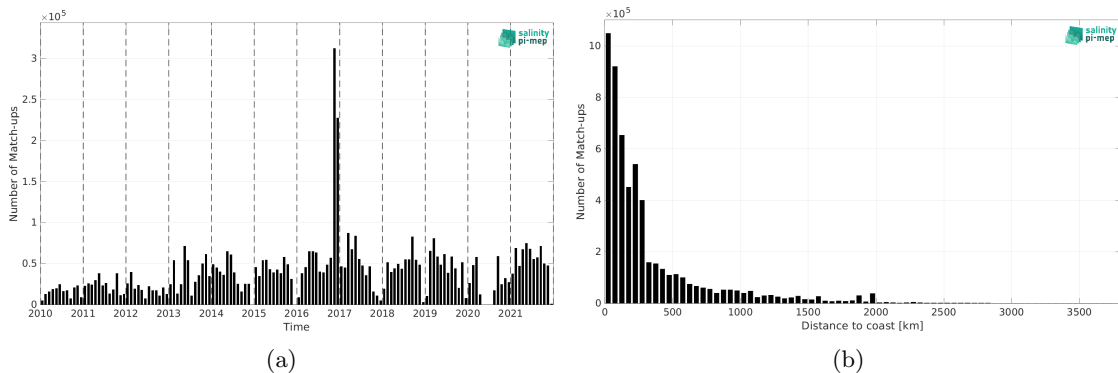
Figure 1: Number of match-ups between TSG (GOSUD-Research-vessel) and SMOS SSS L3 v9 - 9 Days (CATDS-CEC-LOCEAN) SSS as a function of time (a) and as function of the distance to coast (b) over the Global Ocean Pi-MEP region and for the full satellite product period.
