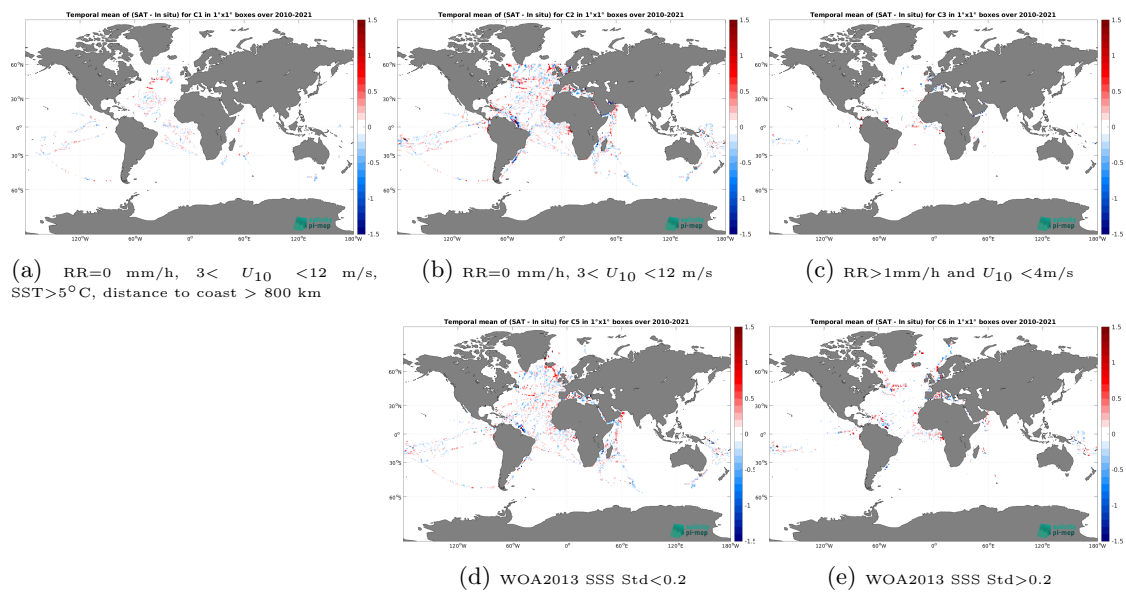
Figure 12: Temporal mean gridded over spatial boxes of size 1^\circ \times 1^\circ of \Delta\text{SSS} (SMOS SSS L3 v9 - 9 Days (CATDS-CEC-LOCEAN) - TSG (GOSUD-Research-vessel)) for 5 different subdatasets corresponding to: RR=0 mm/h, 3 < U_{10} < 12 m/s, SST > 5^\circ\text{C} , distance to coast > 800 km (a), RR=0 mm/h, 3 < U_{10} < 12 m/s (b), RR > 1 mm/h and U_{10} < 4 m/s (c), WOA2013 SSS Std < 0.2 (d), WOA2013 SSS Std > 0.2 (e).
