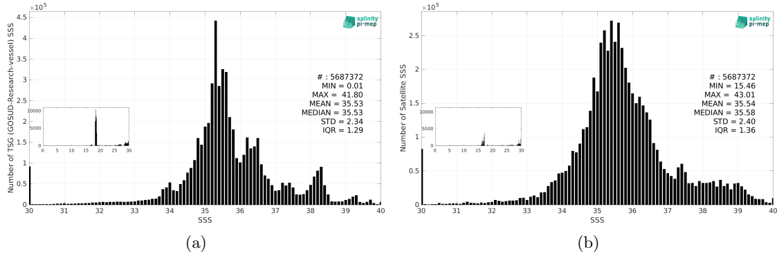
Figure 2: Histograms of SSS from TSG (GOSUD-Research-vessel) (a) and SMOS SSS L3 v9 - 9 Days (CATDS-CEC-LOCEAN) (b) considering all match-up pairs per bins of 0.1 over the Global Ocean Pi-MEP region and for the full satellite product period.
