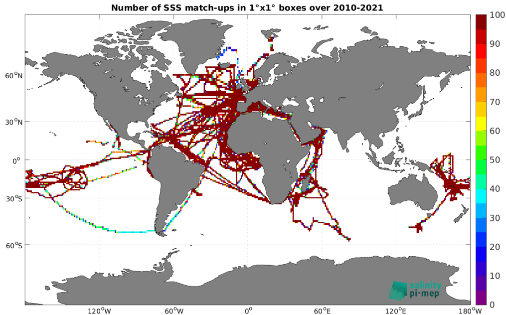
Figure 4: Number of SSS match-ups between TSG (GOSUD-Research-vessel) SSS and the SMOS SSS L3 v9 - 9 Days (CATDS-CEC-LOCEAN) SSS product for the Global Ocean Pi-MEP region over 1^\circ \times 1^\circ boxes and for the full satellite product period.
