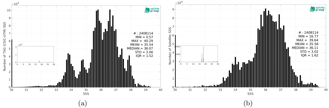
Figure 3: Histograms of SSS from TSG (CSIC-UTM) (a) and SMOS SSS L3 v9 - 9 Days (CATDS-CEC-LOCEAN) (b) considering all match-up pairs per bins of 0.1 over the Global Ocean Pi-MEP region and for the full satellite product period.
