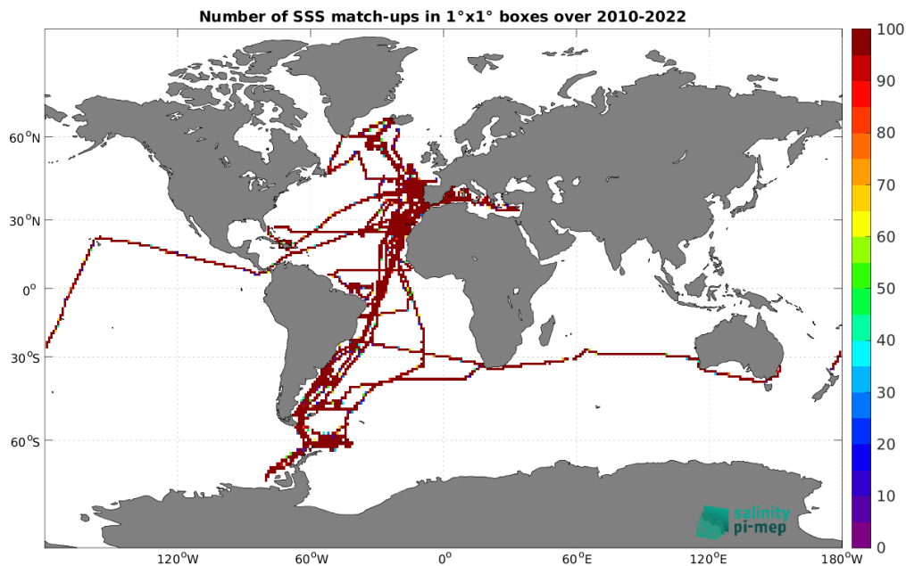
Figure 5: Number of SSS match-ups between TSG (CSIC-UTM) SSS and the SMOS SSS L3 v9 - 9 Days (CATDS-CEC-LOCEAN) SSS product for the Global Ocean Pi-MEP region over 1^\circ \times 1^\circ boxes and for the full satellite product period.
