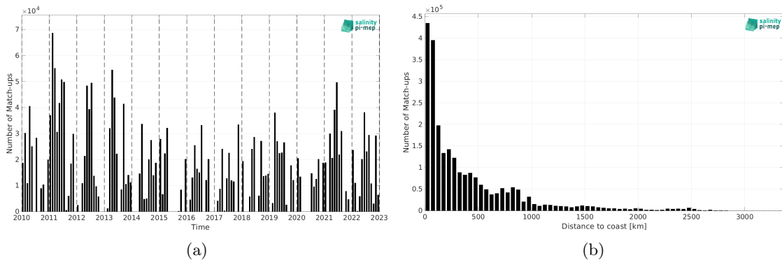
Figure 2: Number of match-ups between TSG (CSIC-UTM) and SMOS SSS L3 v9 - 9 Days (CATDS-CEC-LOCEAN) SSS as a function of time (a) and as function of the distance to coast (b) over the Global Ocean Pi-MEP region and for the full satellite product period.
