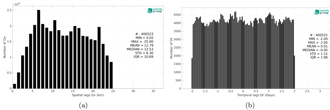
Figure 6: Histograms of the spatial (a) and temporal (b) lags between the location/time of the TSG (Amundsen) measurement and the date of the corresponding SMOS SSS L3 v9 - 9 Days (CATDS-CEC-LOCEAN) SSS pixel.
