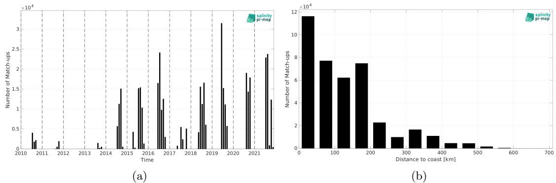
Figure 2: Number of match-ups between TSG (Amundsen) and SMOS SSS L3 v9 - 9 Days (CATDS-CEC-LOCEAN) SSS as a function of time (a) and as function of the distance to coast (b) over the Global Ocean Pi-MEP region and for the full satellite product period.
