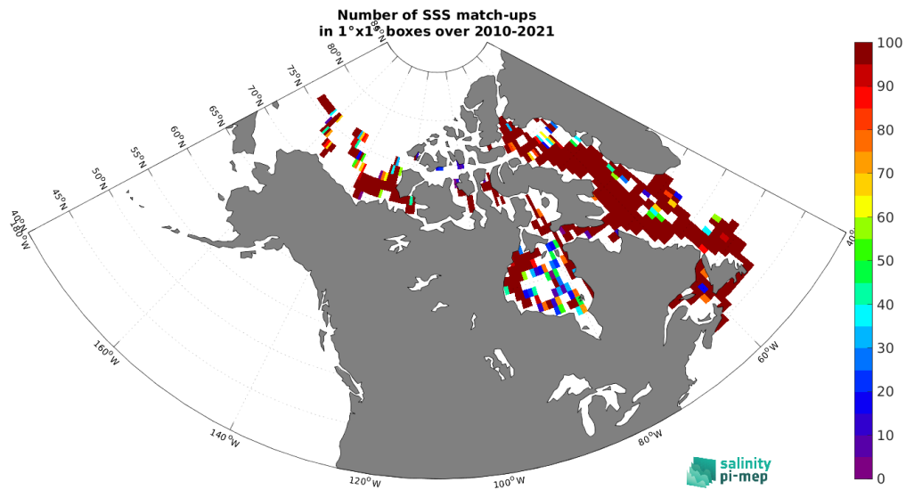
Figure 5: Number of SSS match-ups between TSG (Amundsen) SSS and the SMOS SSS L3 v9 - 9 Days (CATDS-CEC-LOCEAN) SSS product for the Global Ocean Pi-MEP region over 1^\circ \times 1^\circ boxes and for the full satellite product period.
