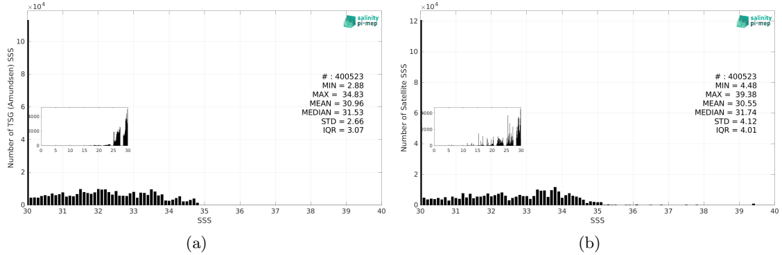
Figure 3: Histograms of SSS from TSG (Amundsen) (a) and SMOS SSS L3 v9 - 9 Days (CATDS-CEC-LOCEAN) (b) considering all match-up pairs per bins of 0.1 over the Global Ocean Pi-MEP region and for the full satellite product period.
