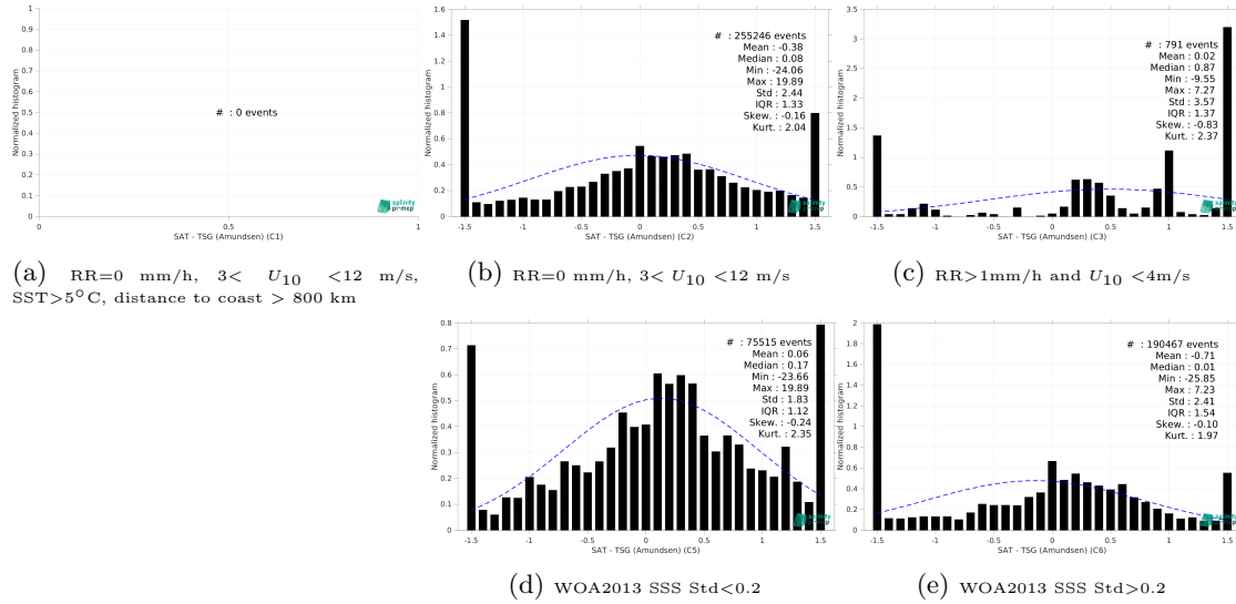
Figure 15: Normalized histogram of \Delta SSS (SMOS SSS L3 v9 - 9 Days (CATDS-CEC-LOCEAN) - TSG (Amundsen)) for 5 different subdatasets corresponding to: RR=0 mm/h, 3 < U_{10} < 12 m/s, SST > 5°C, distance to coast > 800 km (a), RR=0 mm/h, 3 < U_{10} < 12 m/s (b), RR > 1mm/h and U_{10} < 4 m/s (c), WOA2013 SSS Std < 0.2 (d), WOA2013 SSS Std > 0.2 (e).
