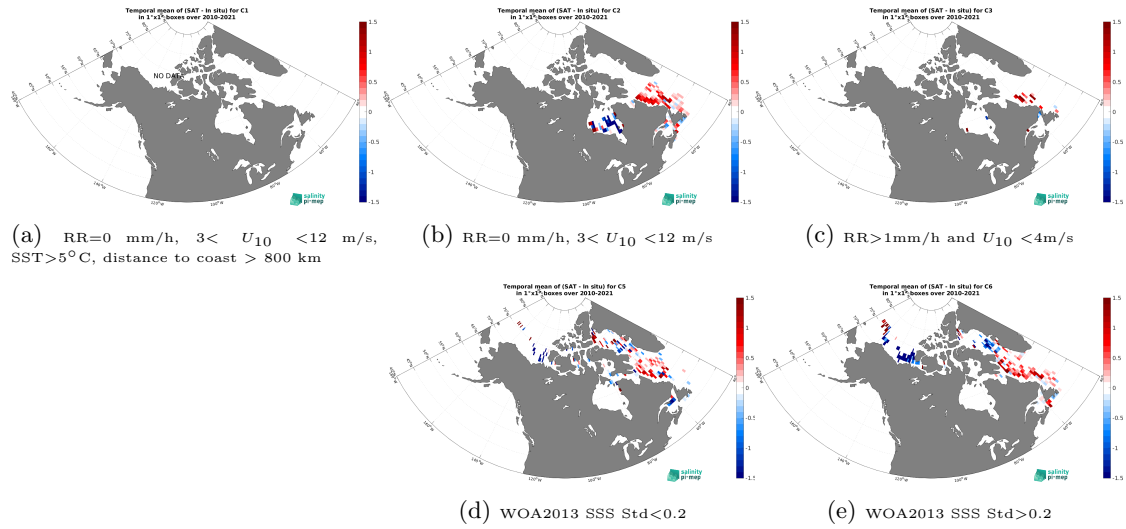
Figure 12: Temporal mean gridded over spatial boxes of size 1^{\circ}\times 1^{\circ} of \Delta\text{SSS} (SMOS SSS L3 v9 - 9 Days (CATDS-CEC-LOCEAN) - TSG (Amundsen)) for 5 different subdatasets corresponding to:RR=0 mm/h, 3 < U_{10} < 12 m/s, SST > 5^{\circ}\text{C} , distance to coast > 800 km (a), RR=0 mm/h, 3 < U_{10} < 12 m/s (b), RR > 1 mm/h and U_{10} < 4 m/s (c), WOA2013 SSS Std < 0.2 (d), WOA2013 SSS Std > 0.2 (e).
