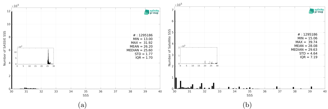
Figure 3: Histograms of SSS from SASSIE (a) and SMOS SSS L3 v9 - 9 Days (CATDS-CEC-LOCEAN) (b) considering all match-up pairs per bins of 0.1 over the Global Ocean Pi-MEP region and for the full satellite product period.
