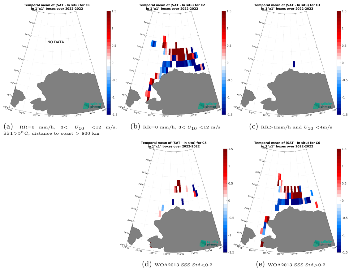
Figure 14: Temporal mean gridded over spatial boxes of size 1^\circ \times 1^\circ of \Delta SSS (SMOS SSS L3 v9 - 9 Days (CATDS-CEC-LOCEAN) - SASSIE) for 5 different subdatasets corresponding to:RR=0 mm/h, 3 < U_{10} < 12 m/s, SST >5^\circ\text{C} , distance to coast > 800 km (a), RR=0 mm/h, 3 < U_{10} < 12 m/s (b), RR >1 mm/h and U_{10} < 4 m/s (c), WOA2013 SSS Std <0.2 (d), WOA2013 SSS Std >0.2 (e).
