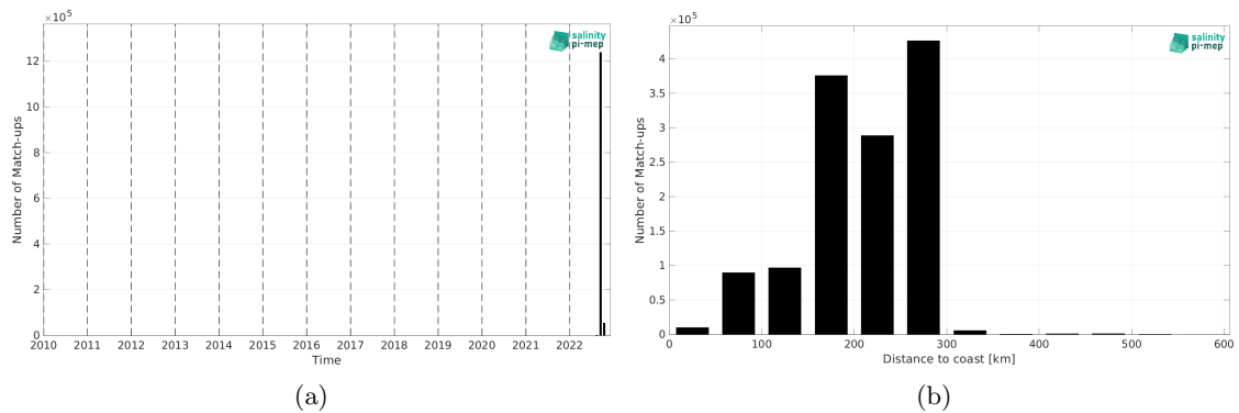
Figure 2: Number of match-ups between SASSIE and SMOS SSS L3 v9 - 9 Days (CATDS-CEC-LOCEAN) SSS as a function of time (a) and as function of the distance to coast (b) over the Global Ocean Pi-MEP region and for the full satellite product period.
