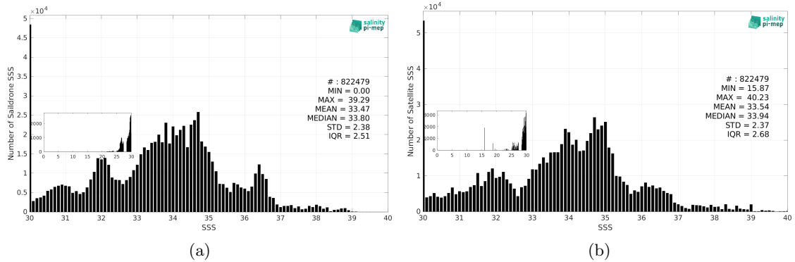
Figure 3: Histograms of SSS from Saildrone (a) and SMOS SSS L3 v9 - 9 Days (CATDS-CEC-LOCEAN) (b) considering all match-up pairs per bins of 0.1 over the Global Ocean Pi-MEP region and for the full satellite product period.
