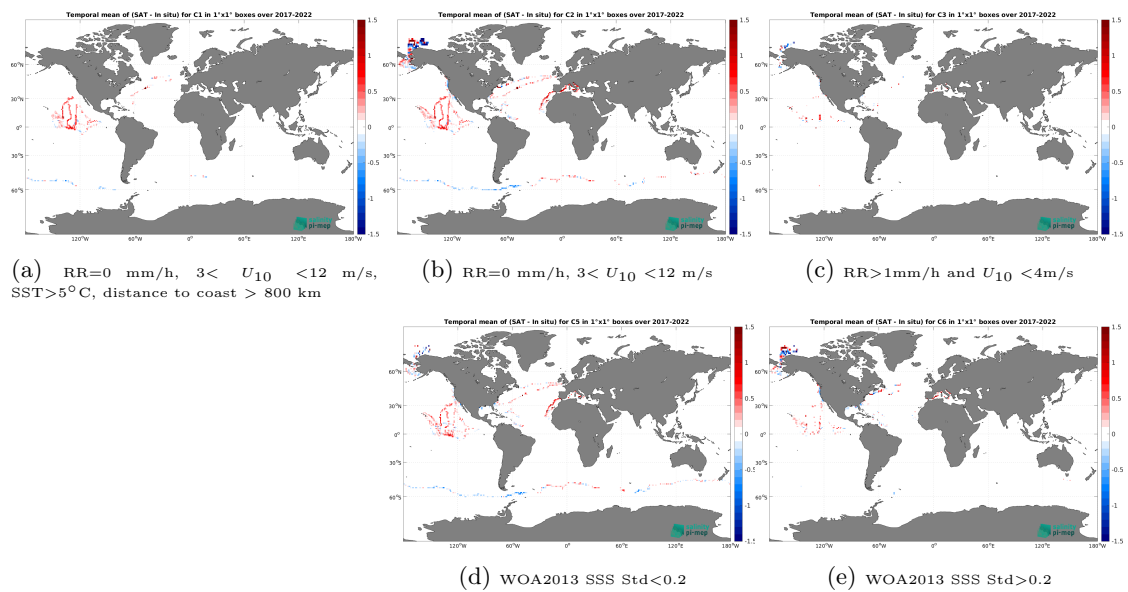
Figure 14: Temporal mean gridded over spatial boxes of size 1^\circ \times 1^\circ of \Delta SSS (SMOS SSS L3 v9 - 9 Days (CATDS-CEC-LOCEAN) - Saildrone) for 5 different subdatasets corresponding to:RR=0 mm/h, 3 < U_{10} < 12 m/s, SST > 5^\circ\text{C} , distance to coast > 800 km (a), RR=0 mm/h, 3 < U_{10} < 12 m/s (b), RR > 1 mm/h and U_{10} < 4 m/s (c), WOA2013 SSS Std < 0.2 (d), WOA2013 SSS Std > 0.2 (e).
