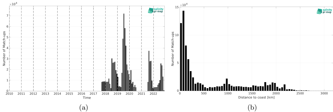
Figure 2: Number of match-ups between Saildrone and SMOS SSS L3 v9 - 9 Days (CATDS-CEC-LOCEAN) SSS as a function of time (a) and as function of the distance to coast (b) over the Global Ocean Pi-MEP region and for the full satellite product period.
