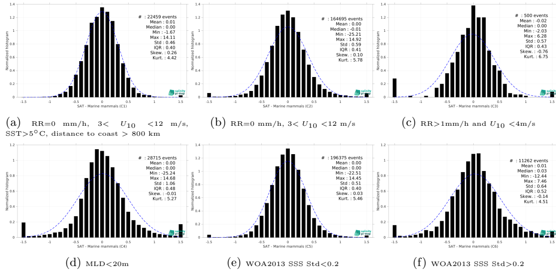
Figure 15: Normalized histogram of \Delta\text{SSS} (SMOS SSS L3 v9 - 9 Days (CATDS-CEC-LOCEAN) - Marine mammals) for 6 different subdatasets corresponding to: RR=0 mm/h, 3 < U_{10} < 12 m/s, SST>5°C, distance to coast > 800 km (a), RR=0 mm/h, 3 < U_{10} < 12 m/s (b), RR>1mm/h and U_{10} < 4 m/s (c), MLD<20m (d), WOA2013 SSS Std<0.2 (e), WOA2013 SSS Std>0.2 (f).
