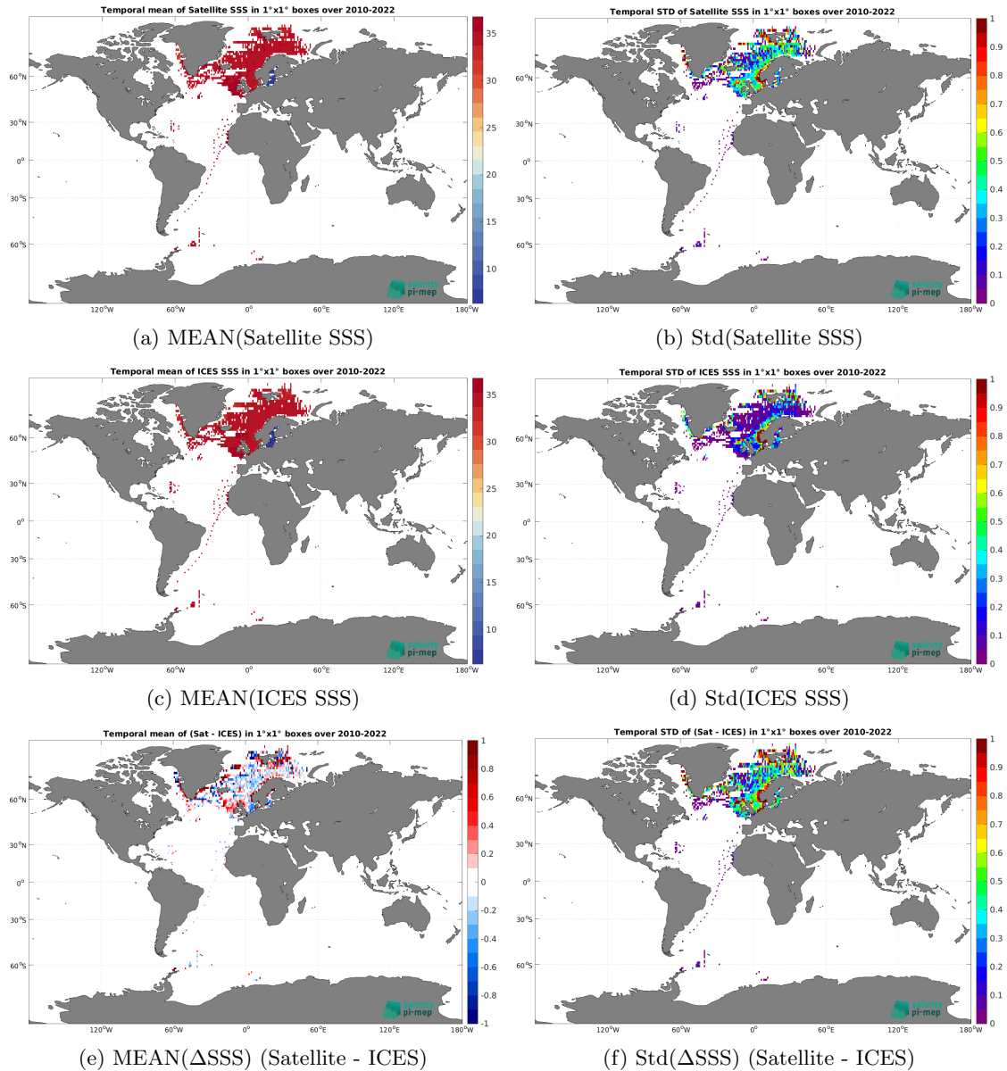
Figure 7: Temporal mean (left) and Std (right) of SSS from SMOS SSS L3 v9 - 9 Days (CATDS-CEC-LOCEAN) (top), ICES (middle), and of \Delta SSS (Satellite - ICES). Only match-up pairs are used to generate these maps.
