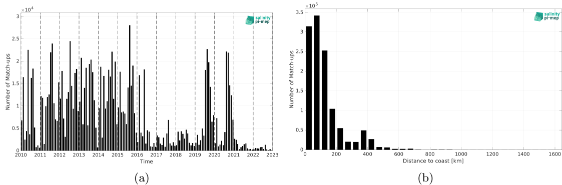
Figure 2: Number of match-ups between ICES and SMOS SSS L3 v9 - 9 Days (CATDS-CEC-LOCEAN) SSS as a function of time (a) and as function of the distance to coast (b) over the Global Ocean Pi-MEP region and for the full satellite product period.
