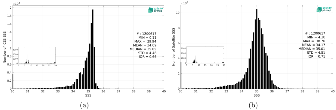
Figure 3: Histograms of SSS from ICES (a) and SMOS SSS L3 v9 - 9 Days (CATDS-CEC-LOCEAN) (b) considering all match-up pairs per bins of 0.1 over the Global Ocean Pi-MEP region and for the full satellite product period.
