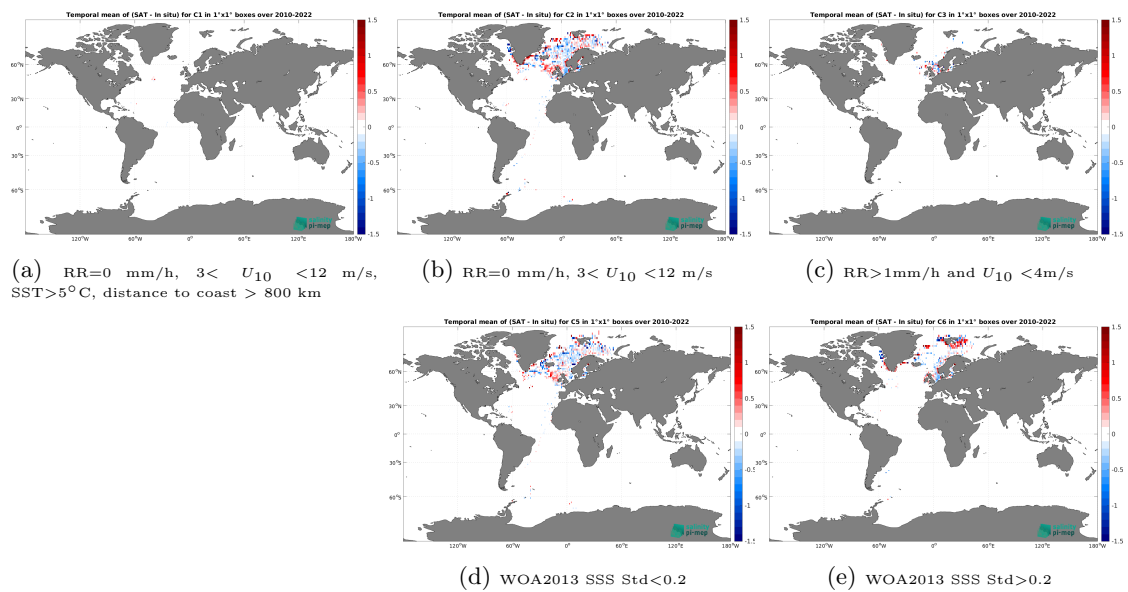
Figure 14: Temporal mean gridded over spatial boxes of size 1^\circ \times 1^\circ of \Delta SSS (SMOS SSS L3 v9 - 9 Days (CATDS-CEC-LOCEAN) - ICES) for 5 different subdatasets corresponding to:RR=0 mm/h, 3 < U_{10} < 12 m/s, SST > 5^\circ\text{C} , distance to coast > 800 km (a), RR=0 mm/h, 3 < U_{10} < 12 m/s (b), RR > 1 mm/h and U_{10} < 4 m/s (c), WOA2013 SSS Std < 0.2 (d), WOA2013 SSS Std > 0.2 (e).
