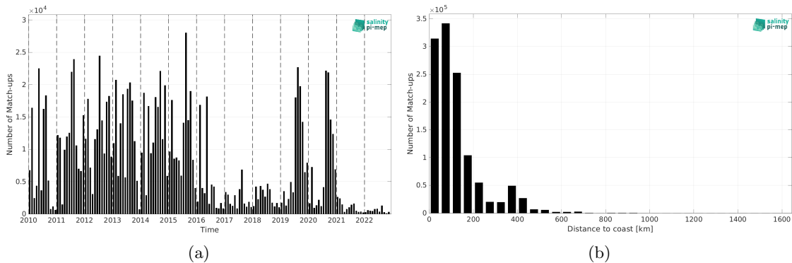
Figure 1: Number of match-ups between ICES and SMOS SSS L3 v9 - 9 Days (CATDS-CEC-LOCEAN) SSS as a function of time (a) and as function of the distance to coast (b) over the Global Ocean Pi-MEP region and for the full satellite product period.
