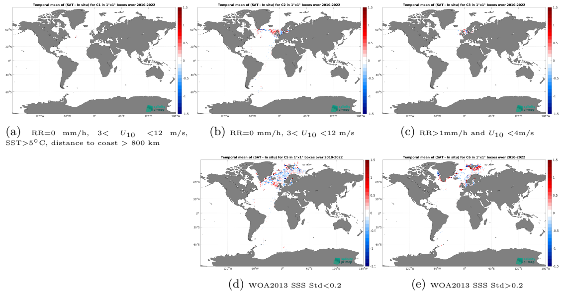
Figure 12: Temporal mean gridded over spatial boxes of size 1^\circ \times 1^\circ of \Delta SSS (SMOS SSS L3 v9 - 9 Days (CATDS-CEC-LOCEAN) - ICES) for 5 different subdatasets corresponding to:RR=0 mm/h, 3 < U_{10} < 12 m/s, SST > 5^\circ\text{C} , distance to coast > 800 km (a), RR=0 mm/h, 3 < U_{10} < 12 m/s (b), RR > 1 mm/h and U_{10} < 4 m/s (c), WOA2013 SSS Std < 0.2 (d), WOA2013 SSS Std > 0.2 (e).
