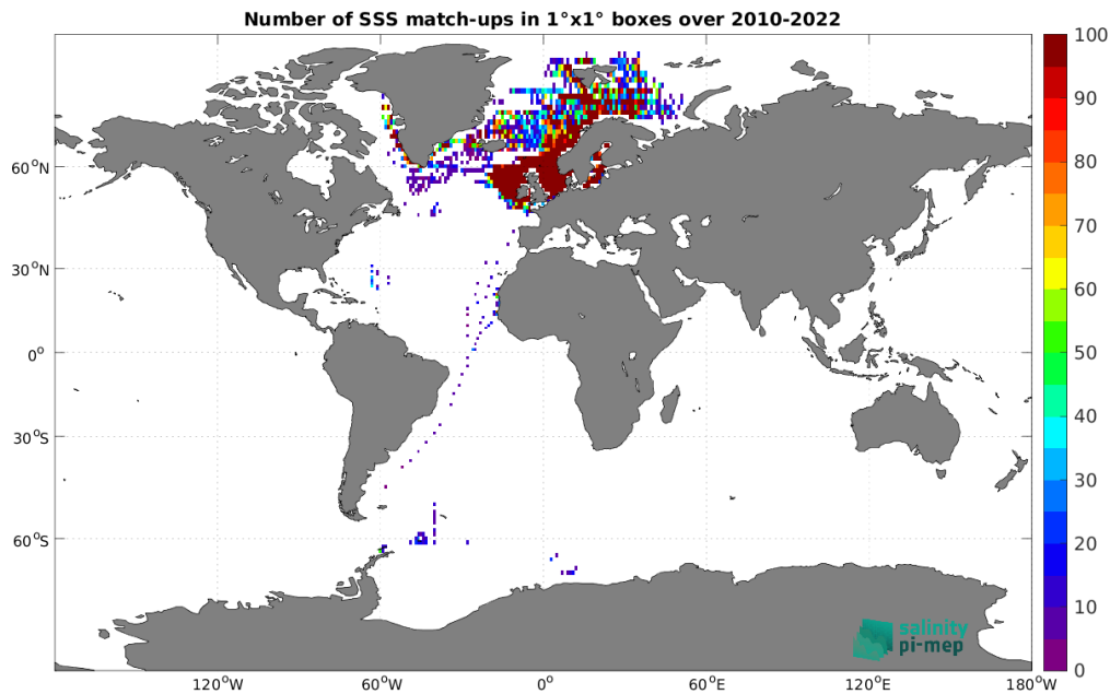
Figure 4: Number of SSS match-ups between ICES SSS and the SMOS SSS L3 v9 - 9 Days (CATDS-CEC-LOCEAN) SSS product for the Global Ocean Pi-MEP region over 1^\circ \times 1^\circ boxes and for the full satellite product period.
