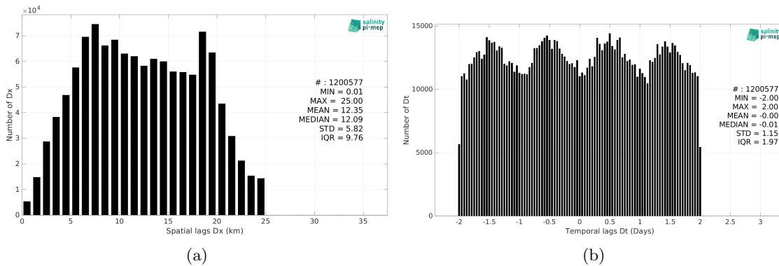
Figure 5: Histograms of the spatial (a) and temporal (b) lags between the location/time of the ICES measurement and the date of the corresponding SMOS SSS L3 v9 - 9 Days (CATDS-CEC-LOCEAN) SSS pixel.
