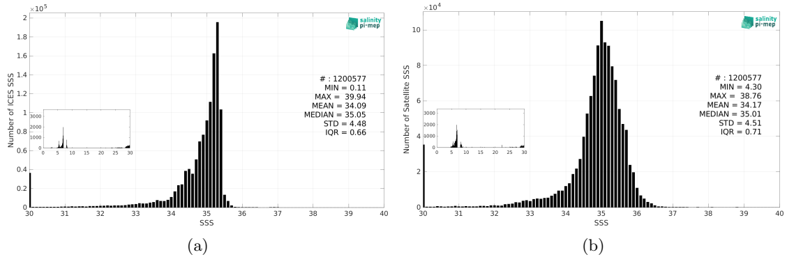
Figure 2: Histograms of SSS from ICES (a) and SMOS SSS L3 v9 - 9 Days (CATDS-CEC-LOCEAN) (b) considering all match-up pairs per bins of 0.1 over the Global Ocean Pi-MEP region and for the full satellite product period.
