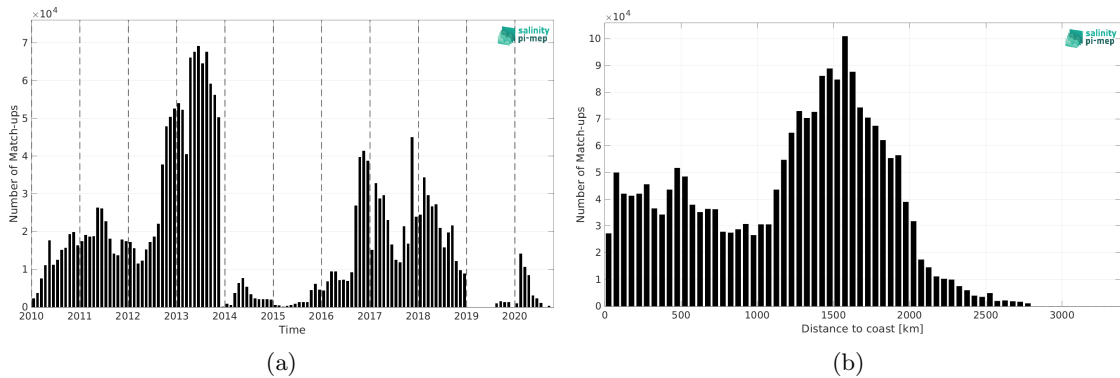
Figure 1: Number of match-ups between Surface drifters and SMOS SSS L3 v9 - 9 Days (CATDS-CEC-LOCEAN) SSS as a function of time (a) and as function of the distance to coast (b) over the Global Ocean Pi-MEP region and for the full satellite product period.
