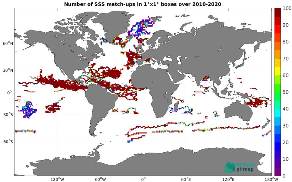
Figure 3: Number of SSS match-ups between Surface drifters SSS and the SMOS SSS L3 v9 - 9 Days (CATDS-CEC-LOCEAN) SSS product for the Global Ocean Pi-MEP region over 1^\circ \times 1^\circ boxes and for the full satellite product period.
