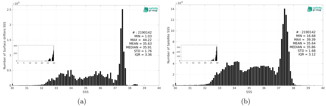
Figure 2: Histograms of SSS from Surface drifters (a) and SMOS SSS L3 v9 - 9 Days (CATDS-CEC-LOCEAN) (b) considering all match-up pairs per bins of 0.1 over the Global Ocean Pi-MEP region and for the full satellite product period.
