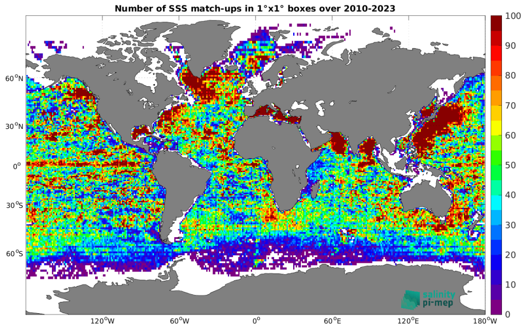
Figure 4: Number of SSS match-ups between Argo SSS and the SMOS SSS L3 v9 - 9 Days (CATDS-CEC-LOCEAN) SSS product for the Global Ocean Pi-MEP region over 1^\circ \times 1^\circ boxes and for the full satellite product period.
