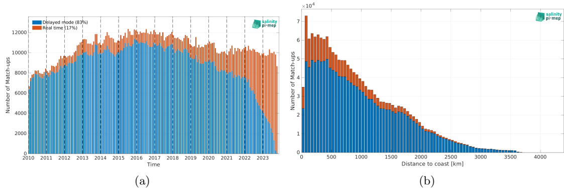
Figure 1: Number of match-ups between Argo and SMOS SSS L3 v9 - 9 Days (CATDS-CEC-LOCEAN) SSS as a function of time (a) and as function of the distance to coast (b) over the Global Ocean Pi-MEP region and for the full satellite product period.
