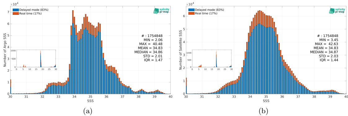
Figure 2: Histograms of SSS from Argo (a) and SMOS SSS L3 v9 - 9 Days (CATDS-CEC-LOCEAN) (b) considering all match-up pairs per bins of 0.1 over the Global Ocean Pi-MEP region and for the full satellite product period.
