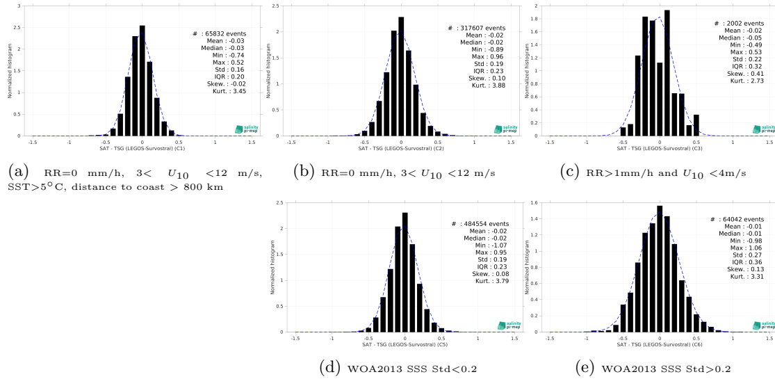
Figure 13: Normalized histogram of \Delta SSS (SMOS SSS L3 v9 - 18 Days (CATDS-CEC-LOCEAN) - TSG (LEGOS-Survostral)) for 5 different subdatasets corresponding to: RR=0 mm/h, 3 < U_{10} < 12 m/s, SST > 5°C, distance to coast > 800 km (a), RR=0 mm/h, 3 < U_{10} < 12 m/s (b), RR > 1mm/h and U_{10} < 4 m/s (c), WOA2013 SSS Std < 0.2 (d), WOA2013 SSS Std > 0.2 (e).
