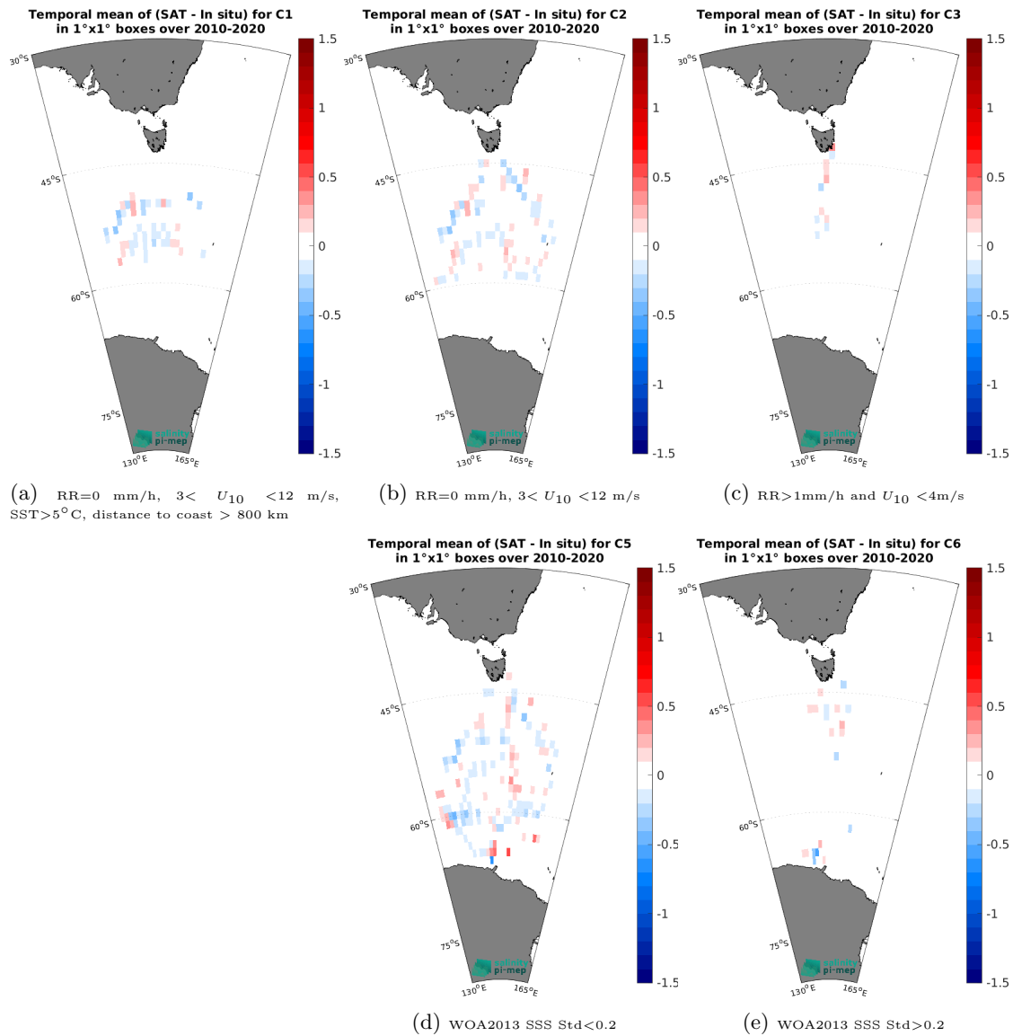
Figure 12: Temporal mean gridded over spatial boxes of size 1^\circ \times 1^\circ of \Delta\text{SSS} (SMOS SSS L3 v9 - 18 Days (CATDS-CEC-LOCEAN) - TSG (LEGOS-Survostral)) for 5 different subdatasets corresponding to: RR=0 mm/h, 3 < U_{10} < 12 m/s, SST > 5^\circ\text{C} , distance to coast > 800 km (a), RR=0 mm/h, 3 < U_{10} < 12 m/s (b), RR > 1 mm/h and U_{10} < 4 m/s (c), WOA2013 SSS Std < 0.2 (d), WOA2013 SSS Std > 0.2 (e).
