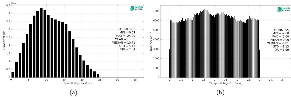
Figure 5: Histograms of the spatial (a) and temporal (b) lags between the location/time of the TSG (LEGOS-Survostral) measurement and the date of the corresponding SMOS SSS L3 v9 - 18 Days (CATDS-CEC-LOCEAN) SSS pixel.
