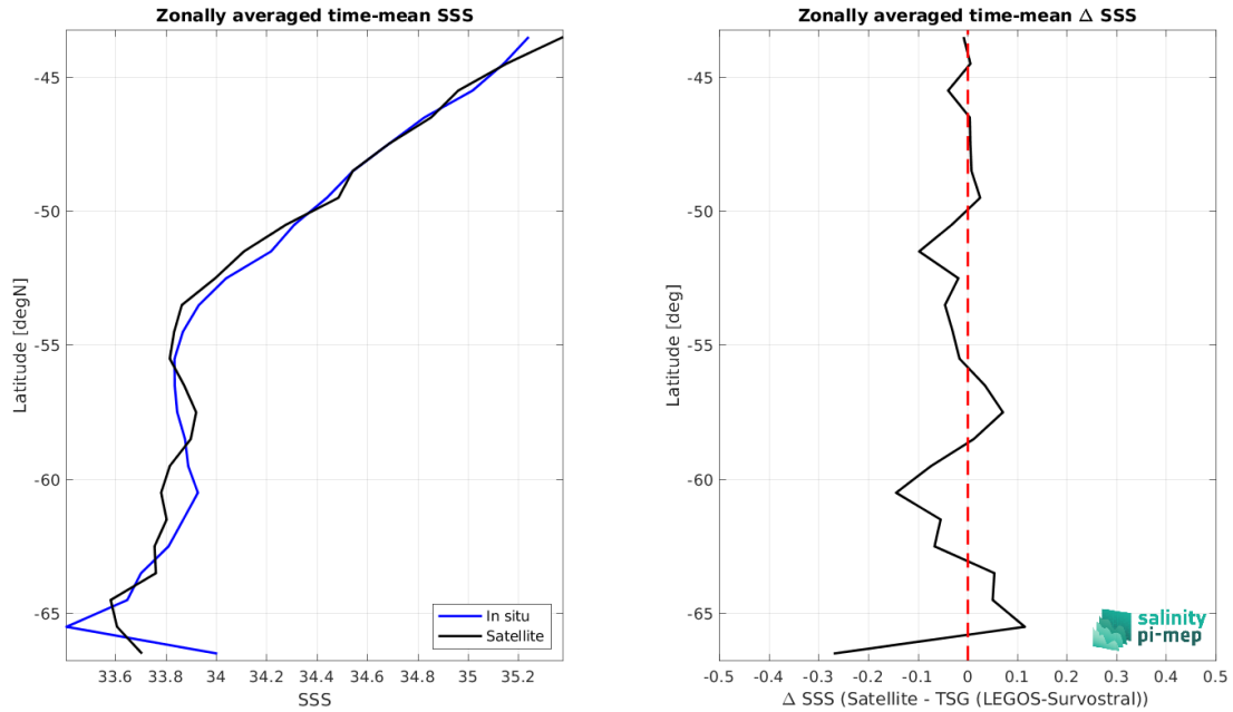
Figure 8: Left panel: Zonal mean SSS from SMOS SSS L3 v9 - 18 Days (CATDS-CEC-LOCEAN) satellite product (black) and from TSG (LEGOS-Survostral) (blue). Right panel: Zonal mean of \Delta SSS (Satellite - TSG (LEGOS-Survostral)) for all the collected Pi-MEP match-up pairs estimated over the full satellite product period.
