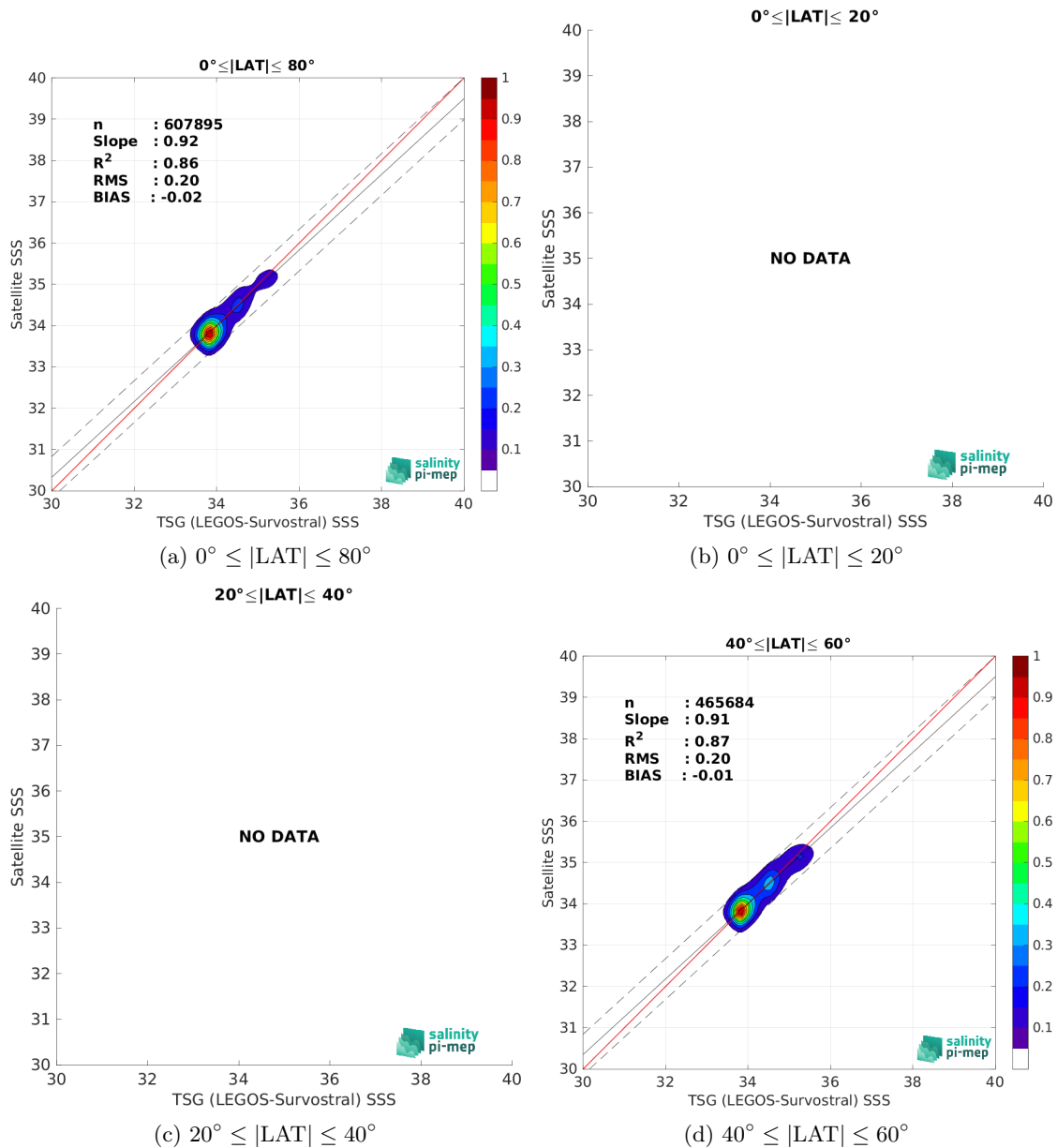
Figure 9: Contour maps of the concentration of SMOS SSS L3 v9 - 18 Days (CATDS-CEC-LOCEAN) SSS (y-axis) versus TSG (LEGOS-Survostral) SSS (x-axis) at match-up pairs for different latitude bands. For each plot, the red line shows x=y . The black thin and dashed lines indicate a linear fit through the data cloud and the \pm 95\% confidence levels, respectively. The number match-up pairs n , the slope and R^2 coefficient of the linear fit, the root mean square (RMS) and the mean bias between satellite and in situ data are indicated for each latitude band in each plots.
