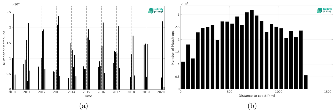
Figure 1: Number of match-ups between TSG (LEGOS-Survostral) and SMOS SSS L3 v9 - 18 Days (CATDS-CEC-LOCEAN) SSS as a function of time (a) and as function of the distance to coast (b) over the Global Ocean Pi-MEP region and for the full satellite product period.
