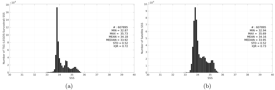
Figure 2: Histograms of SSS from TSG (LEGOS-Survostral) (a) and SMOS SSS L3 v9 - 18 Days (CATDS-CEC-LOCEAN) (b) considering all match-up pairs per bins of 0.1 over the Global Ocean Pi-MEP region and for the full satellite product period.
