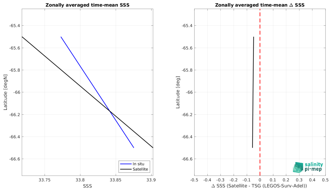
Figure 9: Left panel: Zonal mean SSS from SMOS SSS L3 v9 - 18 Days (CATDS-CEC-LOCEAN) satellite product (black) and from TSG (LEGOS-Surv-Adel) (blue). Right panel: Zonal mean of \Delta SSS (Satellite - TSG (LEGOS-Surv-Adel)) for all the collected Pi-MEP match-up pairs estimated over the full satellite product period.
