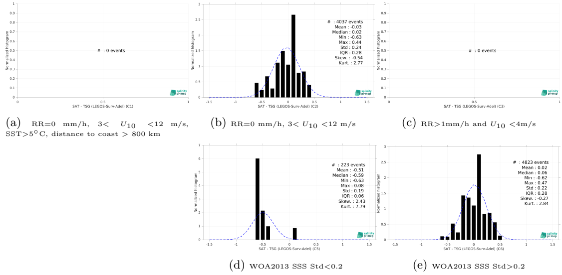
Figure 15: Normalized histogram of \Delta SSS (SMOS SSS L3 v9 - 18 Days (CATDS-CEC-LOCEAN) - TSG (LEGOS-Surv-Adel)) for 5 different subdatasets corresponding to: RR=0 mm/h, 3 < U_{10} < 12 m/s, SST > 5°C, distance to coast > 800 km (a), RR=0 mm/h, 3 < U_{10} < 12 m/s (b), RR > 1mm/h and U_{10} < 4 m/s (c), WOA2013 SSS Std < 0.2 (d), WOA2013 SSS Std > 0.2 (e).
