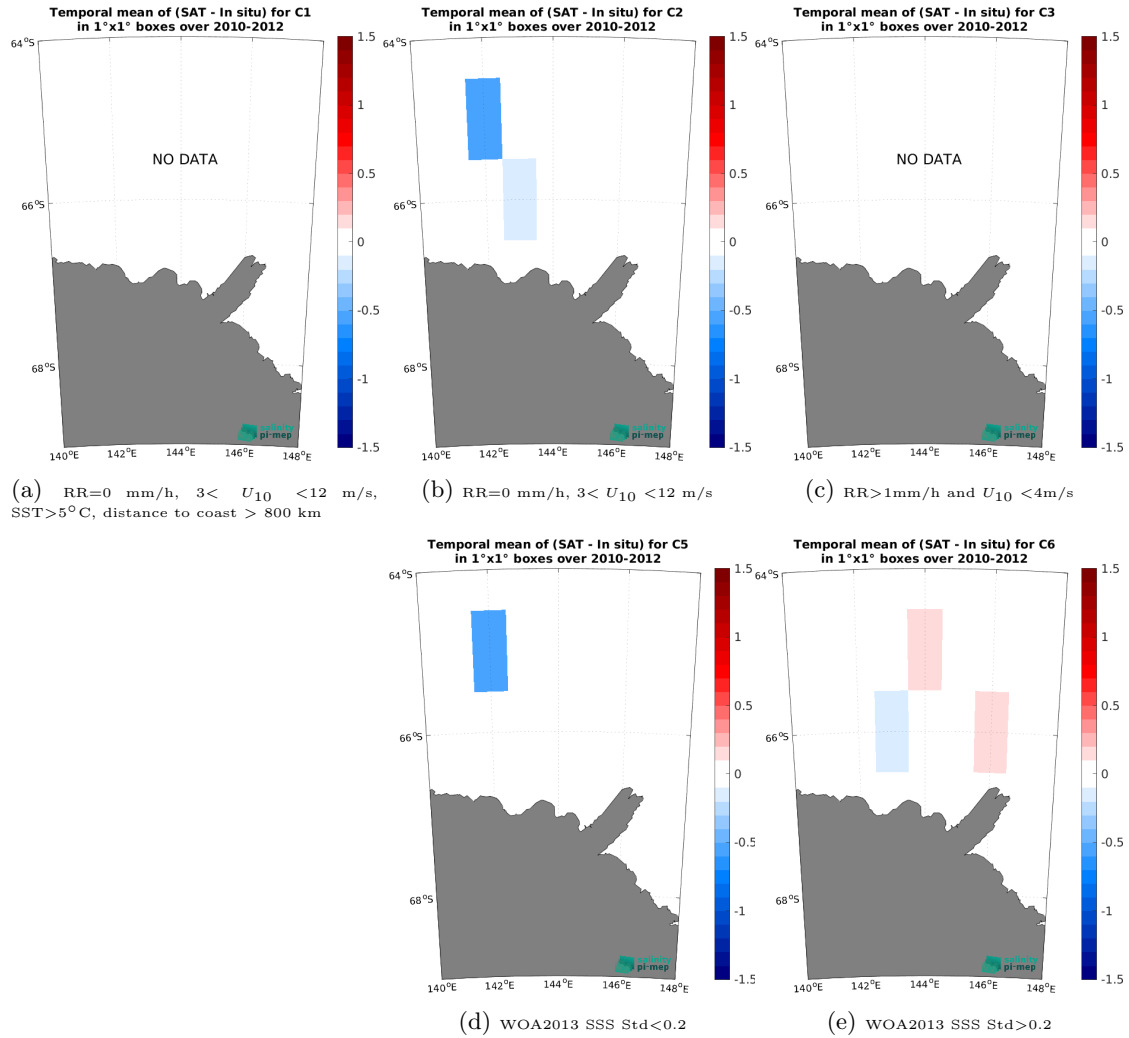
Figure 14: Temporal mean gridded over spatial boxes of size 1^{\circ}\times 1^{\circ} of \Delta SSS (SMOS SSS L3 v9 - 18 Days (CATDS-CEC-LOCEAN) - TSG (LEGOS-Surv-Adel)) for 5 different subdatasets corresponding to:RR=0 mm/h, 3 < U_{10} < 12 m/s, SST>5°C, distance to coast > 800 km (a), RR=0 mm/h, 3 < U_{10} < 12 m/s (b), RR>1mm/h and U_{10} < 4 m/s (c), WOA2013 SSS Std<0.2 (d), WOA2013 SSS Std>0.2 (e).
