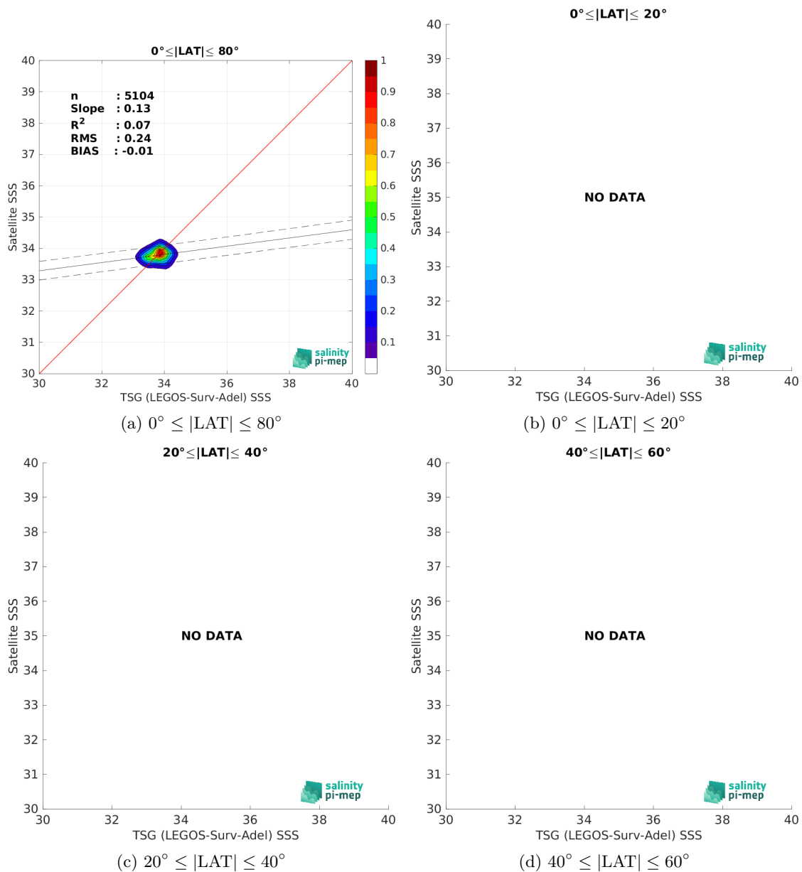
Figure 10: Contour maps of the concentration of SMOS SSS L3 v9 - 18 Days (CATDS-CEC-LOCEAN) SSS (y-axis) versus TSG (LEGOS-Surv-Adel) SSS (x-axis) at match-up pairs for different latitude bands. For each plot, the red line shows x=y . The black thin and dashed lines indicate a linear fit through the data cloud and the \pm 95\% confidence levels, respectively. The number match-up pairs n , the slope and R^2 coefficient of the linear fit, the root mean square (RMS) and the mean bias between satellite and in situ data are indicated for each latitude band in each plots.
