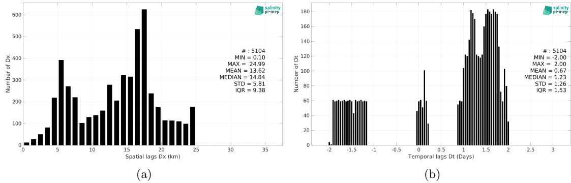
Figure 6: Histograms of the spatial (a) and temporal (b) lags between the location/time of the TSG (LEGOS-Surv-Adel) measurement and the date of the corresponding SMOS SSS L3 v9 - 18 Days (CATDS-CEC-LOCEAN) SSS pixel.
