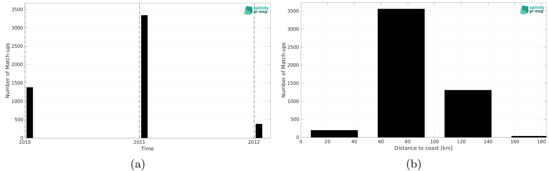
Figure 1: Number of match-ups between TSG (LEGOS-Surv-Adel) and SMOS SSS L3 v9 - 18 Days (CATDS-CEC-LOCEAN) SSS as a function of time (a) and as function of the distance to coast (b) over the Global Ocean Pi-MEP region and for the full satellite product period.
