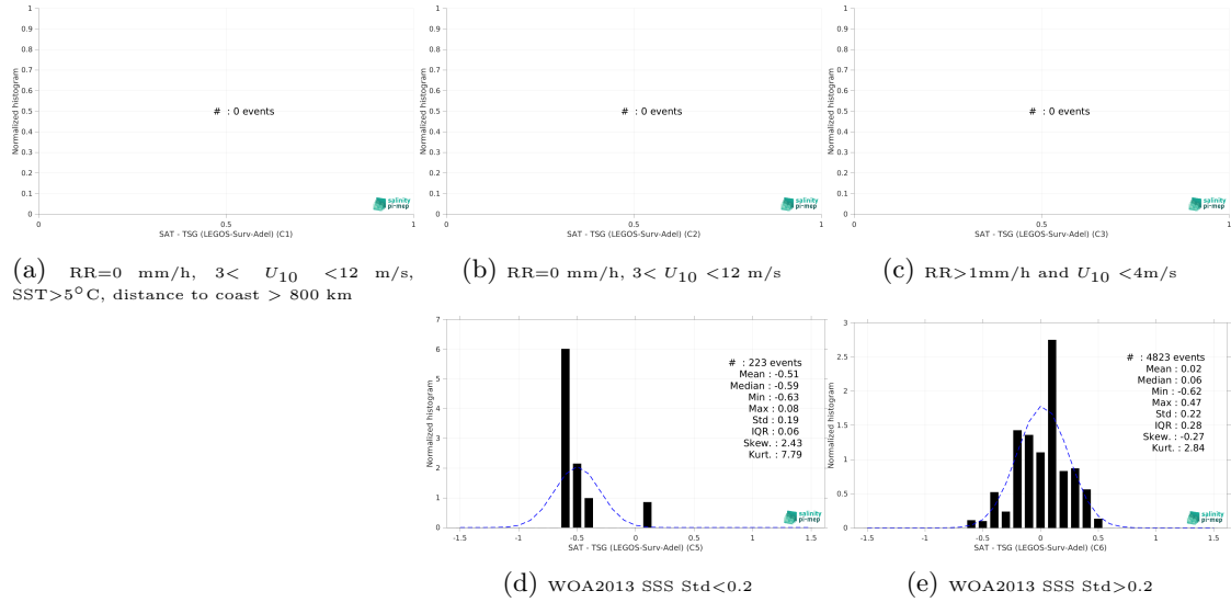
Figure 13: Normalized histogram of \Delta SSS (SMOS SSS L3 v9 - 18 Days (CATDS-CEC-LOCEAN) - TSG (LEGOS-Surv-Adel)) for 5 different subdatasets corresponding to: RR=0 mm/h, 3 < U_{10} < 12 m/s, SST>5°C, distance to coast > 800 km (a), RR=0 mm/h, 3 < U_{10} < 12 m/s (b), RR>1mm/h and U_{10} < 4 m/s (c), WOA2013 SSS Std<0.2 (d), WOA2013 SSS Std>0.2 (e).
