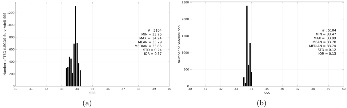
Figure 2: Histograms of SSS from TSG (LEGOS-Surv-Adel) (a) and SMOS SSS L3 v9 - 18 Days (CATDS-CEC-LOCEAN) (b) considering all match-up pairs per bins of 0.1 over the Global Ocean Pi-MEP region and for the full satellite product period.
