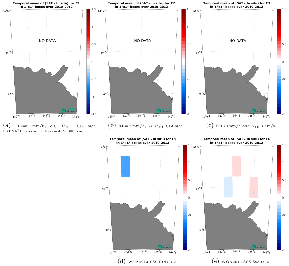
Figure 12: Temporal mean gridded over spatial boxes of size 1^\circ \times 1^\circ of \Delta SSS (SMOS SSS L3 v9 - 18 Days (CATDS-CEC-LOCEAN) - TSG (LEGOS-Surv-Adel)) for 5 different subdatasets corresponding to: RR=0 mm/h, 3 < U_{10} < 12 m/s, SST > 5°C, distance to coast > 800 km (a), RR=0 mm/h, 3 < U_{10} < 12 m/s (b), RR > 1mm/h and U_{10} < 4 m/s (c), WOA2013 SSS Std < 0.2 (d), WOA2013 SSS Std > 0.2 (e).
