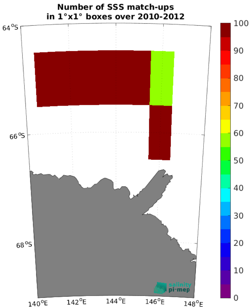
Figure 4: Number of SSS match-ups between TSG (LEGOS-Surv-Adel) SSS and the SMOS SSS L3 v9 - 18 Days (CATDS-CEC-LOCEAN) SSS product for the Global Ocean Pi-MEP region over 1°x1° boxes and for the full satellite product period.
