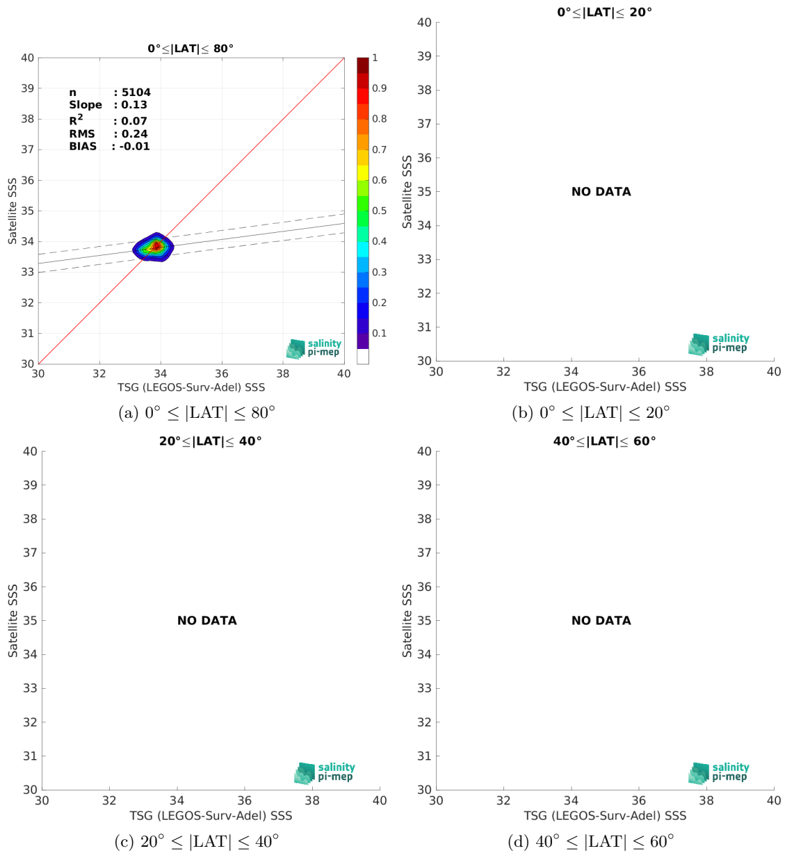
Figure 9: Contour maps of the concentration of SMOS SSS L3 v9 - 18 Days (CATDS-CEC-LOCEAN) SSS (y-axis) versus TSG (LEGOS-Surv-Adel) SSS (x-axis) at match-up pairs for different latitude bands. For each plot, the red line shows x=y . The black thin and dashed lines indicate a linear fit through the data cloud and the \pm 95\% confidence levels, respectively. The number match-up pairs n , the slope and R^2 coefficient of the linear fit, the root mean square (RMS) and the mean bias between satellite and in situ data are indicated for each latitude band in each plots.
