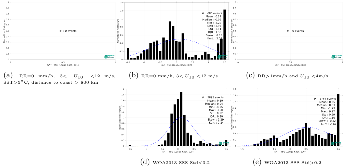
Figure 13: Normalized histogram of \Delta SSS (SMOS SSS L3 v9 - 18 Days (CATDS-CEC-LOCEAN) - TSG (Lauge-Koch)) for 5 different subdatasets corresponding to: RR=0 mm/h, 3 < U_{10} < 12 m/s, SST>5°C, distance to coast > 800 km (a), RR=0 mm/h, 3 < U_{10} < 12 m/s (b), RR>1mm/h and U_{10} < 4 m/s (c), WOA2013 SSS Std<0.2 (d), WOA2013 SSS Std>0.2 (e).
