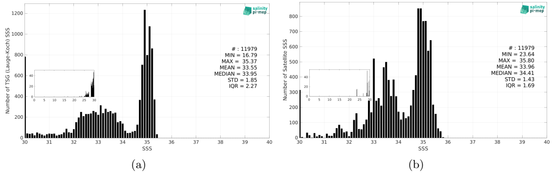
Figure 2: Histograms of SSS from TSG (Lauge-Koch) (a) and SMOS SSS L3 v9 - 18 Days (CATDS-CEC-LOCEAN) (b) considering all match-up pairs per bins of 0.1 over the Global Ocean Pi-MEP region and for the full satellite product period.
