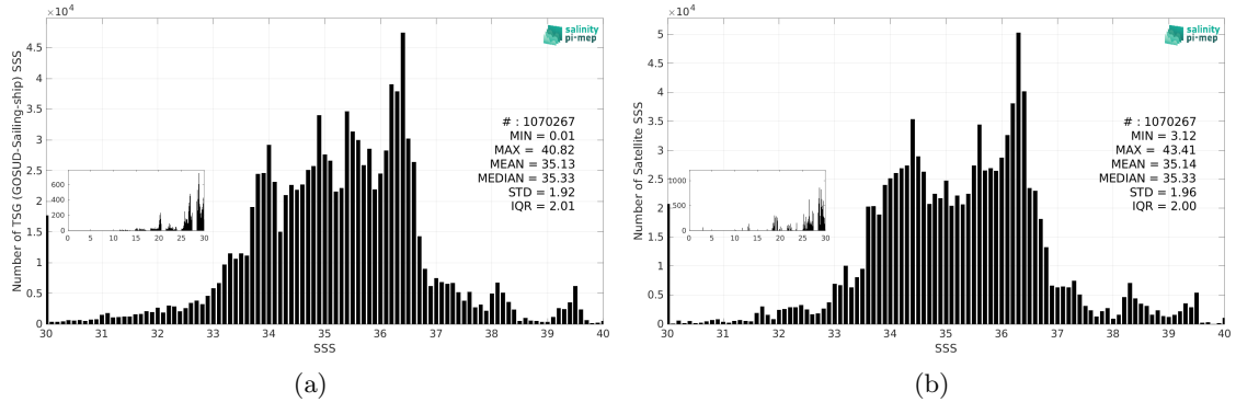
Figure 3: Histograms of SSS from TSG (GOSUD-Sailing-ship) (a) and SMOS SSS L3 v9 - 18 Days (CATDS-CEC-LOCEAN) (b) considering all match-up pairs per bins of 0.1 over the Global Ocean Pi-MEP region and for the full satellite product period.
