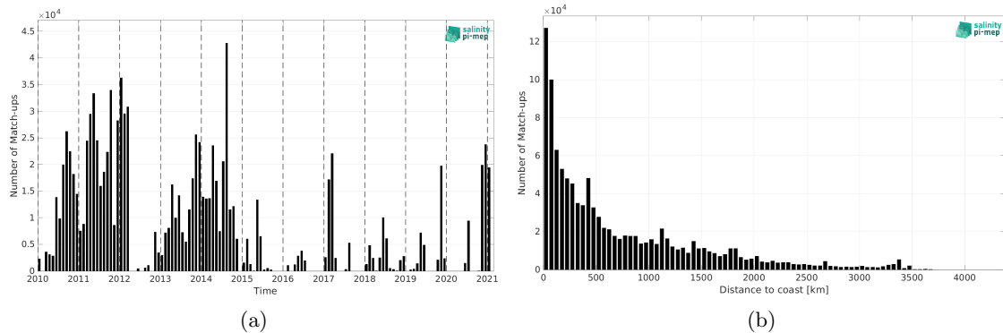
Figure 2: Number of match-ups between TSG (GOSUD-Sailing-ship) and SMOS SSS L3 v9 - 18 Days (CATDS-CEC-LOCEAN) SSS as a function of time (a) and as function of the distance to coast (b) over the Global Ocean Pi-MEP region and for the full satellite product period.
