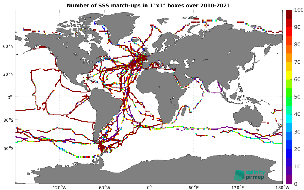
Figure 5: Number of SSS match-ups between TSG (GOSUD-Sailing-ship) SSS and the SMOS SSS L3 v9 - 18 Days (CATDS-CEC-LOCEAN) SSS product for the Global Ocean Pi-MEP region over 1^\circ \times 1^\circ boxes and for the full satellite product period.
