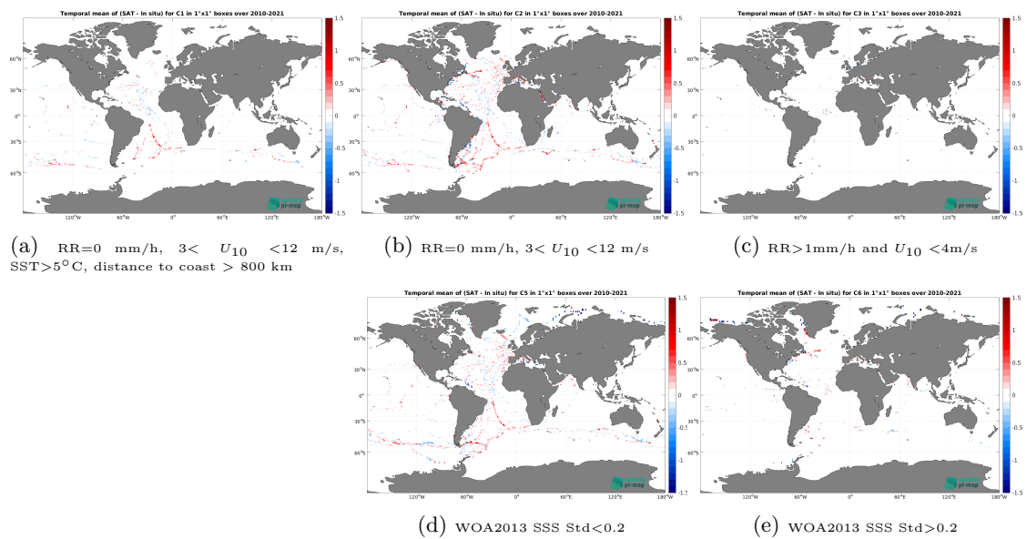
Figure 12: Temporal mean gridded over spatial boxes of size 1^\circ \times 1^\circ of \Delta SSS (SMOS SSS L3 v9 - 18 Days (CATDS-CEC-LOCEAN) - TSG (GOSUD-Sailing-ship)) for 5 different subdatasets corresponding to:RR=0 mm/h, 3 < U_{10} < 12 m/s, SST >5^\circ C, distance to coast > 800 km (a), RR=0 mm/h, 3 < U_{10} < 12 m/s (b), RR >1 mm/h and U_{10} < 4 m/s (c), WOA2013 SSS Std <0.2 (d), WOA2013 SSS Std >0.2 (e).
