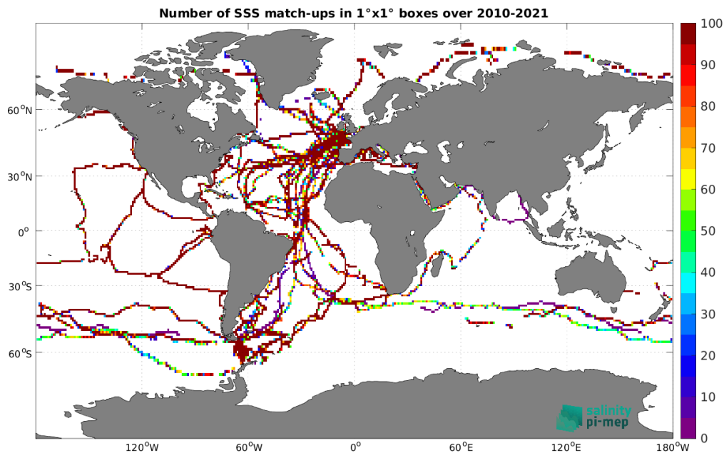
Figure 4: Number of SSS match-ups between TSG (GOSUD-Sailing-ship) SSS and the SMOS SSS L3 v9 - 18 Days (CATDS-CEC-LOCEAN) SSS product for the Global Ocean Pi-MEP region over 1^\circ \times 1^\circ boxes and for the full satellite product period.
