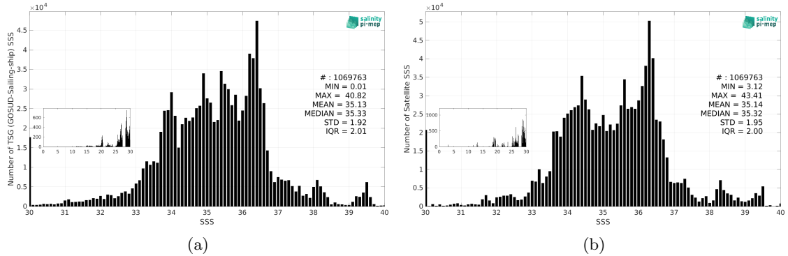
Figure 2: Histograms of SSS from TSG (GOSUD-Sailing-ship) (a) and SMOS SSS L3 v9 - 18 Days (CATDS-CEC-LOCEAN) (b) considering all match-up pairs per bins of 0.1 over the Global Ocean Pi-MEP region and for the full satellite product period.
