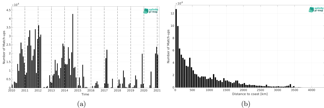
Figure 1: Number of match-ups between TSG (GOSUD-Sailing-ship) and SMOS SSS L3 v9 - 18 Days (CATDS-CEC-LOCEAN) SSS as a function of time (a) and as function of the distance to coast (b) over the Global Ocean Pi-MEP region and for the full satellite product period.
