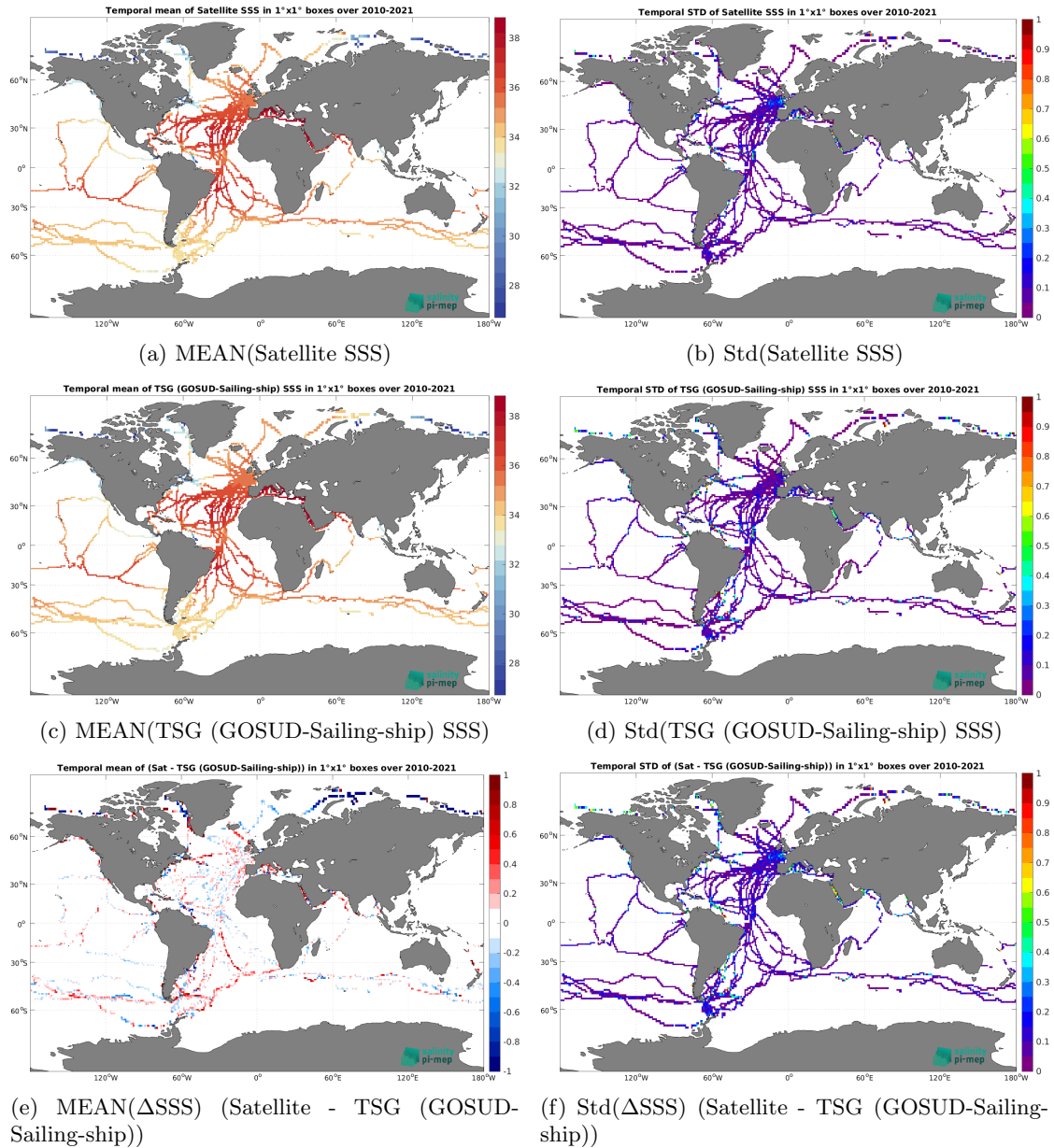
Figure 6: Temporal mean (left) and Std (right) of SSS from SMOS SSS L3 v9 - 18 Days (CATDS-CEC-LOCEAN) (top), TSG (GOSUD-Sailing-ship) (middle), and of \Delta SSS (Satellite - TSG (GOSUD-Sailing-ship)). Only match-up pairs are used to generate these maps.
