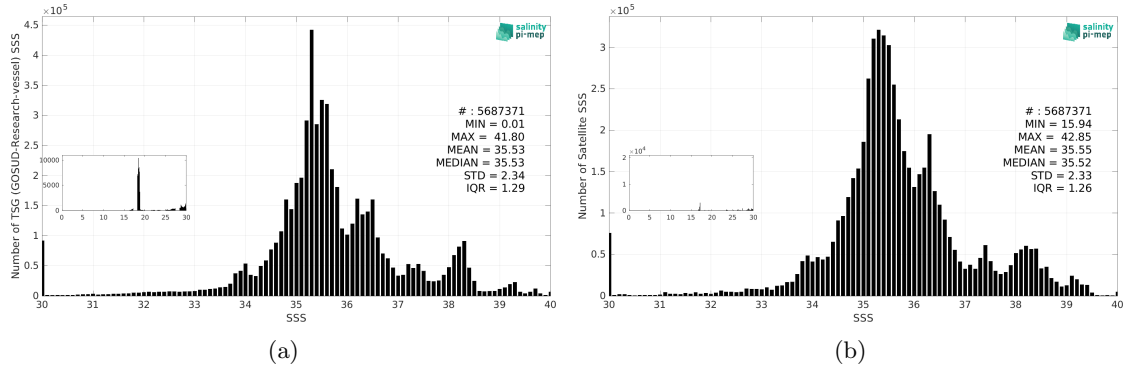
Figure 2: Histograms of SSS from TSG (GOSUD-Research-vessel) (a) and SMOS SSS L3 v9 - 18 Days (CATDS-CEC-LOCEAN) (b) considering all match-up pairs per bins of 0.1 over the Global Ocean Pi-MEP region and for the full satellite product period.
