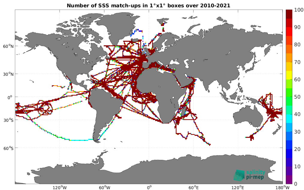
Figure 4: Number of SSS match-ups between TSG (GOSUD-Research-vessel) SSS and the SMOS SSS L3 v9 - 18 Days (CATDS-CEC-LOCEAN) SSS product for the Global Ocean Pi-MEP region over 1^\circ \times 1^\circ boxes and for the full satellite product period.
