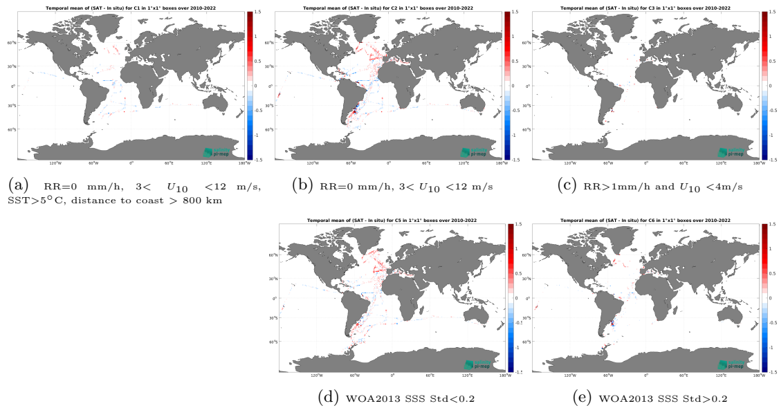
Figure 12: Temporal mean gridded over spatial boxes of size 1^\circ \times 1^\circ of \Delta SSS (SMOS SSS L3 v9 - 18 Days (CATDS-CEC-LOCEAN) - TSG (CSIC-UTM)) for 5 different subdatasets corresponding to: RR=0 mm/h, 3 < U_{10} < 12 m/s, SST > 5^\circ\text{C} , distance to coast > 800 km (a), RR=0 mm/h, 3 < U_{10} < 12 m/s (b), RR > 1\text{mm/h} and U_{10} < 4\text{m/s} (c), WOA2013 SSS Std < 0.2 (d), WOA2013 SSS Std > 0.2 (e).
