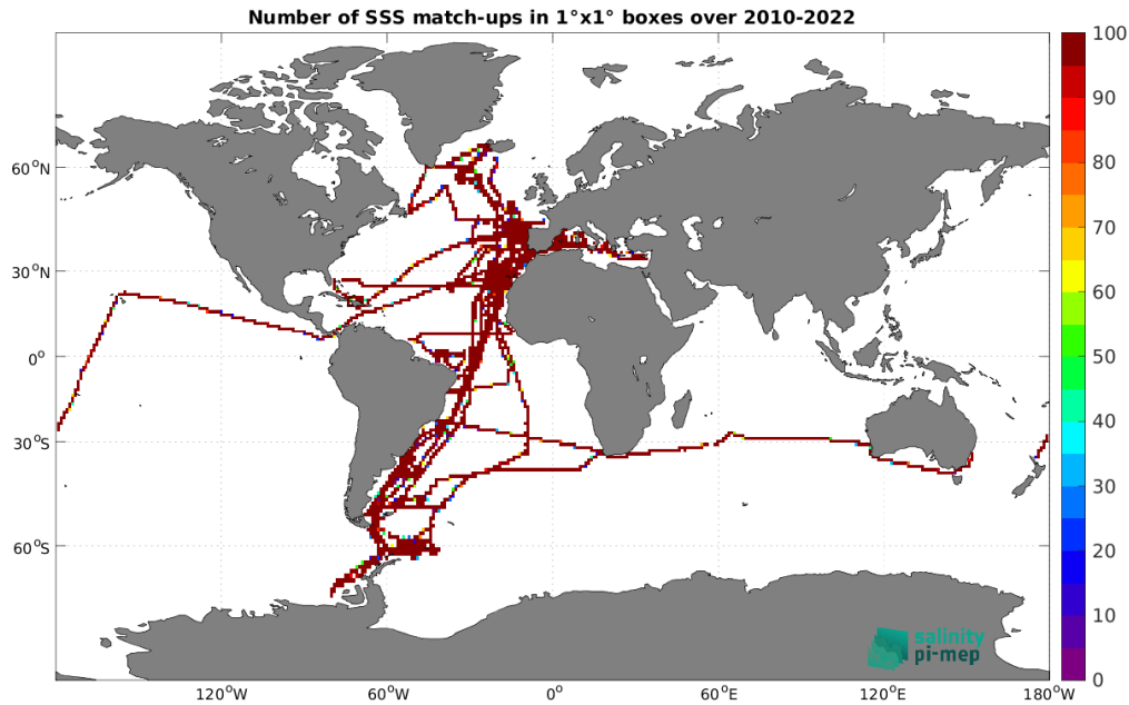
Figure 4: Number of SSS match-ups between TSG (CSIC-UTM) SSS and the SMOS SSS L3 v9 - 18 Days (CATDS-CEC-LOCEAN) SSS product for the Global Ocean Pi-MEP region over 1^\circ \times 1^\circ boxes and for the full satellite product period.
