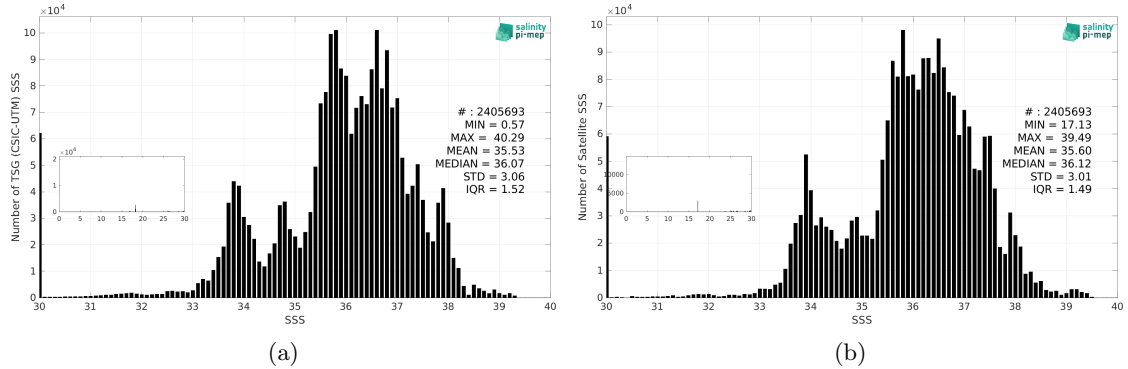
Figure 2: Histograms of SSS from TSG (CSIC-UTM) (a) and SMOS SSS L3 v9 - 18 Days (CATDS-CEC-LOCEAN) (b) considering all match-up pairs per bins of 0.1 over the Global Ocean Pi-MEP region and for the full satellite product period.
