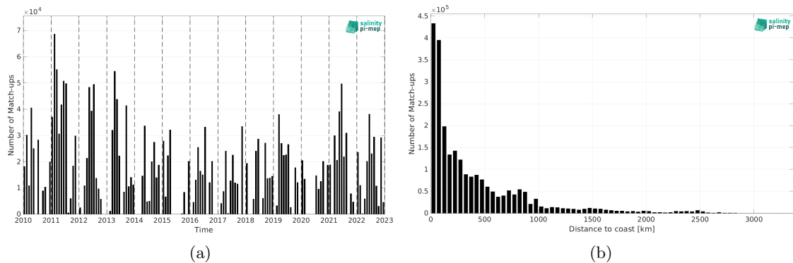
Figure 1: Number of match-ups between TSG (CSIC-UTM) and SMOS SSS L3 v9 - 18 Days (CATDS-CEC-LOCEAN) SSS as a function of time (a) and as function of the distance to coast (b) over the Global Ocean Pi-MEP region and for the full satellite product period.
