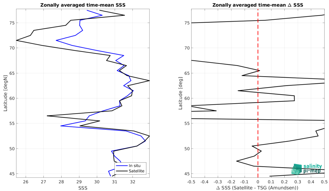
Figure 8: Left panel: Zonal mean SSS from SMOS SSS L3 v9 - 18 Days (CATDS-CEC-LOCEAN) satellite product (black) and from TSG (Amundsen) (blue). Right panel: Zonal mean of \Delta SSS (Satellite - TSG (Amundsen)) for all the collected Pi-MEP match-up pairs estimated over the full satellite product period.
