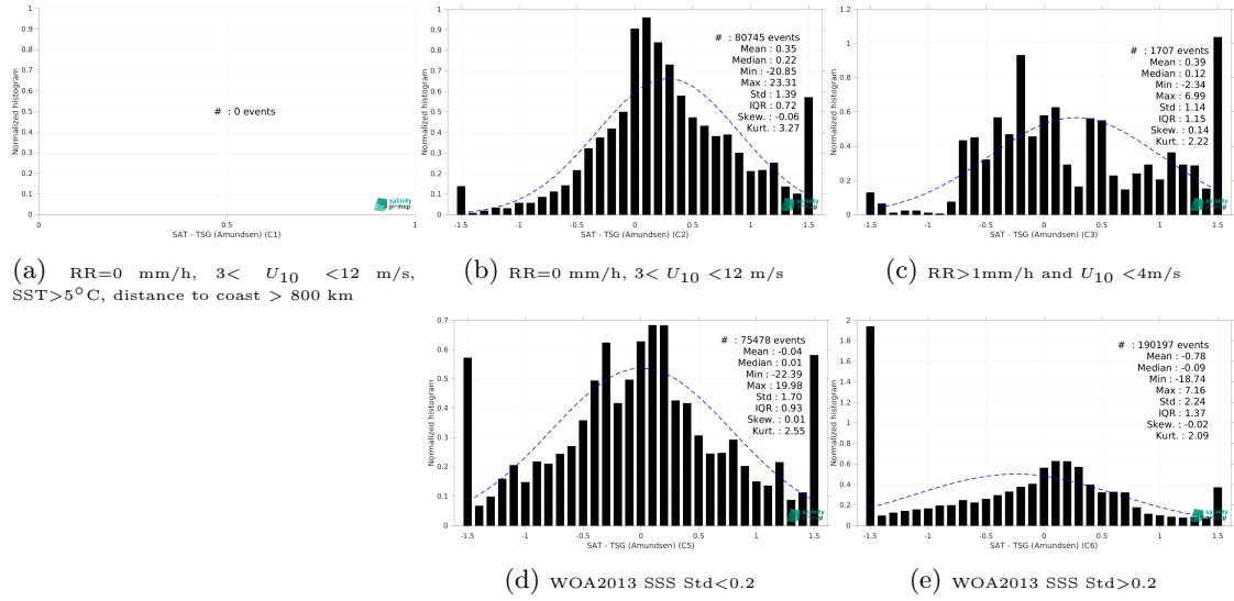
Figure 13: Normalized histogram of \Delta SSS (SMOS SSS L3 v9 - 18 Days (CATDS-CEC-LOCEAN) - TSG (Amundsen)) for 5 different subdatasets corresponding to: RR=0 mm/h, 3 < U_{10} < 12 m/s, SST > 5°C, distance to coast > 800 km (a), RR=0 mm/h, 3 < U_{10} < 12 m/s (b), RR > 1mm/h and U_{10} < 4 m/s (c), WOA2013 SSS Std < 0.2 (d), WOA2013 SSS Std > 0.2 (e).
