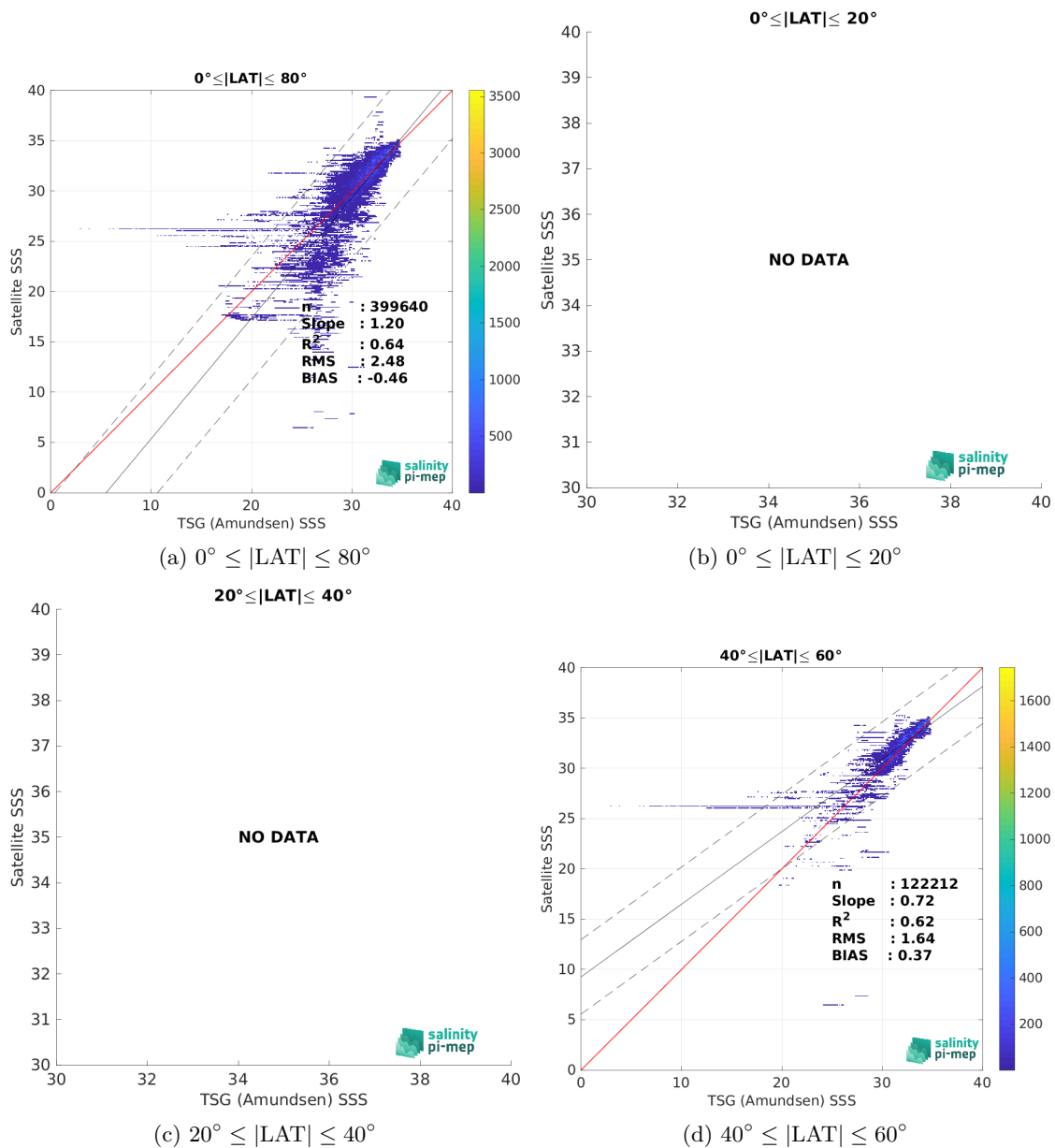
Figure 9: Contour maps of the concentration of SMOS SSS L3 v9 - 18 Days (CATDS-CEC-LOCEAN) SSS (y-axis) versus TSG (Amundsen) SSS (x-axis) at match-up pairs for different latitude bands. For each plot, the red line shows x=y . The black thin and dashed lines indicate a linear fit through the data cloud and the \pm 95\% confidence levels, respectively. The number match-up pairs n , the slope and R^2 coefficient of the linear fit, the root mean square (RMS) and the mean bias between satellite and in situ data are indicated for each latitude band in each plots.
