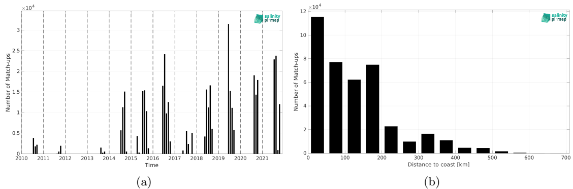
Figure 1: Number of match-ups between TSG (Amundsen) and SMOS SSS L3 v9 - 18 Days (CATDS-CEC-LOCEAN) SSS as a function of time (a) and as function of the distance to coast (b) over the Global Ocean Pi-MEP region and for the full satellite product period.
