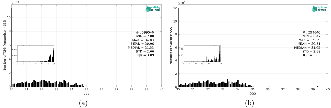
Figure 2: Histograms of SSS from TSG (Amundsen) (a) and SMOS SSS L3 v9 - 18 Days (CATDS-CEC-LOCEAN) (b) considering all match-up pairs per bins of 0.1 over the Global Ocean Pi-MEP region and for the full satellite product period.
