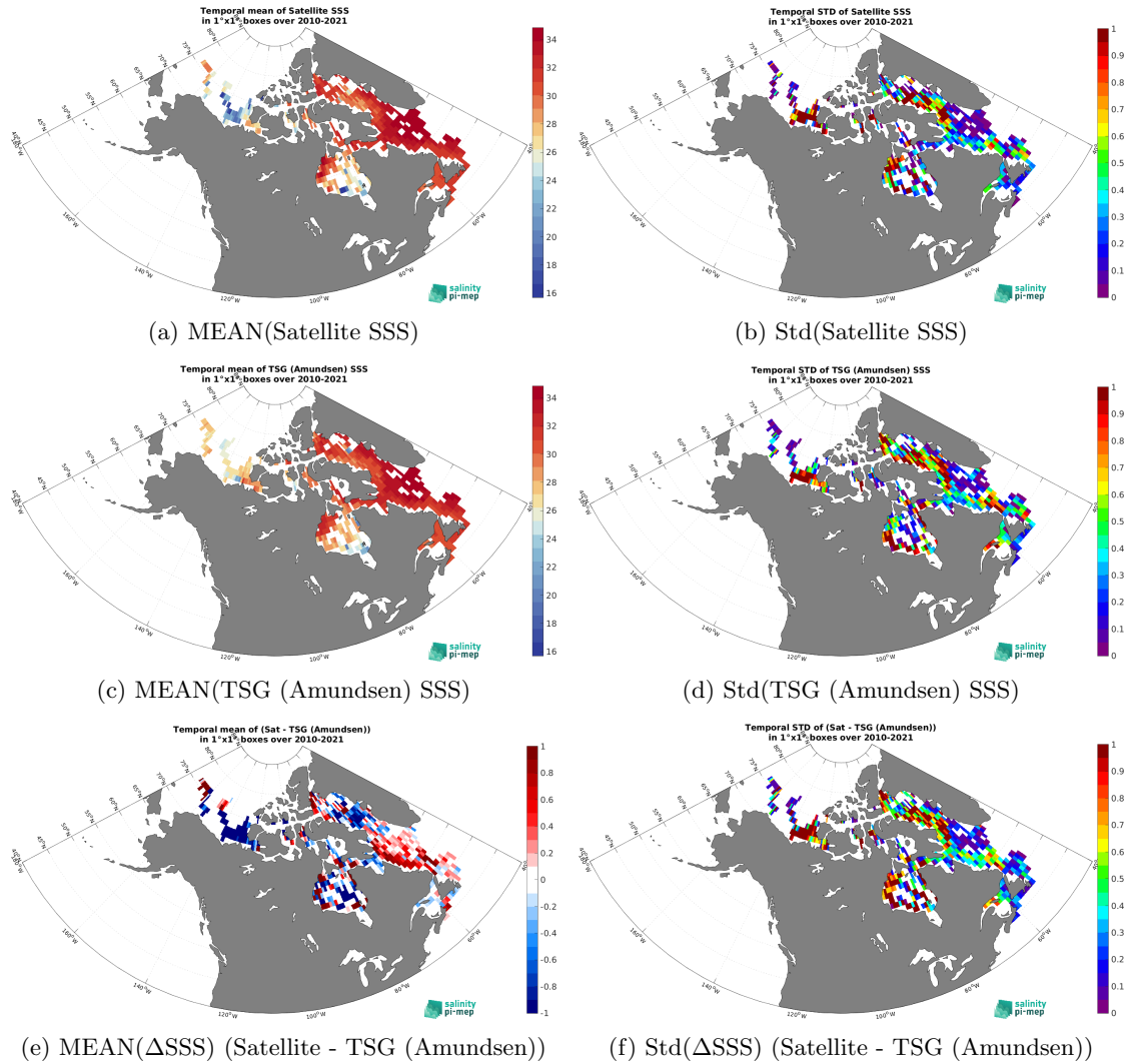
Figure 6: Temporal mean (left) and Std (right) of SSS from SMOS SSS L3 v9 - 18 Days (CATDS-CEC-LOCEAN) (top), TSG (Amundsen) (middle), and of \Delta SSS (Satellite - TSG (Amundsen)). Only match-up pairs are used to generate these maps.
