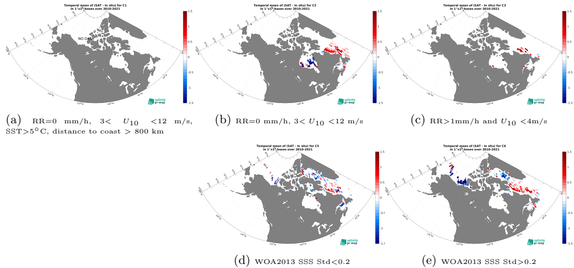
Figure 12: Temporal mean gridded over spatial boxes of size 1^{\circ}\times 1^{\circ} of \Delta\text{SSS} (SMOS SSS L3 v9 - 18 Days (CATDS-CEC-LOCEAN) - TSG (Amundsen)) for 5 different subdatasets corresponding to:RR=0 mm/h, 3 < U_{10} < 12 m/s, SST >5^{\circ}\text{C} , distance to coast > 800 km (a), RR=0 mm/h, 3 < U_{10} < 12 m/s (b), RR >1 mm/h and U_{10} < 4 m/s (c), WOA2013 SSS Std <0.2 (d), WOA2013 SSS Std >0.2 (e).
