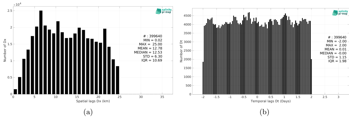
Figure 5: Histograms of the spatial (a) and temporal (b) lags between the location/time of the TSG (Amundsen) measurement and the date of the corresponding SMOS SSS L3 v9 - 18 Days (CATDS-CEC-LOCEAN) SSS pixel.
