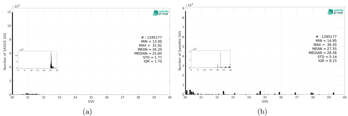
Figure 3: Histograms of SSS from SASSIE (a) and SMOS SSS L3 v9 - 18 Days (CATDS-CEC-LOCEAN) (b) considering all match-up pairs per bins of 0.1 over the Global Ocean Pi-MEP region and for the full satellite product period.
