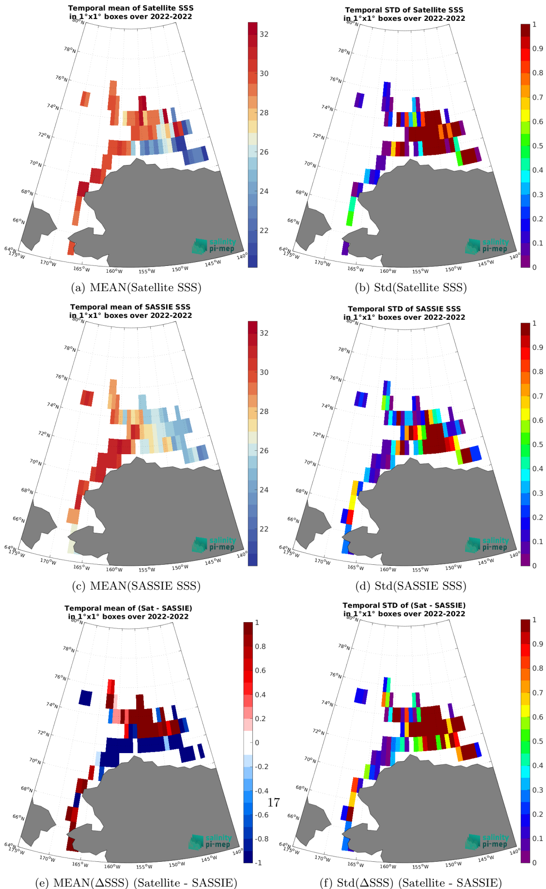
Figure 7: Temporal mean (left) and Std (right) of SSS from SMOS SSS L3 v9 - 18 Days (CATDS-CEC-LOCEAN) (top), SASSIE (middle), and of \Delta SSS (Satellite - SASSIE). Only match-up pairs are used to generate these maps.
