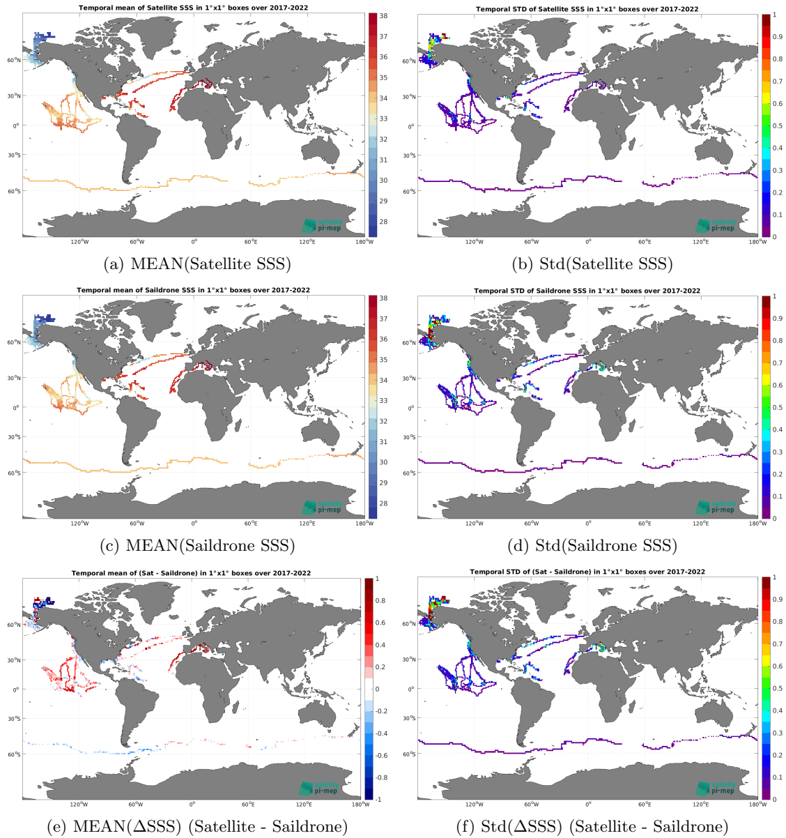
Figure 6: Temporal mean (left) and Std (right) of SSS from SMOS SSS L3 v9 - 18 Days (CATDS-CEC-LOCEAN) (top), Saildrone (middle), and of \Delta SSS (Satellite - Saildrone). Only match-up pairs are used to generate these maps.
