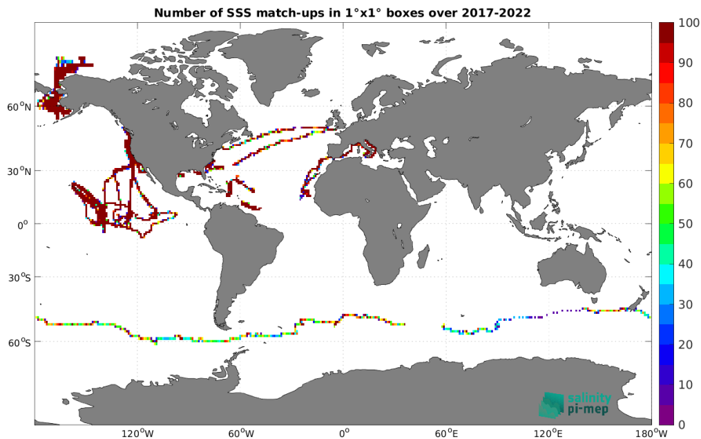
Figure 4: Number of SSS match-ups between Sailability SSS and the SMOS SSS L3 v9 - 18 Days (CATDS-CEC-LOCEAN) SSS product for the Global Ocean Pi-MEP region over 1^\circ \times 1^\circ boxes and for the full satellite product period.
