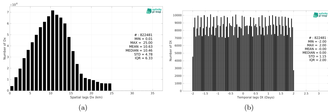
Figure 5: Histograms of the spatial (a) and temporal (b) lags between the location/time of the Sailability measurement and the date of the corresponding SMOS SSS L3 v9 - 18 Days (CATDS-CEC-LOCEAN) SSS pixel.
