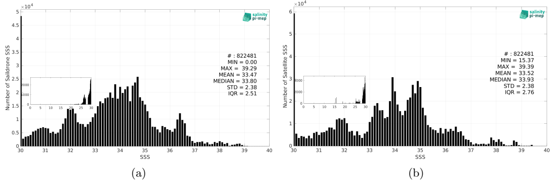
Figure 2: Histograms of SSS from Saildrone (a) and SMOS SSS L3 v9 - 18 Days (CATDS-CEC-LOCEAN) (b) considering all match-up pairs per bins of 0.1 over the Global Ocean Pi-MEP region and for the full satellite product period.
