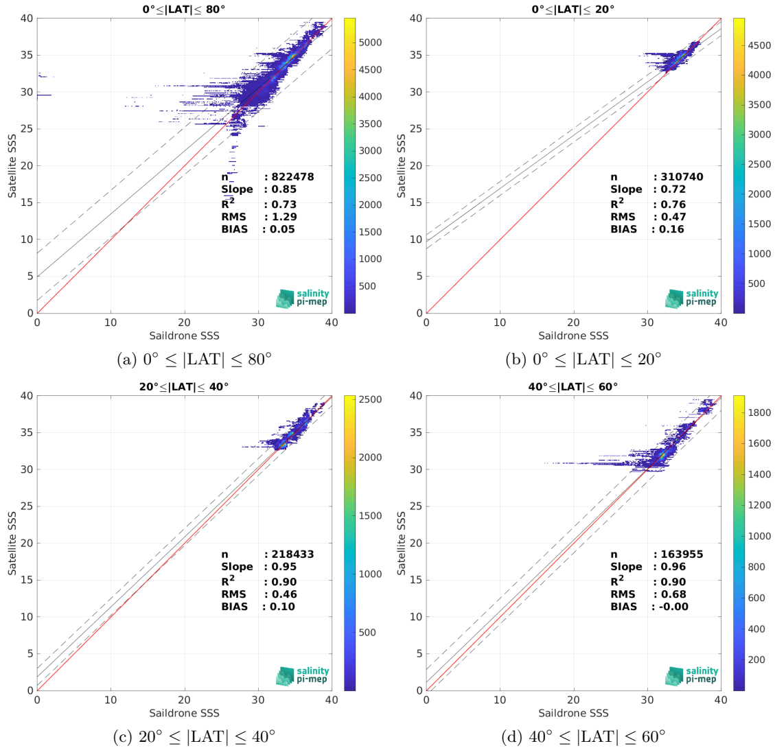
Figure 9: Contour maps of the concentration of SMOS SSS L3 v9 - 18 Days (CATDS-CEC-LOCEAN) SSS (y-axis) versus Saildrone SSS (x-axis) at match-up pairs for different latitude bands. For each plot, the red line shows x=y . The black thin and dashed lines indicate a linear fit through the data cloud and the \pm 95\% confidence levels, respectively. The number match-up pairs n , the slope and R^2 coefficient of the linear fit, the root mean square (RMS) and the mean bias between satellite and in situ data are indicated for each latitude band in each plots.
