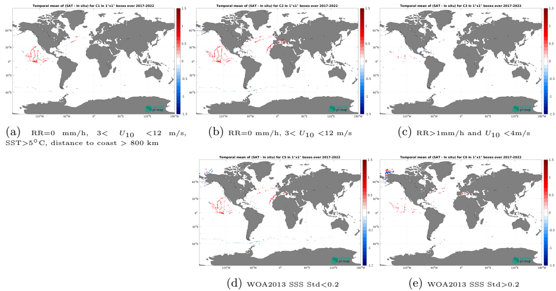
Figure 12: Temporal mean gridded over spatial boxes of size 1^\circ \times 1^\circ of \Delta SSS (SMOS SSS L3 v9 - 18 Days (CATDS-CEC-LOCEAN) - Saildrone) for 5 different subdatasets corresponding to:RR=0 mm/h, 3 < U_{10} < 12 m/s, SST > 5^\circ\text{C} , distance to coast > 800 km (a), RR=0 mm/h, 3 < U_{10} < 12 m/s (b), RR > 1 mm/h and U_{10} < 4 m/s (c), WOA2013 SSS Std < 0.2 (d), WOA2013 SSS Std > 0.2 (e).
