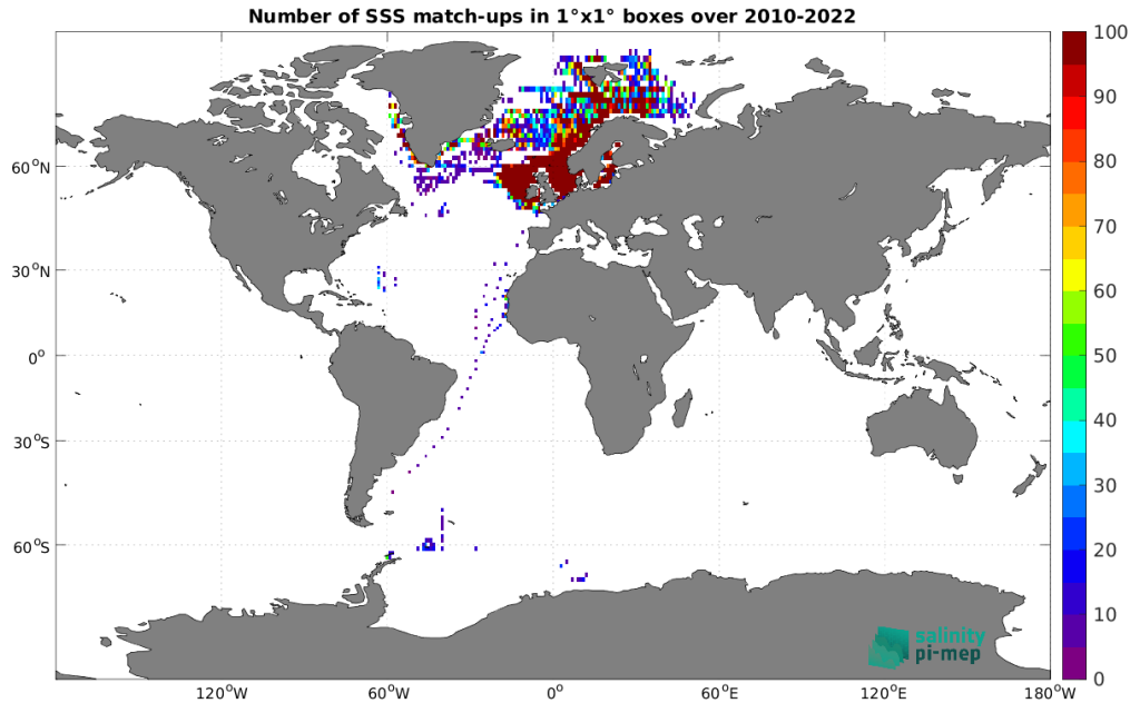
Figure 5: Number of SSS match-ups between ICES SSS and the SMOS SSS L3 v9 - 18 Days (CATDS-CEC-LOCEAN) SSS product for the Global Ocean Pi-MEP region over 1^\circ \times 1^\circ boxes and for the full satellite product period.
