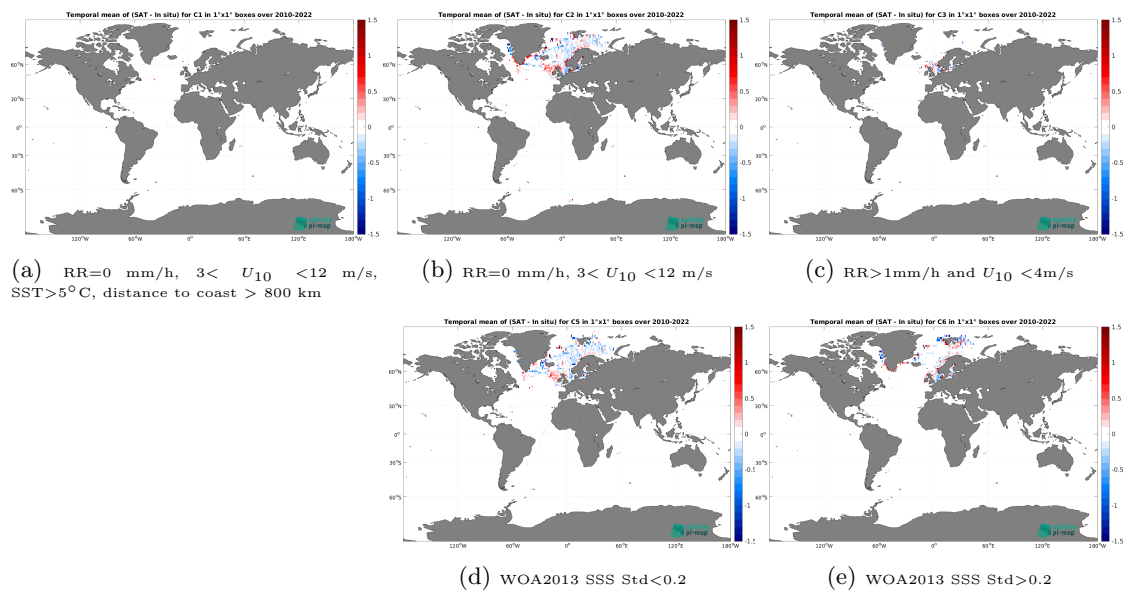
Figure 14: Temporal mean gridded over spatial boxes of size 1^\circ \times 1^\circ of \Delta SSS (SMOS SSS L3 v9 - 18 Days (CATDS-CEC-LOCEAN) - ICES) for 5 different subdatasets corresponding to:RR=0 mm/h, 3 < U_{10} < 12 m/s, SST > 5^\circ\text{C} , distance to coast > 800 km (a), RR=0 mm/h, 3 < U_{10} < 12 m/s (b), RR > 1 mm/h and U_{10} < 4 m/s (c), WOA2013 SSS Std < 0.2 (d), WOA2013 SSS Std > 0.2 (e).
