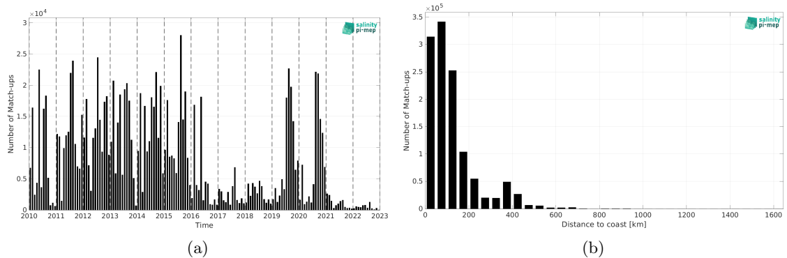
Figure 2: Number of match-ups between ICES and SMOS SSS L3 v9 - 18 Days (CATDS-CEC-LOCEAN) SSS as a function of time (a) and as function of the distance to coast (b) over the Global Ocean Pi-MEP region and for the full satellite product period.
