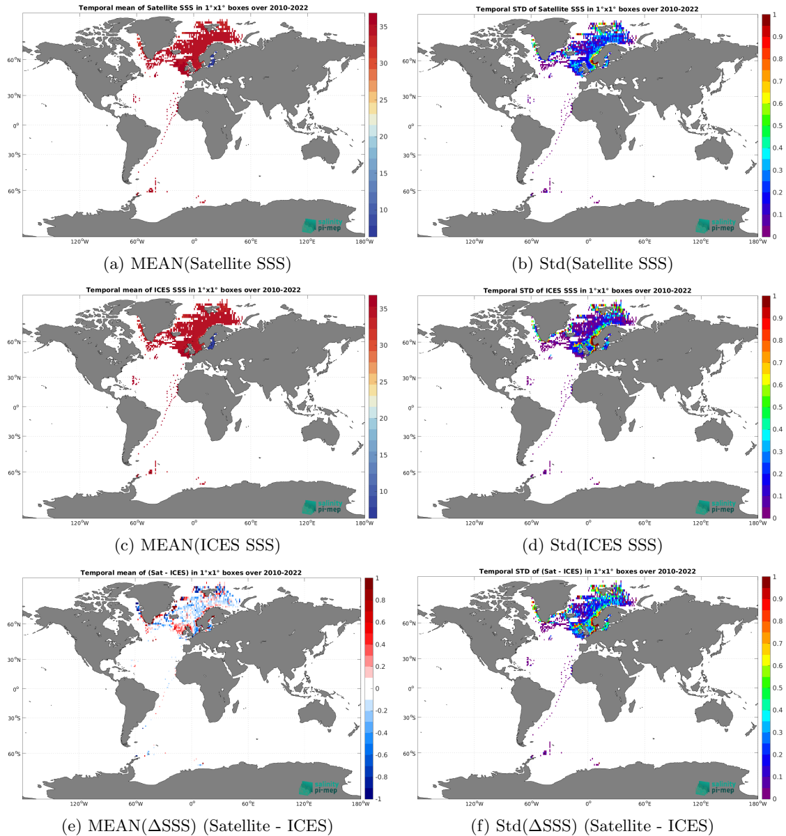
Figure 7: Temporal mean (left) and Std (right) of SSS from SMOS SSS L3 v9 - 18 Days (CATDS-CEC-LOCEAN) (top), ICES (middle), and of \Delta SSS (Satellite - ICES). Only match-up pairs are used to generate these maps.
