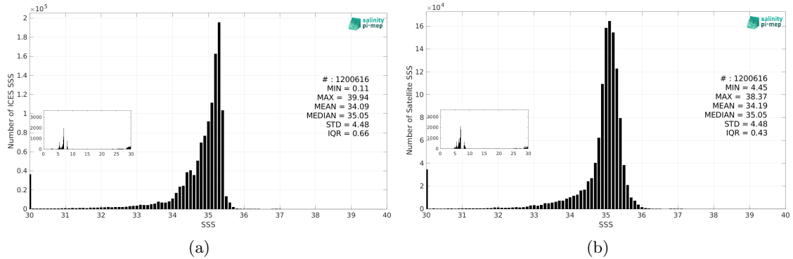
Figure 3: Histograms of SSS from ICES (a) and SMOS SSS L3 v9 - 18 Days (CATDS-CEC-LOCEAN) (b) considering all match-up pairs per bins of 0.1 over the Global Ocean Pi-MEP region and for the full satellite product period.
