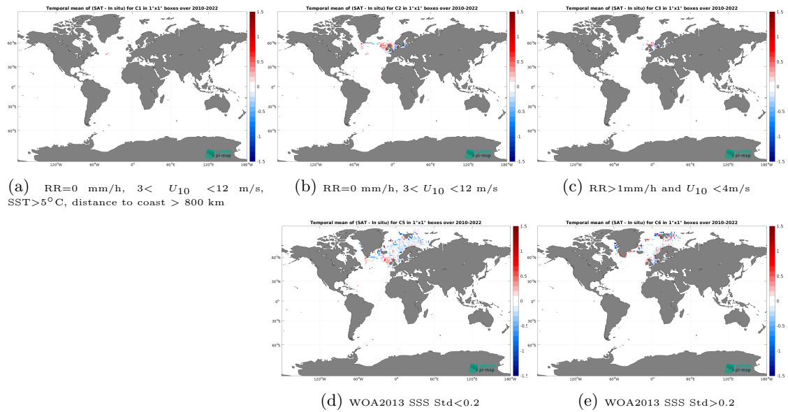
Figure 12: Temporal mean gridded over spatial boxes of size 1^\circ \times 1^\circ of \Delta SSS (SMOS SSS L3 v9 - 18 Days (CATDS-CEC-LOCEAN) - ICES) for 5 different subdatasets corresponding to:RR=0 mm/h, 3 < U_{10} < 12 m/s, SST > 5^\circ\text{C} , distance to coast > 800 km (a), RR=0 mm/h, 3 < U_{10} < 12 m/s (b), RR > 1 mm/h and U_{10} < 4 m/s (c), WOA2013 SSS Std < 0.2 (d), WOA2013 SSS Std > 0.2 (e).
