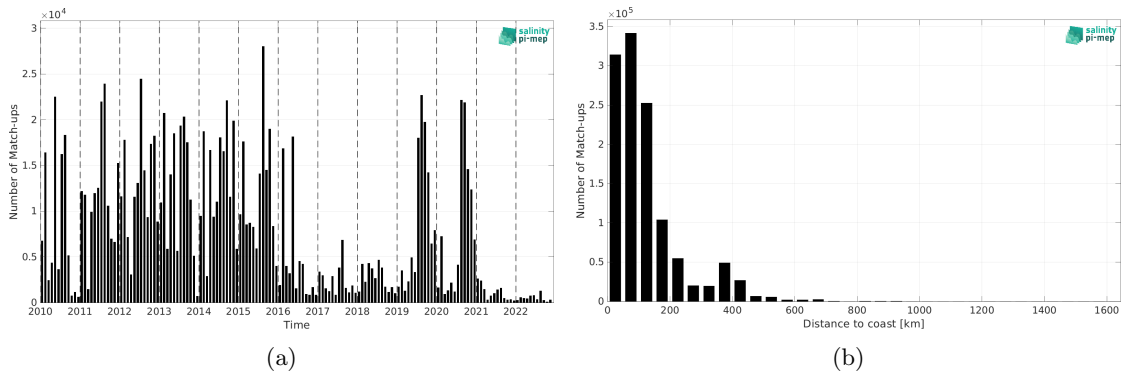
Figure 1: Number of match-ups between ICES and SMOS SSS L3 v9 - 18 Days (CATDS-CEC-LOCEAN) SSS as a function of time (a) and as function of the distance to coast (b) over the Global Ocean Pi-MEP region and for the full satellite product period.
