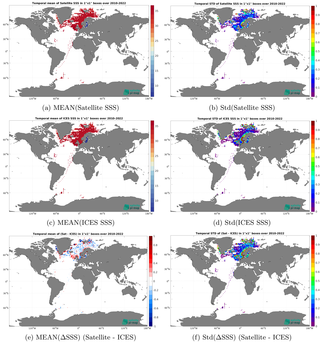
Figure 6: Temporal mean (left) and Std (right) of SSS from SMOS SSS L3 v9 - 18 Days (CATDS-CEC-LOCEAN) (top), ICES (middle), and of \Delta SSS (Satellite - ICES). Only match-up pairs are used to generate these maps.
