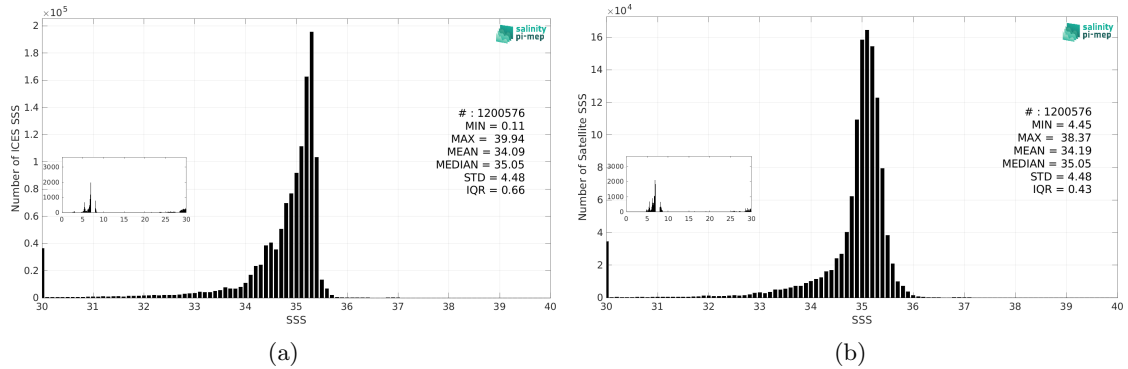
Figure 2: Histograms of SSS from ICES (a) and SMOS SSS L3 v9 - 18 Days (CATDS-CEC-LOCEAN) (b) considering all match-up pairs per bins of 0.1 over the Global Ocean Pi-MEP region and for the full satellite product period.
