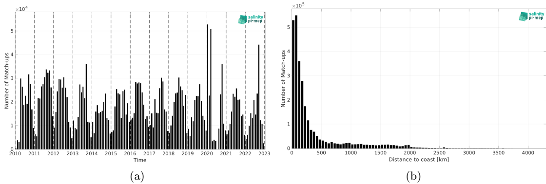
Figure 1: Number of match-ups between TSG (SAMOS) and SMOS SSS L3 v8 - 9 Days (CATDS-CEC-LOCEAN) SSS as a function of time (a) and as function of the distance to coast (b) over the Global Ocean Pi-MEP region and for the full satellite product period.
