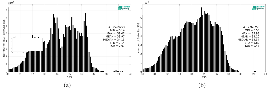
Figure 2: Histograms of SSS from TSG (SAMOS) (a) and SMOS SSS L3 v8 - 9 Days (CATDS-CEC-LOCEAN) (b) considering all match-up pairs per bins of 0.1 over the Global Ocean Pi-MEP region and for the full satellite product period.
