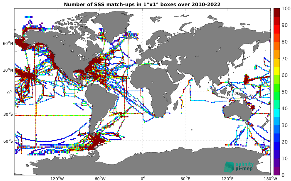
Figure 4: Number of SSS match-ups between TSG (SAMOS) SSS and the SMOS SSS L3 v8 - 9 Days (CATDS-CEC-LOCEAN) SSS product for the Global Ocean Pi-MEP region over 1^\circ \times 1^\circ boxes and for the full satellite product period.
