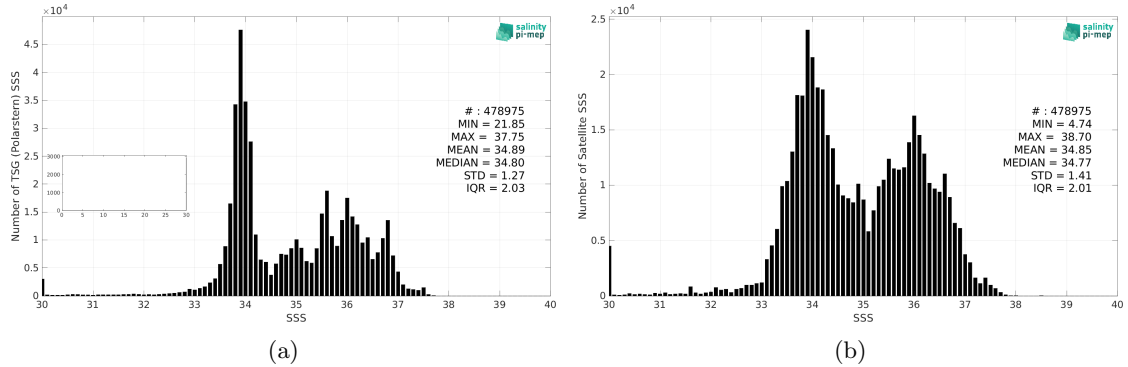
Figure 2: Histograms of SSS from TSG (Polarstern) (a) and SMOS SSS L3 v8 - 9 Days (CATDS-CEC-LOCEAN) (b) considering all match-up pairs per bins of 0.1 over the Global Ocean Pi-MEP region and for the full satellite product period.
