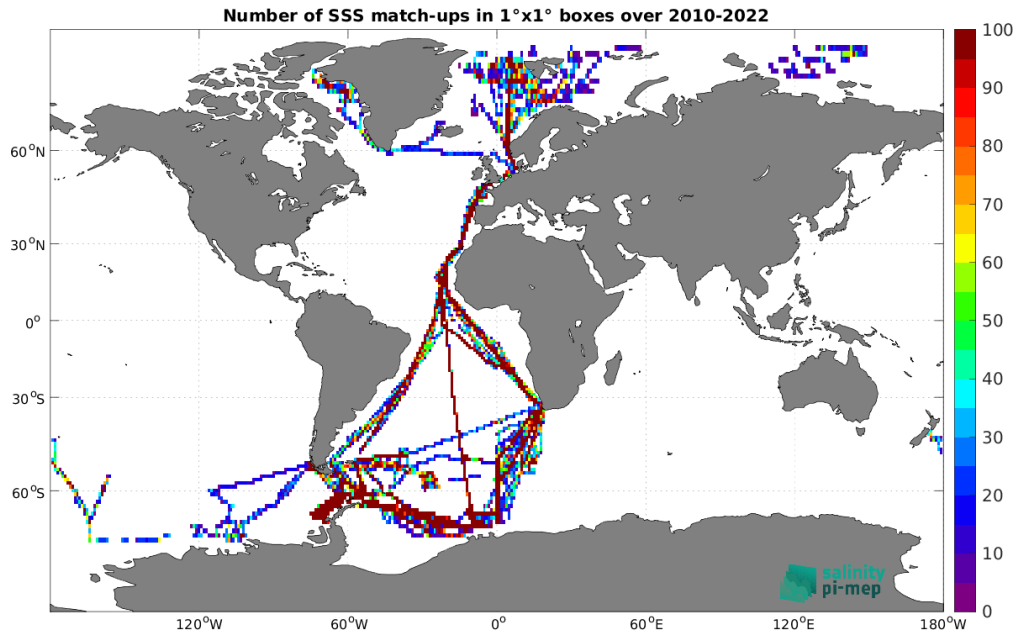
Figure 4: Number of SSS match-ups between TSG (Polarstern) SSS and the SMOS SSS L3 v8 - 9 Days (CATDS-CEC-LOCEAN) SSS product for the Global Ocean Pi-MEP region over 1°x1° boxes and for the full satellite product period.
