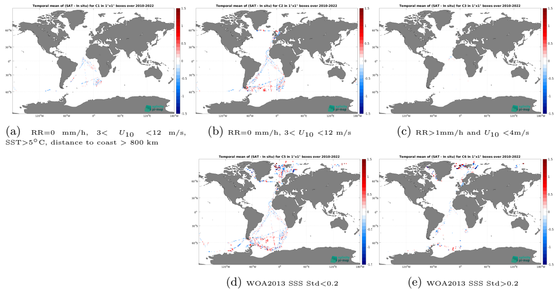
Figure 12: Temporal mean gridded over spatial boxes of size 1^\circ \times 1^\circ of \Delta SSS (SMOS SSS L3 v8 - 9 Days (CATDS-CEC-LOCEAN) - TSG (Polarstern)) for 5 different subdatasets corresponding to:RR=0 mm/h, 3 < U_{10} < 12 m/s, SST > 5^\circ\text{C} , distance to coast > 800 km (a), RR=0 mm/h, 3 < U_{10} < 12 m/s (b), RR > 1 mm/h and U_{10} < 4 m/s (c), WOA2013 SSS Std < 0.2 (d), WOA2013 SSS Std > 0.2 (e).
