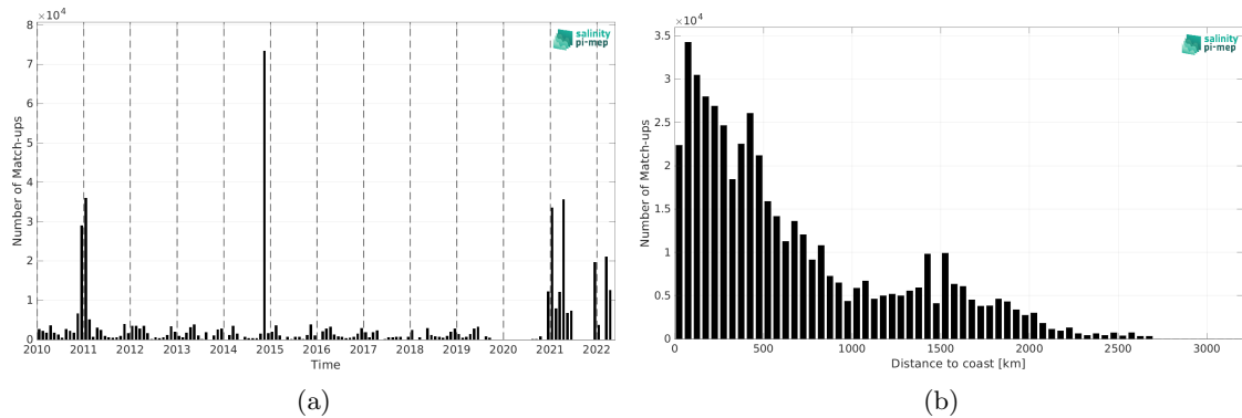
Figure 1: Number of match-ups between TSG (Polarstern) and SMOS SSS L3 v8 - 9 Days (CATDS-CEC-LOCEAN) SSS as a function of time (a) and as function of the distance to coast (b) over the Global Ocean Pi-MEP region and for the full satellite product period.
