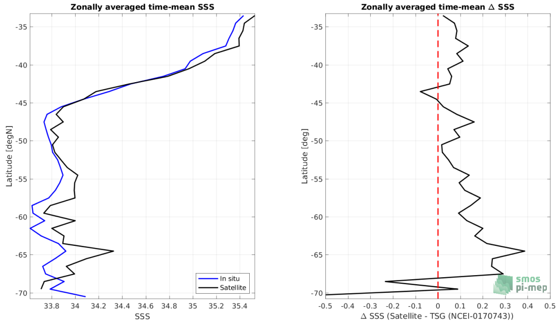
Figure 8: Left panel: Zonal mean SSS from SMOS SSS L3 v8 - 9 Days (CATDS-CECOS-LOCEAN) satellite product (black) and from TSG (NCEI-0170743) (blue). Right panel: Zonal mean of \Delta SSS (Satellite - TSG (NCEI-0170743)) for all the collected Pi-MEP match-up pairs estimated over the full satellite product period.
