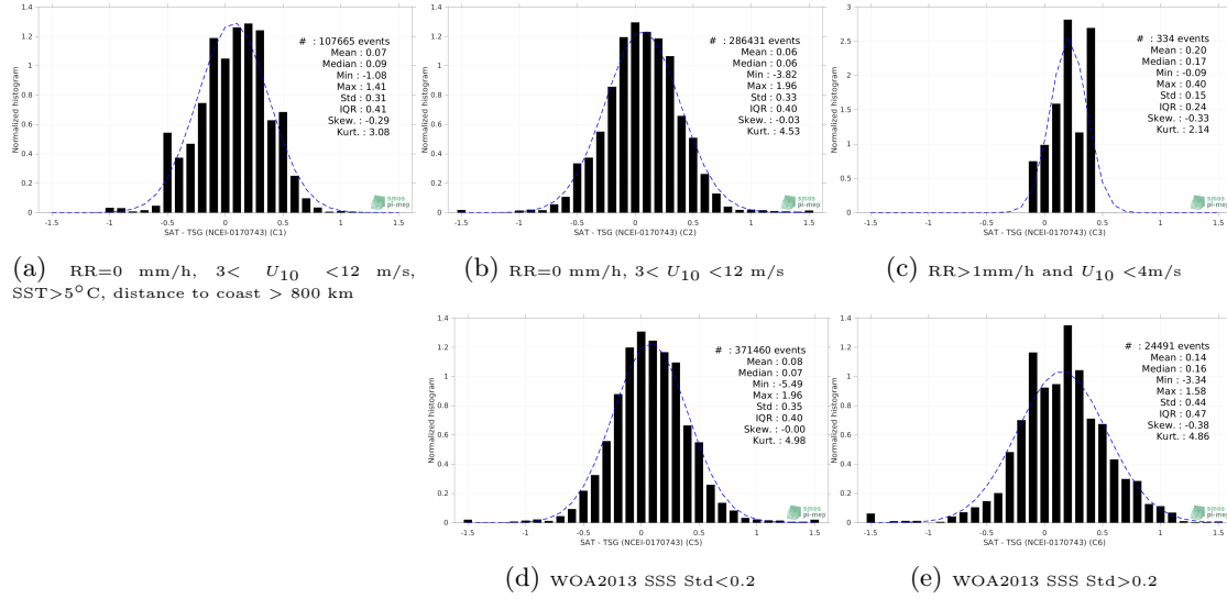
Figure 13: Normalized histogram of \Delta SSS (SMOS SSS L3 v8 - 9 Days (CATDS-CECOS-LOCEAN) - TSG (NCEI-0170743)) for 5 different subdatasets corresponding to: RR=0 mm/h, 3 < U_{10} < 12 m/s, SST > 5°C, distance to coast > 800 km (a), RR=0 mm/h, 3 < U_{10} < 12 m/s (b), RR > 1mm/h and U_{10} < 4 m/s (c), WOA2013 SSS Std < 0.2 (d), WOA2013 SSS Std > 0.2 (e).
