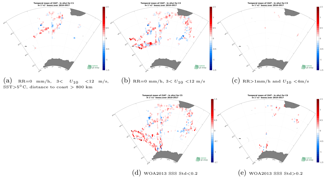
Figure 12: Temporal mean gridded over spatial boxes of size 1^{\circ}\times 1^{\circ} of \Delta\text{SSS} (SMOS SSS L3 v8 - 9 Days (CATDS-CECOS-LOCEAN) - TSG (NCEI-0170743)) for 5 different subdatasets corresponding to:RR=0 mm/h, 3 < U_{10} < 12 m/s, SST >5^{\circ}\text{C} , distance to coast > 800 km (a), RR=0 mm/h, 3 < U_{10} < 12 m/s (b), RR >1 mm/h and U_{10} < 4 m/s (c), WOA2013 SSS Std <0.2 (d), WOA2013 SSS Std >0.2 (e).
