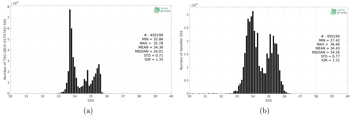
Figure 2: Histograms of SSS from TSG (NCEI-0170743) (a) and SMOS SSS L3 v8 - 9 Days (CATDS-CECOS-LOCEAN) (b) considering all match-up pairs per bins of 0.1 over the Global Ocean Pi-MEP region and for the full satellite product period.
