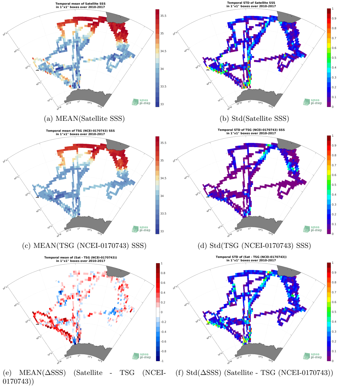
Figure 6: Temporal mean (left) and Std (right) of SSS from SMOS SSS L3 v8 - 9 Days (CATDS-CECOS-LOCEAN) (top), TSG (NCEI-0170743) (middle), and of \Delta SSS (Satellite - TSG (NCEI-0170743)). Only match-up pairs are used to generate these maps.
