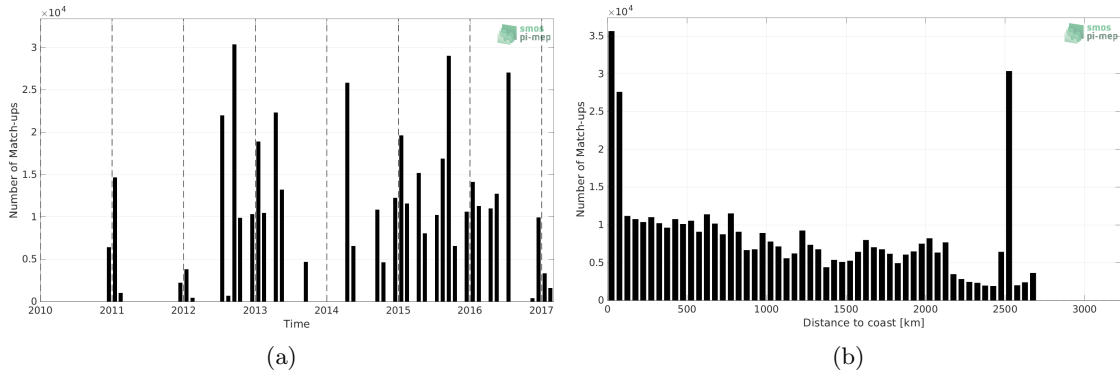
Figure 1: Number of match-ups between TSG (NCEI-0170743) and SMOS SSS L3 v8 - 9 Days (CATDS-CECOS-LOCEAN) SSS as a function of time (a) and as function of the distance to coast (b) over the Global Ocean Pi-MEP region and for the full satellite product period.
