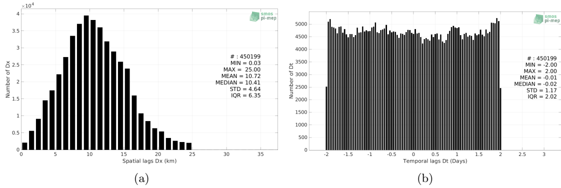
Figure 5: Histograms of the spatial (a) and temporal (b) lags between the location/time of the TSG (NCEI-0170743) measurement and the date of the corresponding SMOS SSS L3 v8 - 9 Days (CATDS-CECOS-LOCEAN) SSS pixel.
