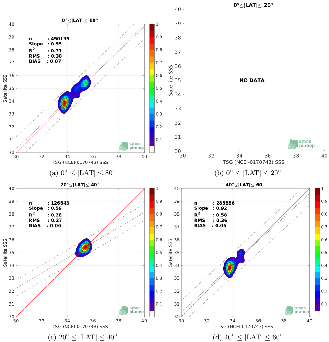
Figure 9: Contour maps of the concentration of SMOS SSS L3 v8 - 9 Days (CATDS-CECOS-LOCEAN) SSS (y-axis) versus TSG (NCEI-0170743) SSS (x-axis) at match-up pairs for different latitude bands. For each plot, the red line shows x=y . The black thin and dashed lines indicate a linear fit through the data cloud and the \pm 95\% confidence levels, respectively. The number match-up pairs n , the slope and R^2 coefficient of the linear fit, the root mean square (RMS) and the mean bias between satellite and in situ data are indicated for each latitude band in each plots.
