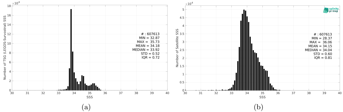
Figure 2: Histograms of SSS from TSG (LEGOS-Survostral) (a) and SMOS SSS L3 v8 - 9 Days (CATDS-CEC-LOCEAN) (b) considering all match-up pairs per bins of 0.1 over the Global Ocean Pi-MEP region and for the full satellite product period.
