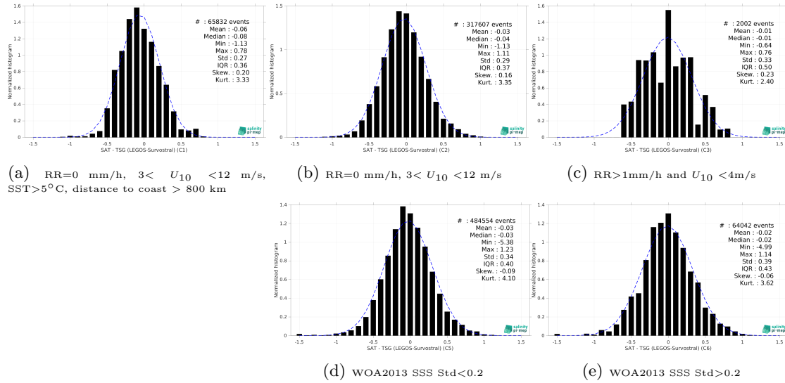
Figure 13: Normalized histogram of \Delta SSS (SMOS SSS L3 v8 - 9 Days (CATDS-CEC-LOCEAN) - TSG (LEGOS-Survostral)) for 5 different subdatasets corresponding to: RR=0 mm/h, 3 < U_{10} < 12 m/s, SST>5°C, distance to coast > 800 km (a), RR=0 mm/h, 3 < U_{10} < 12 m/s (b), RR>1mm/h and U_{10} < 4 m/s (c), WOA2013 SSS Std<0.2 (d), WOA2013 SSS Std>0.2 (e).
