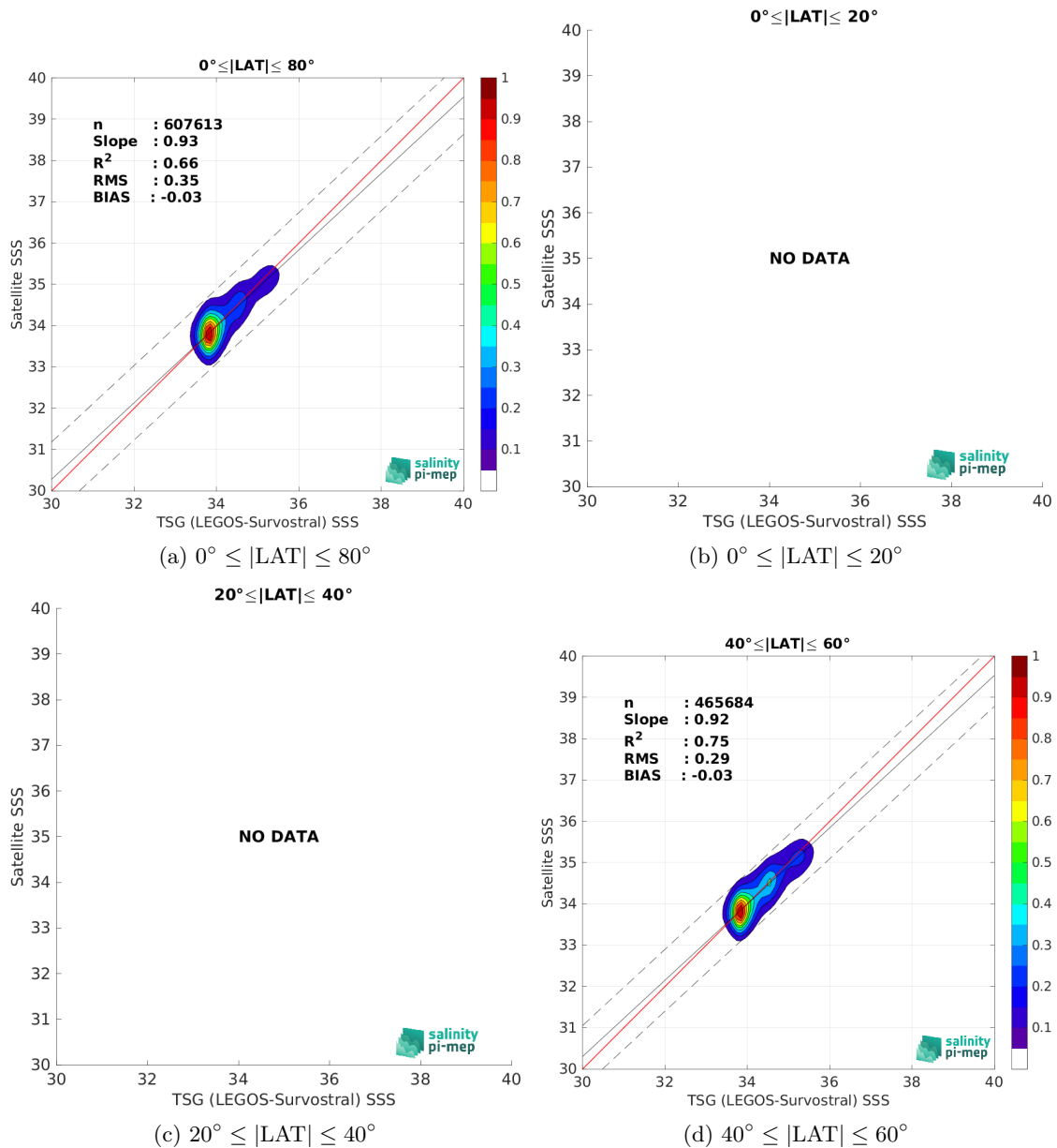
Figure 9: Contour maps of the concentration of SMOS SSS L3 v8 - 9 Days (CATDS-CEC-LOCEAN) SSS (y-axis) versus TSG (LEGOS-Survostral) SSS (x-axis) at match-up pairs for different latitude bands. For each plot, the red line shows x=y . The black thin and dashed lines indicate a linear fit through the data cloud and the \pm 95\% confidence levels, respectively. The number match-up pairs n , the slope and R^2 coefficient of the linear fit, the root mean square (RMS) and the mean bias between satellite and in situ data are indicated for each latitude band in each plots.
