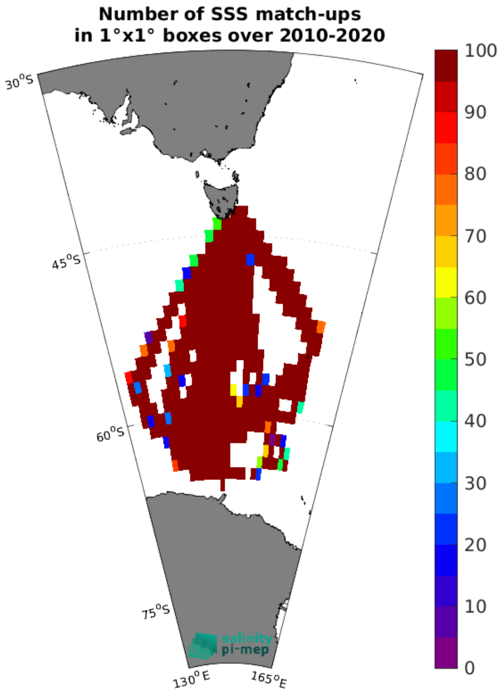
Figure 4: Number of SSS match-ups between TSG (LEGOS-Survostral) SSS and the SMOS SSS L3 v8 - 9 Days (CATDS-CEC-LOCEAN) SSS product for the Global Ocean Pi-MEP region over 1°x1° boxes and for the full satellite product period.
