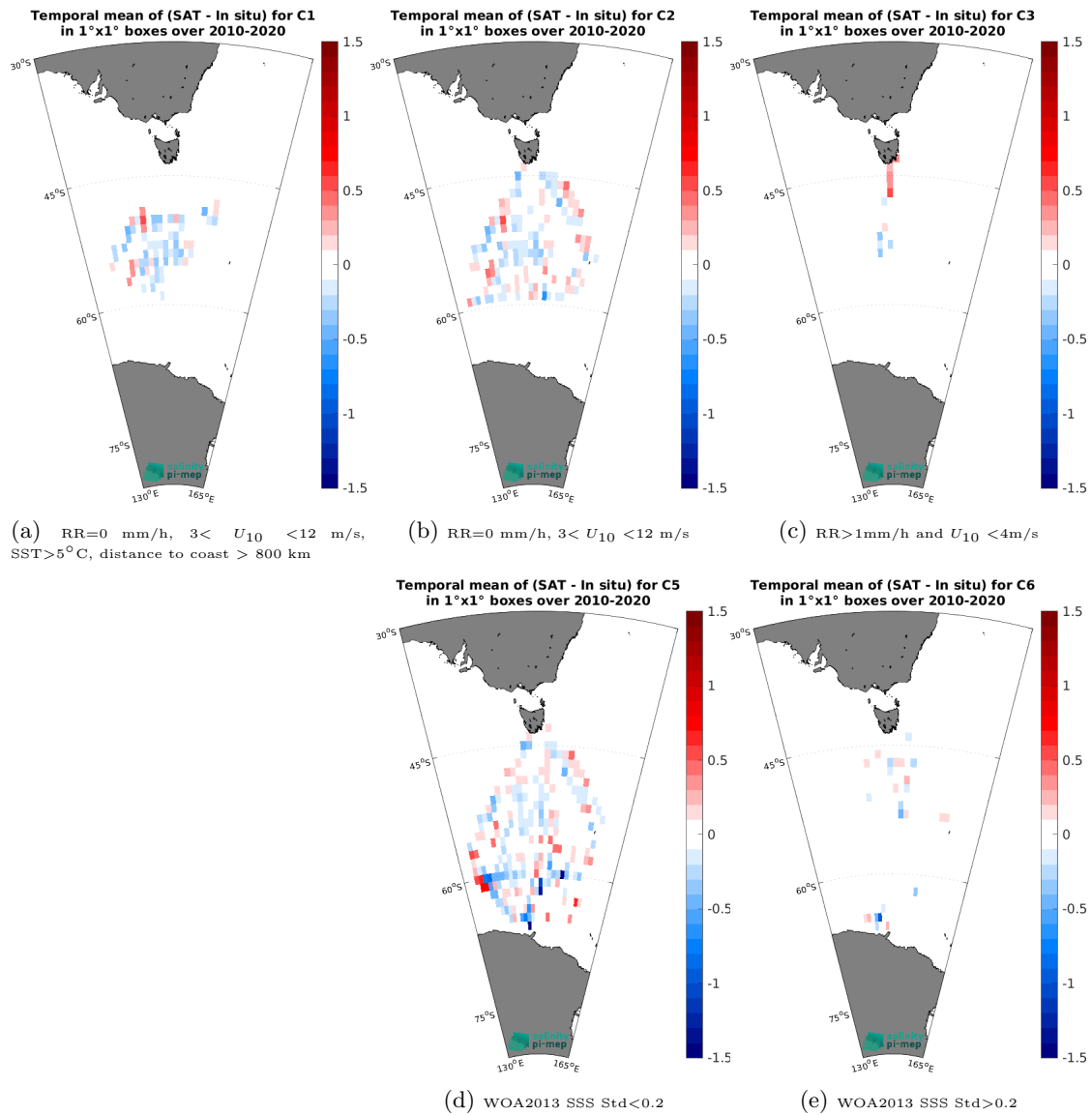
Figure 12: Temporal mean gridded over spatial boxes of size 1^\circ \times 1^\circ of \Delta\text{SSS} (SMOS SSS L3 v8 - 9 Days (CATDS-CEC-LOCEAN) - TSG (LEGOS-Survostral)) for 5 different subdatasets corresponding to: RR=0 mm/h, 3 < U_{10} < 12 m/s, SST > 5^\circ\text{C} , distance to coast > 800 km (a), RR=0 mm/h, 3 < U_{10} < 12 m/s (b), RR > 1 mm/h and U_{10} < 4 m/s (c), WOA2013 SSS Std < 0.2 (d), WOA2013 SSS Std > 0.2 (e).
