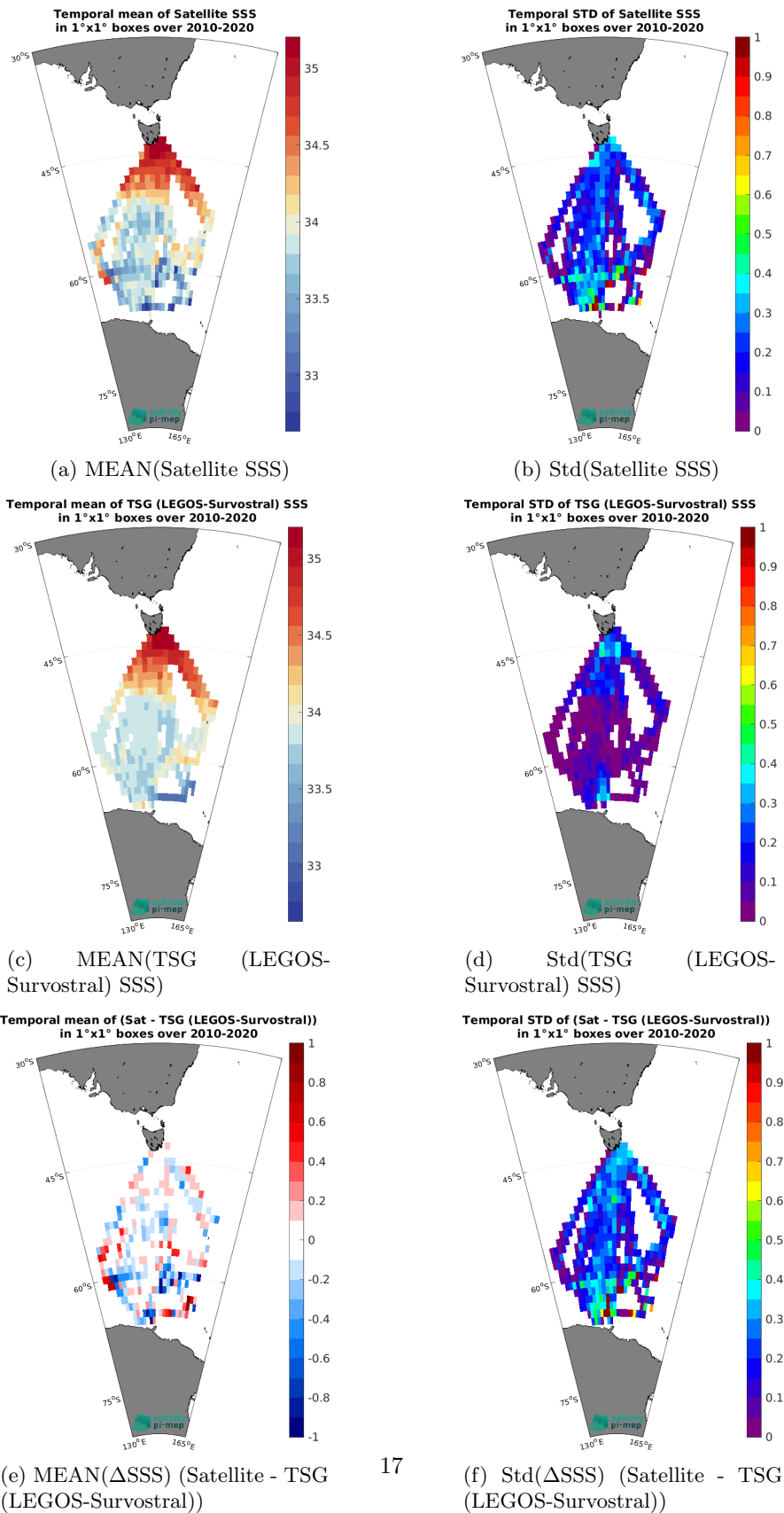
Figure 6: Temporal mean (left) and Std (right) of SSS from SMOS SSS L3 v8 - 9 Days (CATDS-CEC-LOCEAN) (top), TSG (LEGOS-Survostral) (middle), and of \Delta SSS (Satellite - TSG (LEGOS-Survostral)). Only match-up pairs are used to generate these maps.
