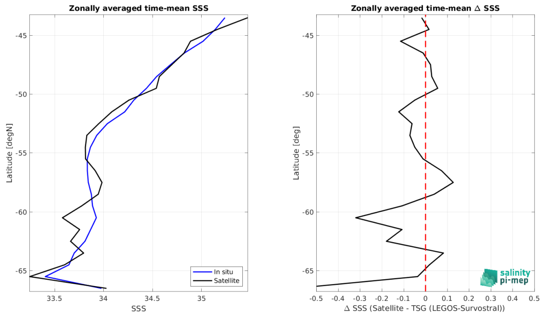
Figure 8: Left panel: Zonal mean SSS from SMOS SSS L3 v8 - 9 Days (CATDS-CEC-LOCEAN) satellite product (black) and from TSG (LEGOS-Survostral) (blue). Right panel: Zonal mean of \Delta SSS (Satellite - TSG (LEGOS-Survostral)) for all the collected Pi-MEP match-up pairs estimated over the full satellite product period.
