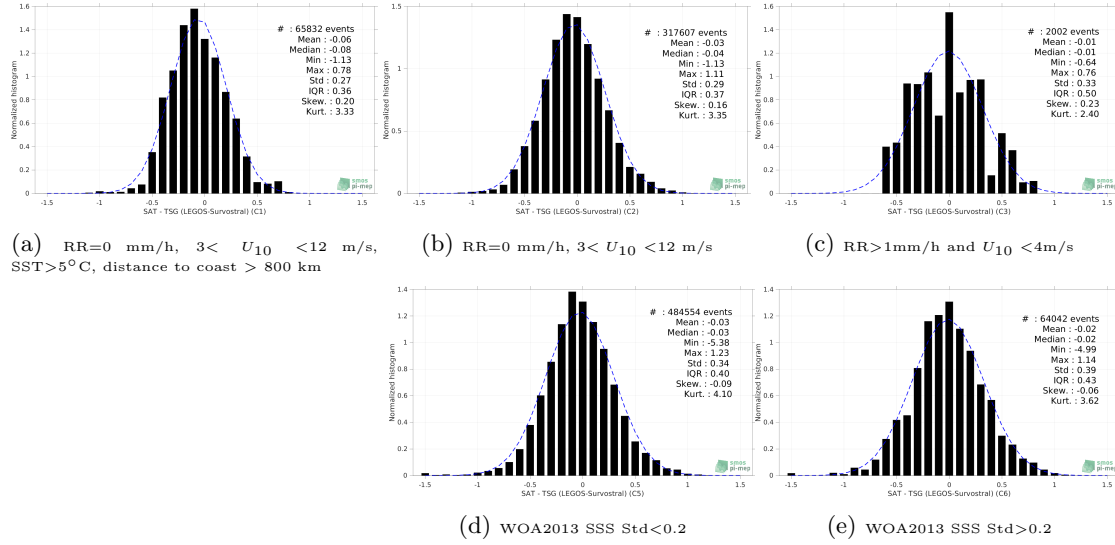
Figure 13: Normalized histogram of \Delta SSS (SMOS SSS L3 v8 - 9 Days (CATDS-CECOS-LOCEAN) - TSG (LEGOS-Survostral)) for 5 different subdatasets corresponding to: RR=0 mm/h, 3 < U_{10} < 12 m/s, SST>5°C, distance to coast > 800 km (a), RR=0 mm/h, 3 < U_{10} < 12 m/s (b), RR>1mm/h and U_{10} < 4 m/s (c), WOA2013 SSS Std<0.2 (d), WOA2013 SSS Std>0.2 (e).
