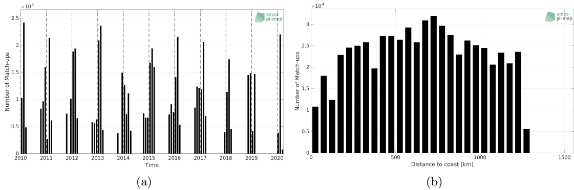
Figure 1: Number of match-ups between TSG (LEGOS-Survostral) and SMOS SSS L3 v8 - 9 Days (CATDS-CECOS-LOCEAN) SSS as a function of time (a) and as function of the distance to coast (b) over the Global Ocean Pi-MEP region and for the full satellite product period.
