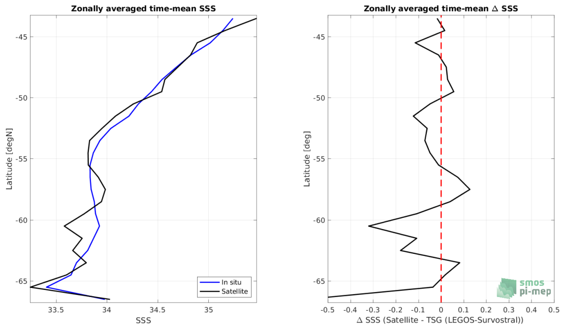
Figure 8: Left panel: Zonal mean SSS from SMOS SSS L3 v8 - 9 Days (CATDS-CECOS-LOCEAN) satellite product (black) and from TSG (LEGOS-Survostral) (blue). Right panel: Zonal mean of \Delta SSS (Satellite - TSG (LEGOS-Survostral)) for all the collected Pi-MEP match-up pairs estimated over the full satellite product period.
