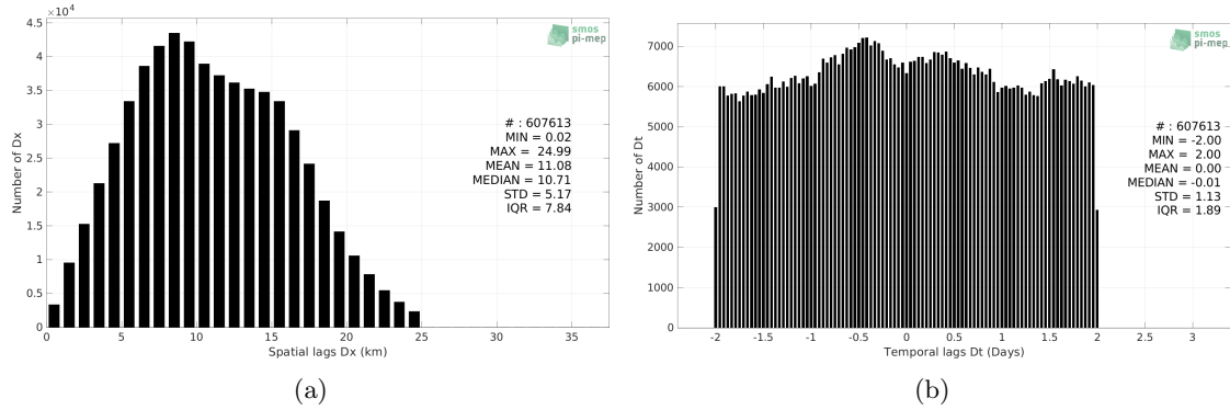
Figure 5: Histograms of the spatial (a) and temporal (b) lags between the location/time of the TSG (LEGOS-Survostral) measurement and the date of the corresponding SMOS SSS L3 v8 - 9 Days (CATDS-CECOS-LOCEAN) SSS pixel.
