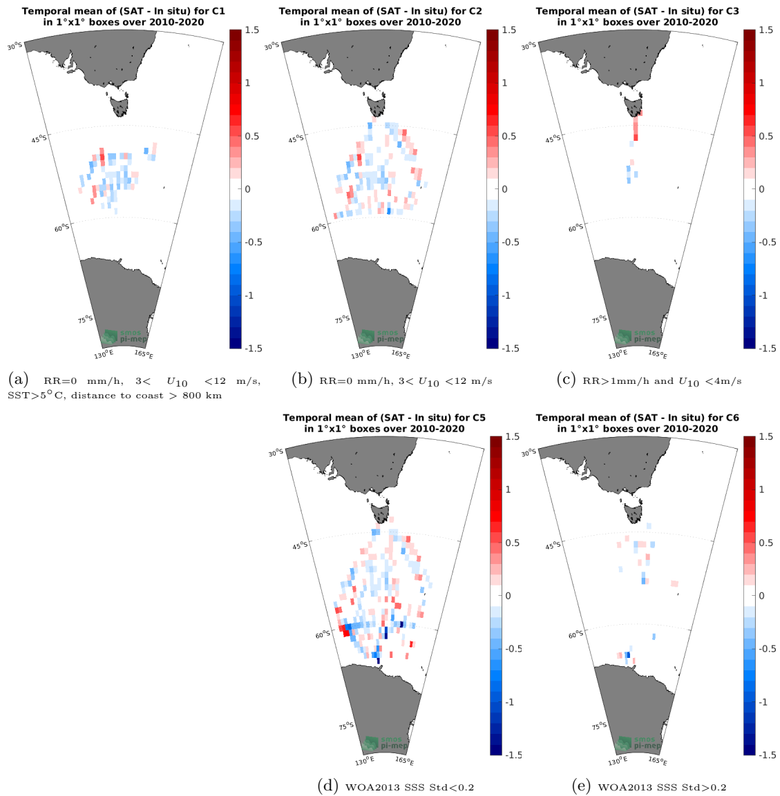
Figure 12: Temporal mean gridded over spatial boxes of size 1^\circ \times 1^\circ of \Delta SSS (SMOS SSS L3 v8 - 9 Days (CATDS-CECOS-LOCEAN) - TSG (LEGOS-Survostral)) for 5 different subdatasets corresponding to:RR=0 mm/h, 3 < U_{10} < 12 m/s, SST>5°C, distance to coast > 800 km (a), RR=0 mm/h, 3 < U_{10} < 12 m/s (b), RR>1mm/h and U_{10} < 4 m/s (c), WOA2013 SSS Std<0.2 (d), WOA2013 SSS Std>0.2 (e).
