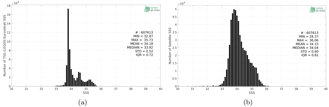
Figure 2: Histograms of SSS from TSG (LEGOS-Survostral) (a) and SMOS SSS L3 v8 - 9 Days (CATDS-CECOS-LOCEAN) (b) considering all match-up pairs per bins of 0.1 over the Global Ocean Pi-MEP region and for the full satellite product period.
