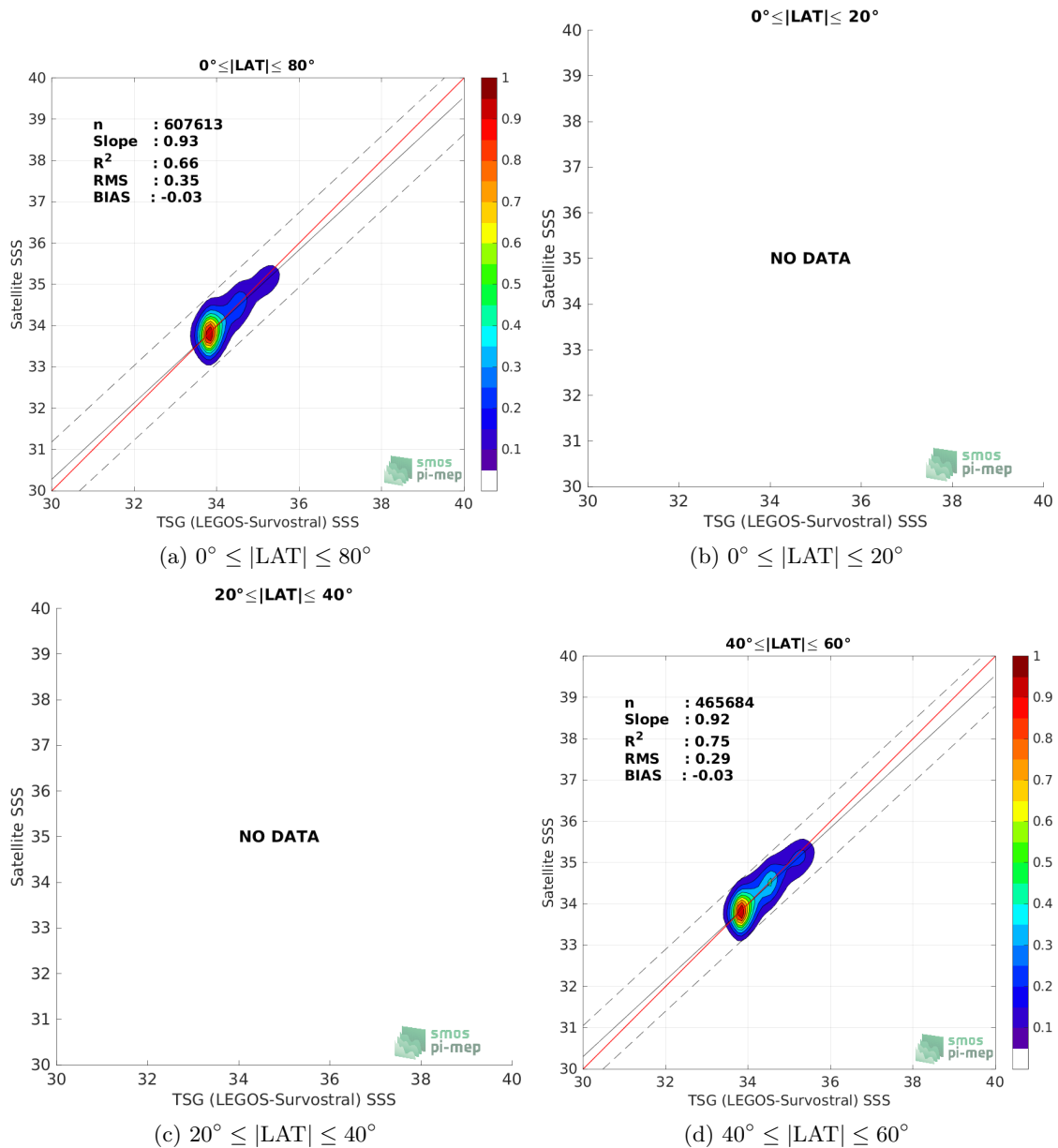
Figure 9: Contour maps of the concentration of SMOS SSS L3 v8 - 9 Days (CATDS-CECOS-LOCEAN) SSS (y-axis) versus TSG (LEGOS-Survostral) SSS (x-axis) at match-up pairs for different latitude bands. For each plot, the red line shows x=y . The black thin and dashed lines indicate a linear fit through the data cloud and the \pm 95\% confidence levels, respectively. The number match-up pairs n , the slope and R^2 coefficient of the linear fit, the root mean square (RMS) and the mean bias between satellite and in situ data are indicated for each latitude band in each plots.
