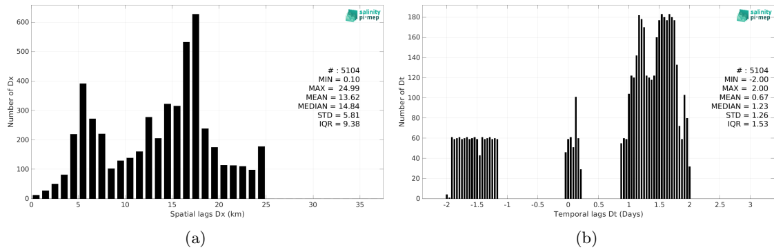
Figure 5: Histograms of the spatial (a) and temporal (b) lags between the location/time of the TSG (LEGOS-Surv-Adel) measurement and the date of the corresponding SMOS SSS L3 v8 - 9 Days (CATDS-CEC-LOCEAN) SSS pixel.
