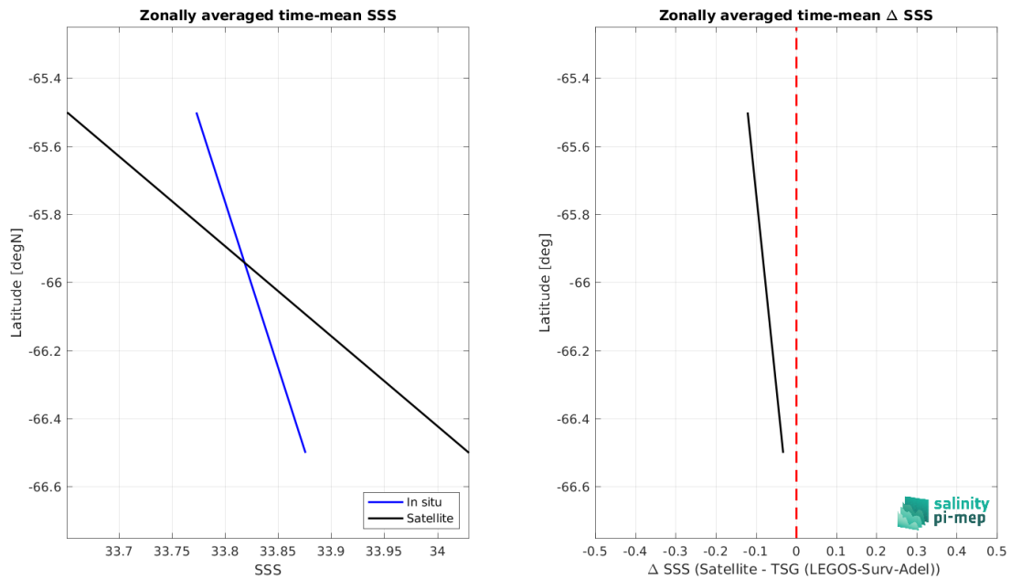
Figure 8: Left panel: Zonal mean SSS from SMOS SSS L3 v8 - 9 Days (CATDS-CEC-LOCEAN) satellite product (black) and from TSG (LEGOS-Surv-Adel) (blue). Right panel: Zonal mean of \Delta SSS (Satellite - TSG (LEGOS-Surv-Adel)) for all the collected Pi-MEP match-up pairs estimated over the full satellite product period.
