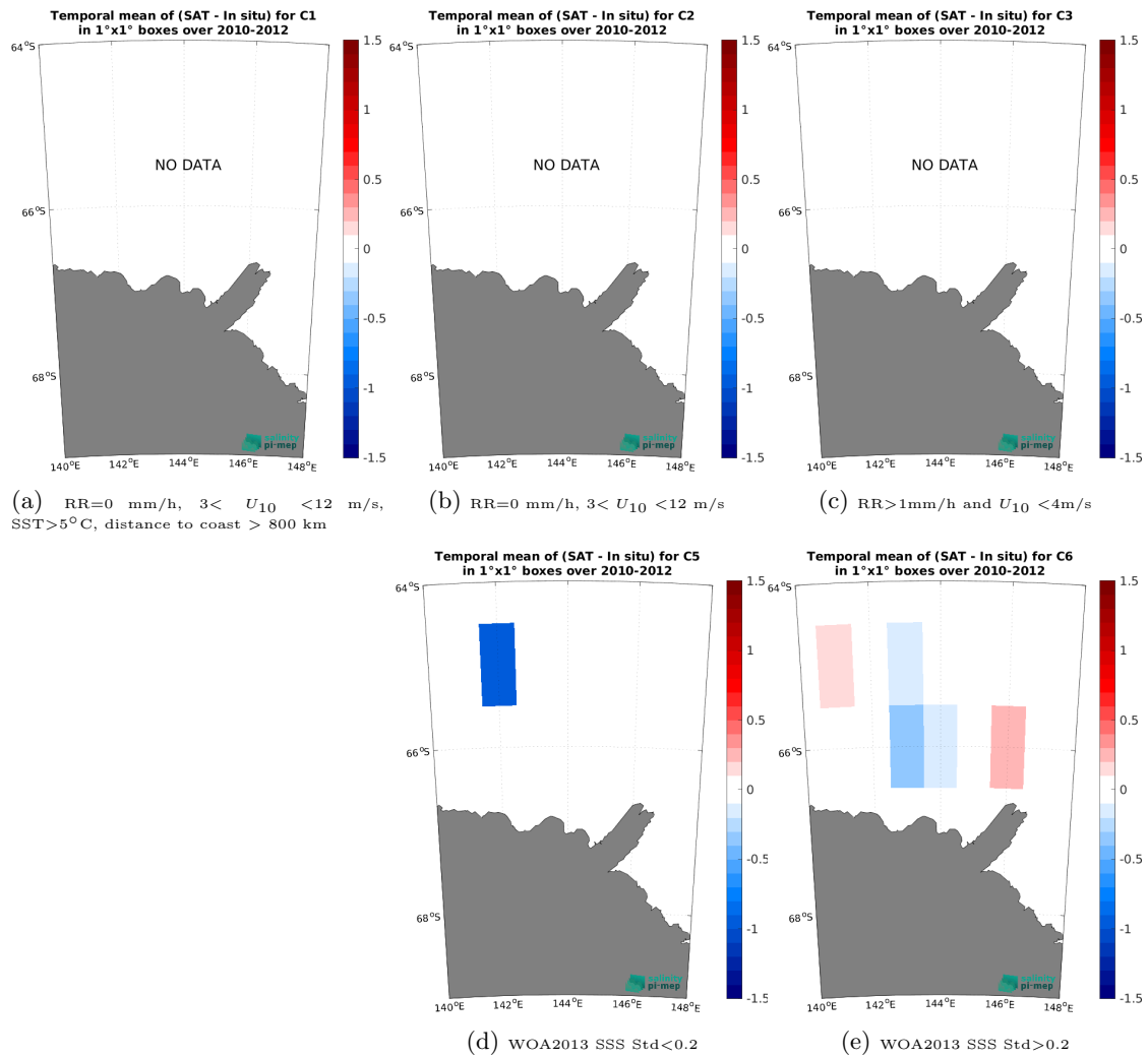
Figure 12: Temporal mean gridded over spatial boxes of size 1^\circ \times 1^\circ of \Delta SSS (SMOS SSS L3 v8 - 9 Days (CATDS-CEC-LOCEAN) - TSG (LEGOS-Surv-Adel)) for 5 different subdatasets corresponding to: RR=0 mm/h, 3 < U_{10} < 12 m/s, SST>5°C, distance to coast > 800 km (a), RR=0 mm/h, 3 < U_{10} < 12 m/s (b), RR>1mm/h and U_{10} < 4 m/s (c), WOA2013 SSS Std<0.2 (d), WOA2013 SSS Std>0.2 (e).
