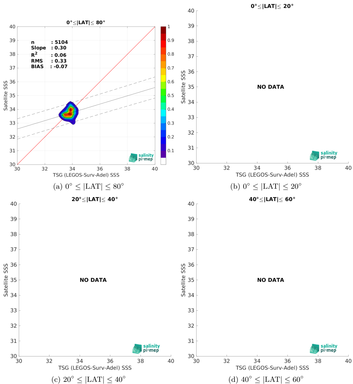
Figure 9: Contour maps of the concentration of SMOS SSS L3 v8 - 9 Days (CATDS-CEC-LOCEAN) SSS (y-axis) versus TSG (LEGOS-Surv-Adel) SSS (x-axis) at match-up pairs for different latitude bands. For each plot, the red line shows x=y . The black thin and dashed lines indicate a linear fit through the data cloud and the \pm 95\% confidence levels, respectively. The number match-up pairs n , the slope and R^2 coefficient of the linear fit, the root mean square (RMS) and the mean bias between satellite and in situ data are indicated for each latitude band in each plots.
