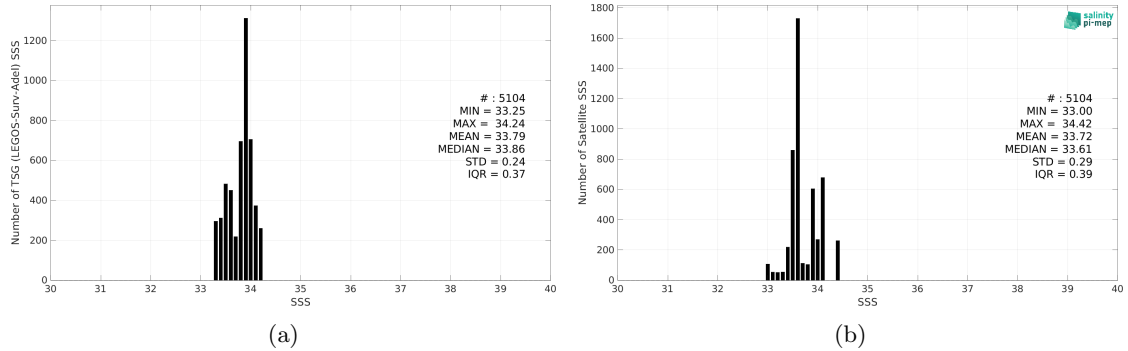
Figure 2: Histograms of SSS from TSG (LEGOS-Surv-Adel) (a) and SMOS SSS L3 v8 - 9 Days (CATDS-CEC-LOCEAN) (b) considering all match-up pairs per bins of 0.1 over the Global Ocean Pi-MEP region and for the full satellite product period.
