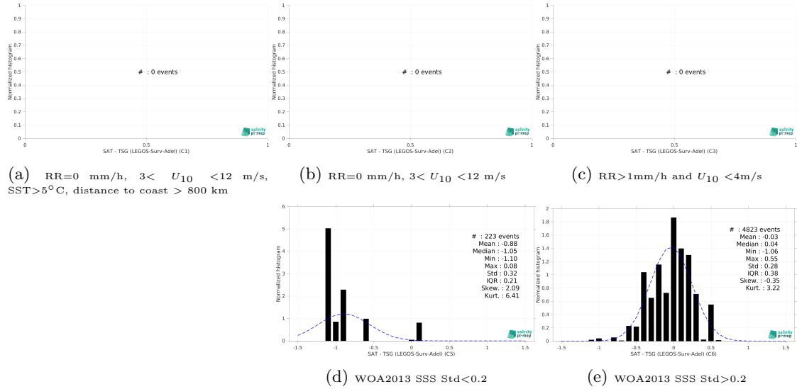
Figure 13: Normalized histogram of \Delta SSS (SMOS SSS L3 v8 - 9 Days (CATDS-CEC-LOCEAN) - TSG (LEGOS-Surv-Adel)) for 5 different subdatasets corresponding to: RR=0 mm/h, 3 < U_{10} < 12 m/s, SST>5°C, distance to coast > 800 km (a), RR=0 mm/h, 3 < U_{10} < 12 m/s (b), RR>1mm/h and U_{10} < 4 m/s (c), WOA2013 SSS Std<0.2 (d), WOA2013 SSS Std>0.2 (e).
