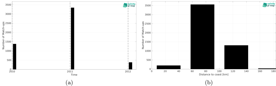
Figure 1: Number of match-ups between TSG (LEGOS-Surv-Adel) and SMOS SSS L3 v8 - 9 Days (CATDS-CEC-LOCEAN) SSS as a function of time (a) and as function of the distance to coast (b) over the Global Ocean Pi-MEP region and for the full satellite product period.
