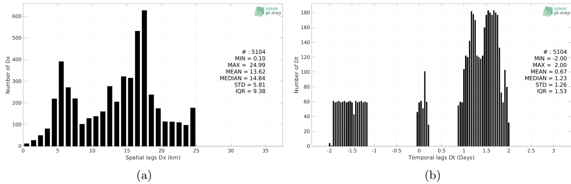
Figure 5: Histograms of the spatial (a) and temporal (b) lags between the location/time of the TSG (LEGOS-Surv-Adel) measurement and the date of the corresponding SMOS SSS L3 v8 - 9 Days (CATDS-CECOS-LOCEAN) SSS pixel.
