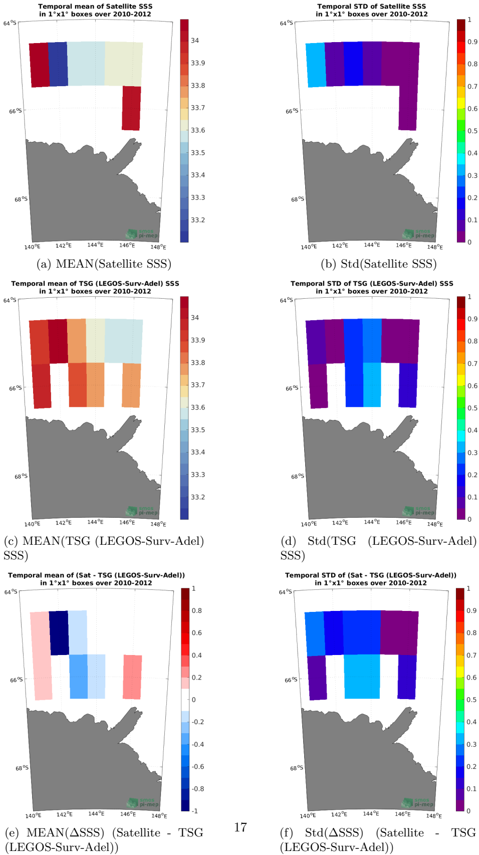
Figure 6: Temporal mean (left) and Std (right) of SSS from SMOS SSS L3 v8 - 9 Days (CATDS-CECOS-LOCEAN) (top), TSG (LEGOS-Surv-Adel) (middle), and of \Delta SSS (Satellite - TSG (LEGOS-Surv-Adel)). Only match-up pairs are used to generate these maps.
