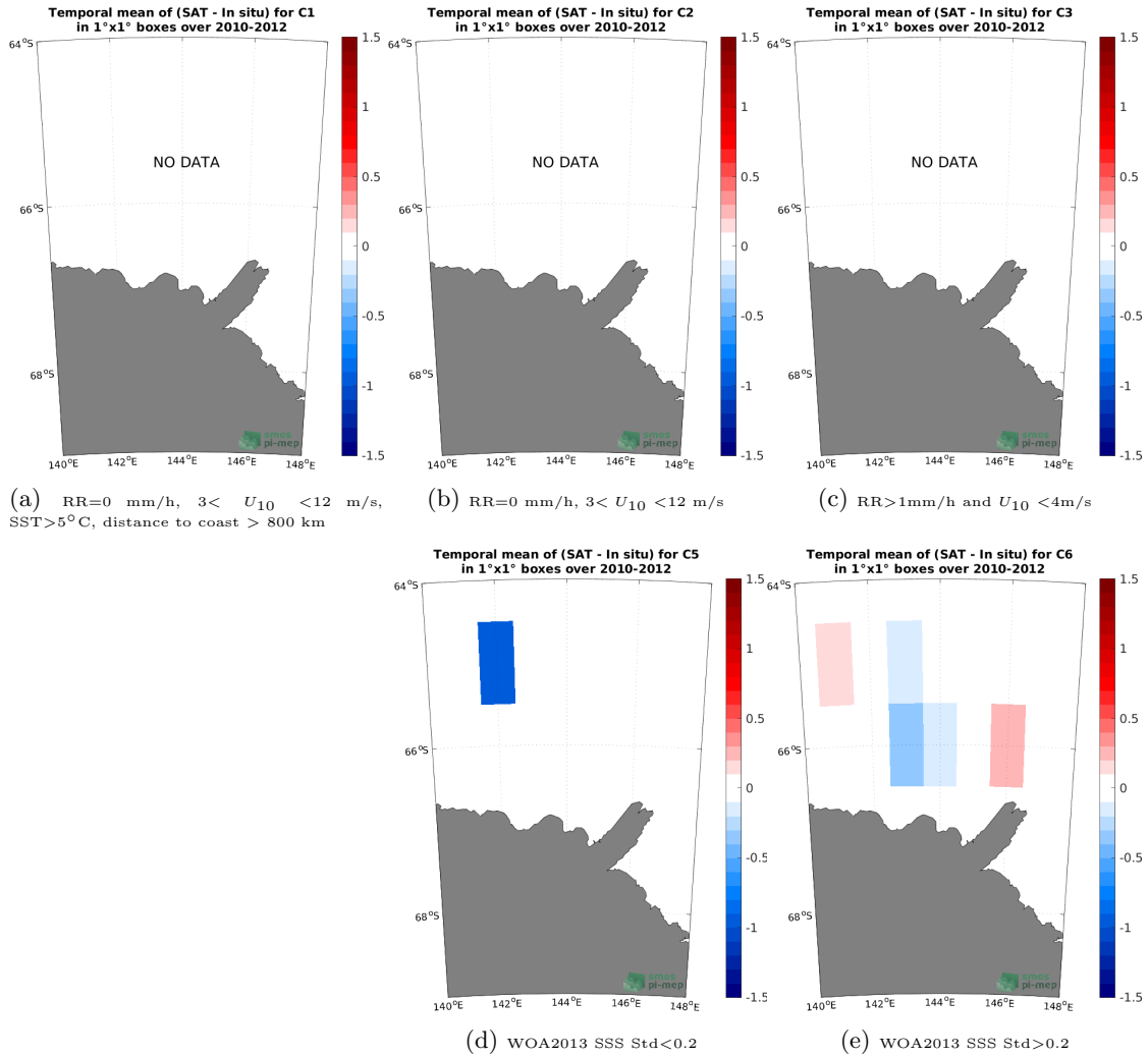
Figure 12: Temporal mean gridded over spatial boxes of size 1^\circ \times 1^\circ of \Delta SSS (SMOS SSS L3 v8 - 9 Days (CATDS-CECOS-LOCEAN) - TSG (LEGOS-Surv-Adel)) for 5 different subdatasets corresponding to:RR=0 mm/h, 3 < U_{10} < 12 m/s, SST>5°C, distance to coast > 800 km (a), RR=0 mm/h, 3 < U_{10} < 12 m/s (b), RR>1mm/h and U_{10} < 4 m/s (c), WOA2013 SSS Std<0.2 (d), WOA2013 SSS Std>0.2 (e).
