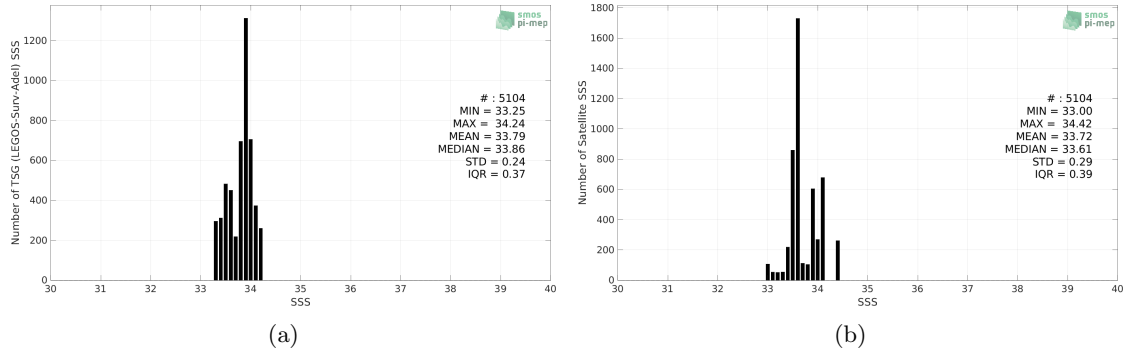
Figure 2: Histograms of SSS from TSG (LEGOS-Surv-Adel) (a) and SMOS SSS L3 v8 - 9 Days (CATDS-CECOS-LOCEAN) (b) considering all match-up pairs per bins of 0.1 over the Global Ocean Pi-MEP region and for the full satellite product period.
