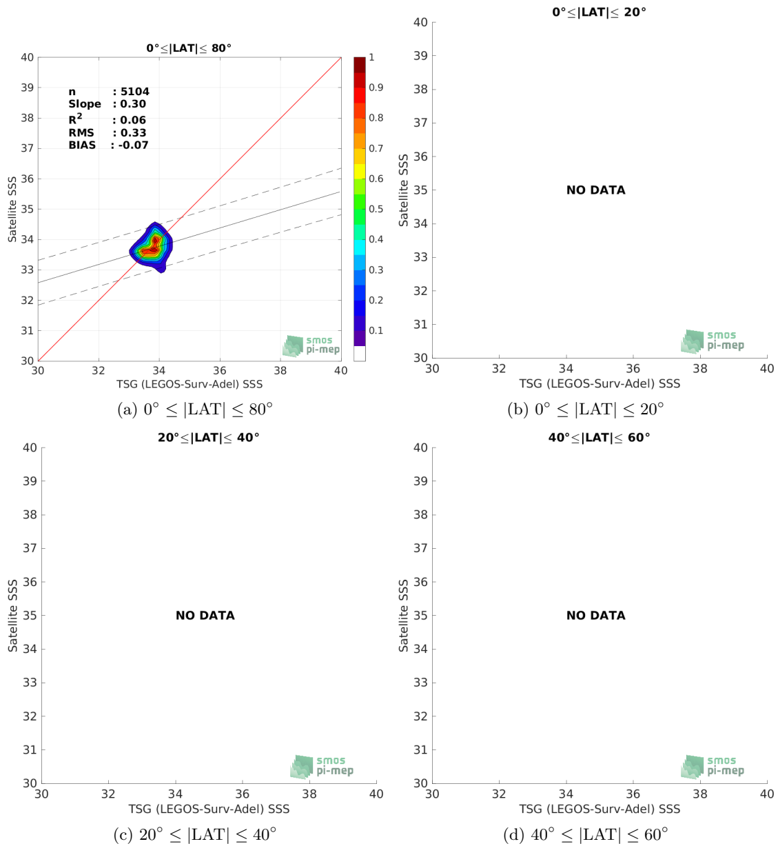
Figure 9: Contour maps of the concentration of SMOS SSS L3 v8 - 9 Days (CATDS-CECOS-LOCEAN) SSS (y-axis) versus TSG (LEGOS-Surv-Adel) SSS (x-axis) at match-up pairs for different latitude bands. For each plot, the red line shows x=y . The black thin and dashed lines indicate a linear fit through the data cloud and the \pm 95\% confidence levels, respectively. The number match-up pairs n , the slope and R^2 coefficient of the linear fit, the root mean square (RMS) and the mean bias between satellite and in situ data are indicated for each latitude band in each plots.
