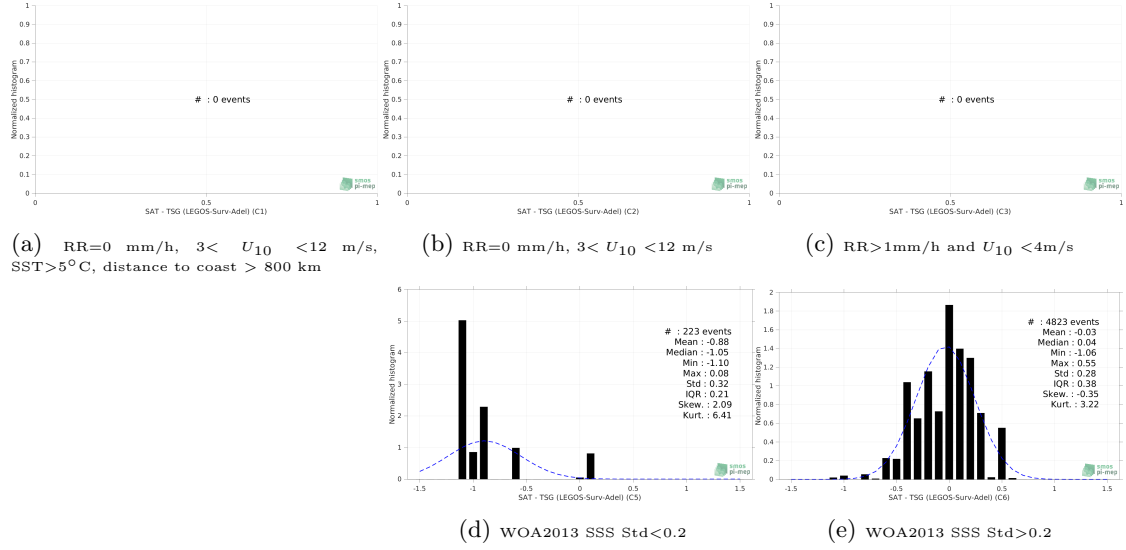
Figure 13: Normalized histogram of \Delta SSS (SMOS SSS L3 v8 - 9 Days (CATDS-CECOS-LOCEAN) - TSG (LEGOS-Surv-Adel)) for 5 different subdatasets corresponding to: RR=0 mm/h, 3 < U_{10} < 12 m/s, SST>5°C, distance to coast > 800 km (a), RR=0 mm/h, 3 < U_{10} < 12 m/s (b), RR>1mm/h and U_{10} < 4 m/s (c), WOA2013 SSS Std<0.2 (d), WOA2013 SSS Std>0.2 (e).
