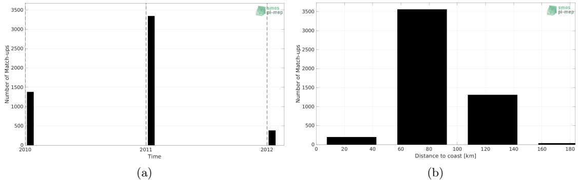
Figure 1: Number of match-ups between TSG (LEGOS-Surv-Adel) and SMOS SSS L3 v8 - 9 Days (CATDS-CECOS-LOCEAN) SSS as a function of time (a) and as function of the distance to coast (b) over the Global Ocean Pi-MEP region and for the full satellite product period.
