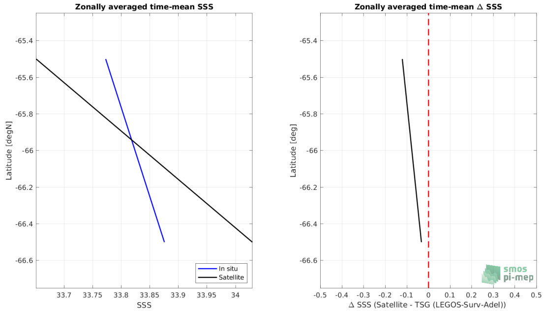
Figure 8: Left panel: Zonal mean SSS from SMOS SSS L3 v8 - 9 Days (CATDS-CECOS-LOCEAN) satellite product (black) and from TSG (LEGOS-Surv-Adel) (blue). Right panel: Zonal mean of \Delta SSS (Satellite - TSG (LEGOS-Surv-Adel)) for all the collected Pi-MEP match-up pairs estimated over the full satellite product period.
