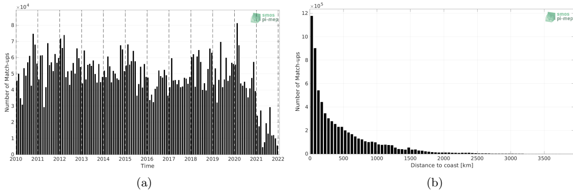
Figure 1: Number of match-ups between TSG (LEGOS-DM) and SMOS SSS L3 v8 - 9 Days (CATDS-CECOS-LOCEAN) SSS as a function of time (a) and as function of the distance to coast (b) over the Global Ocean Pi-MEP region and for the full satellite product period.
