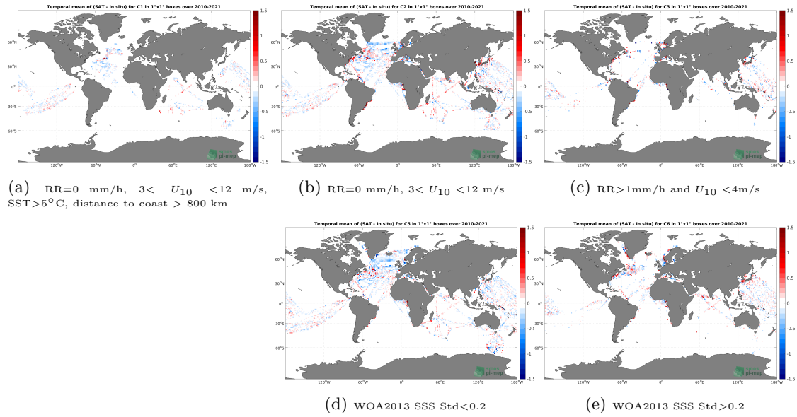
Figure 12: Temporal mean gridded over spatial boxes of size 1^\circ \times 1^\circ of \Delta SSS (SMOS SSS L3 v8 - 9 Days (CATDS-CECOS-LOCEAN) - TSG (LEGOS-DM)) for 5 different subdatasets corresponding to:RR=0 mm/h, 3 < U_{10} < 12 m/s, SST >5^\circ C, distance to coast > 800 km (a), RR=0 mm/h, 3 < U_{10} < 12 m/s (b), RR >1 mm/h and U_{10} < 4 m/s (c), WOA2013 SSS Std <0.2 (d), WOA2013 SSS Std >0.2 (e).
