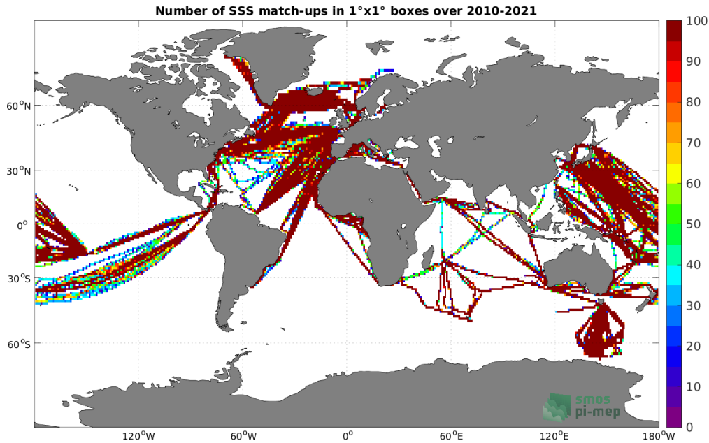
Figure 4: Number of SSS match-ups between TSG (LEGOS-DM) SSS and the SMOS SSS L3 v8 - 9 Days (CATDS-CECOS-LOCEAN) SSS product for the Global Ocean Pi-MEP region over 1^\circ \times 1^\circ boxes and for the full satellite product period.
