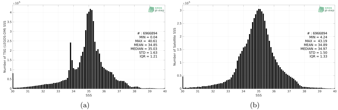
Figure 2: Histograms of SSS from TSG (LEGOS-DM) (a) and SMOS SSS L3 v8 - 9 Days (CATDS-CECOS-LOCEAN) (b) considering all match-up pairs per bins of 0.1 over the Global Ocean Pi-MEP region and for the full satellite product period.
