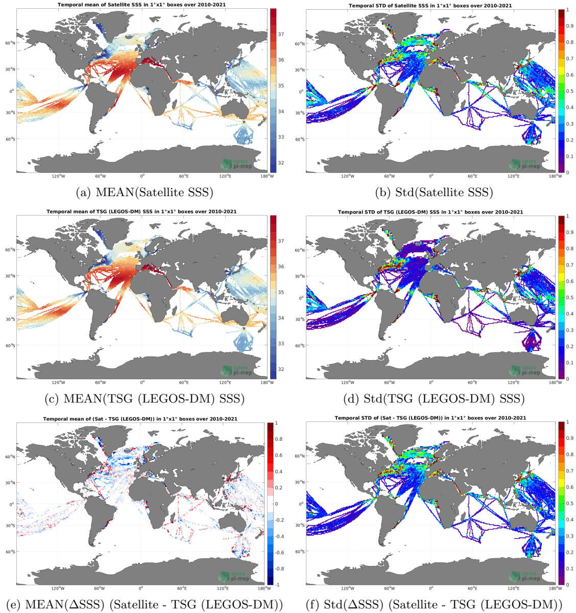
Figure 6: Temporal mean (left) and Std (right) of SSS from SMOS SSS L3 v8 - 9 Days (CATDS-CECOS-LOCEAN) (top), TSG (LEGOS-DM) (middle), and of \Delta SSS (Satellite - TSG (LEGOS-DM)). Only match-up pairs are used to generate these maps.
