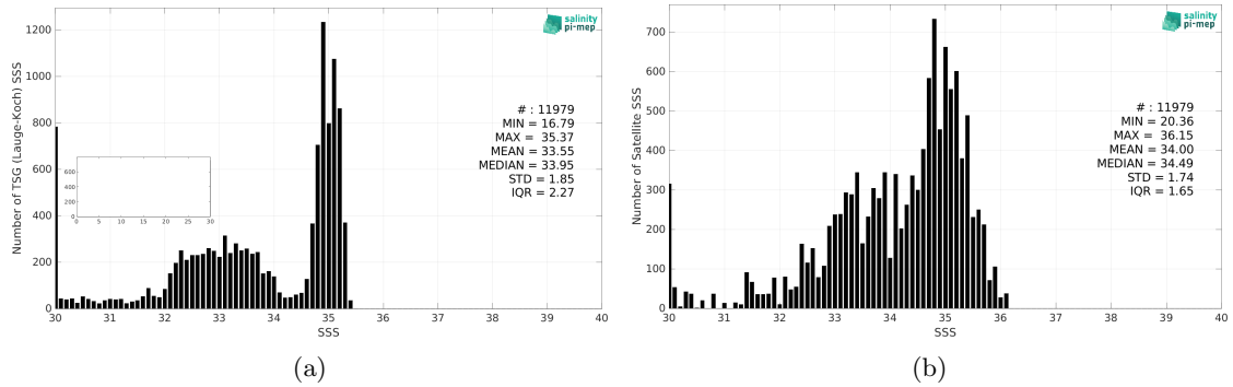
Figure 2: Histograms of SSS from TSG (Lauge-Koch) (a) and SMOS SSS L3 v8 - 9 Days (CATDS-CEC-LOCEAN) (b) considering all match-up pairs per bins of 0.1 over the Global Ocean Pi-MEP region and for the full satellite product period.
