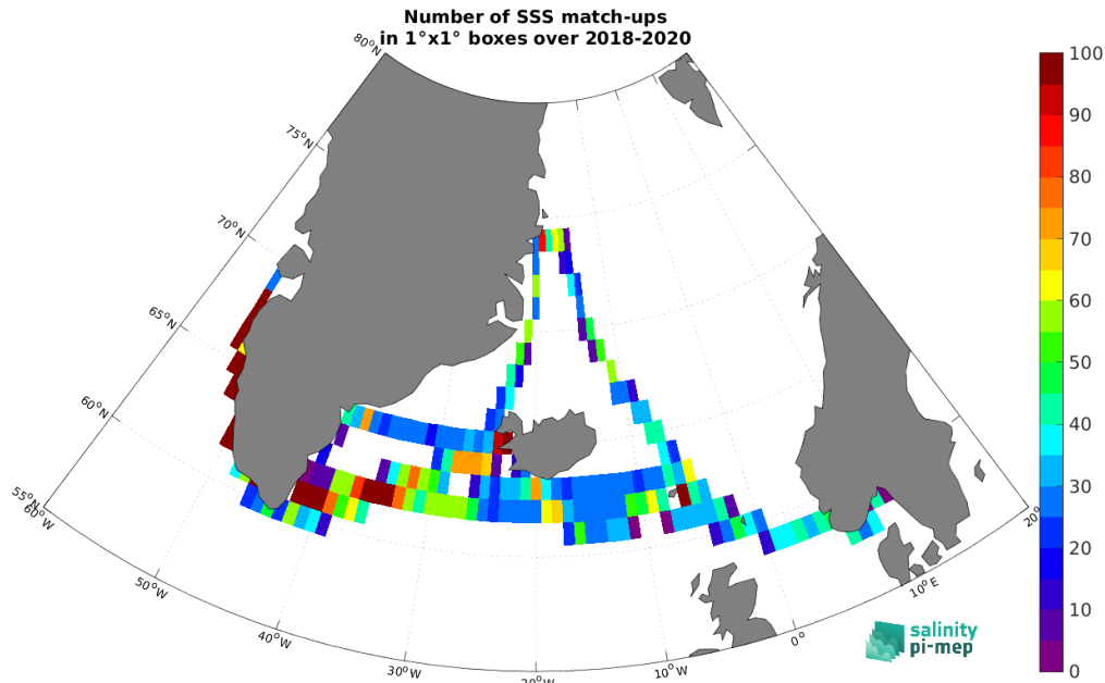
Figure 4: Number of SSS match-ups between TSG (Lauge-Koch) SSS and the SMOS SSS L3 v8 - 9 Days (CATDS-CEC-LOCEAN) SSS product for the Global Ocean Pi-MEP region over 1^\circ \times 1^\circ boxes and for the full satellite product period.
