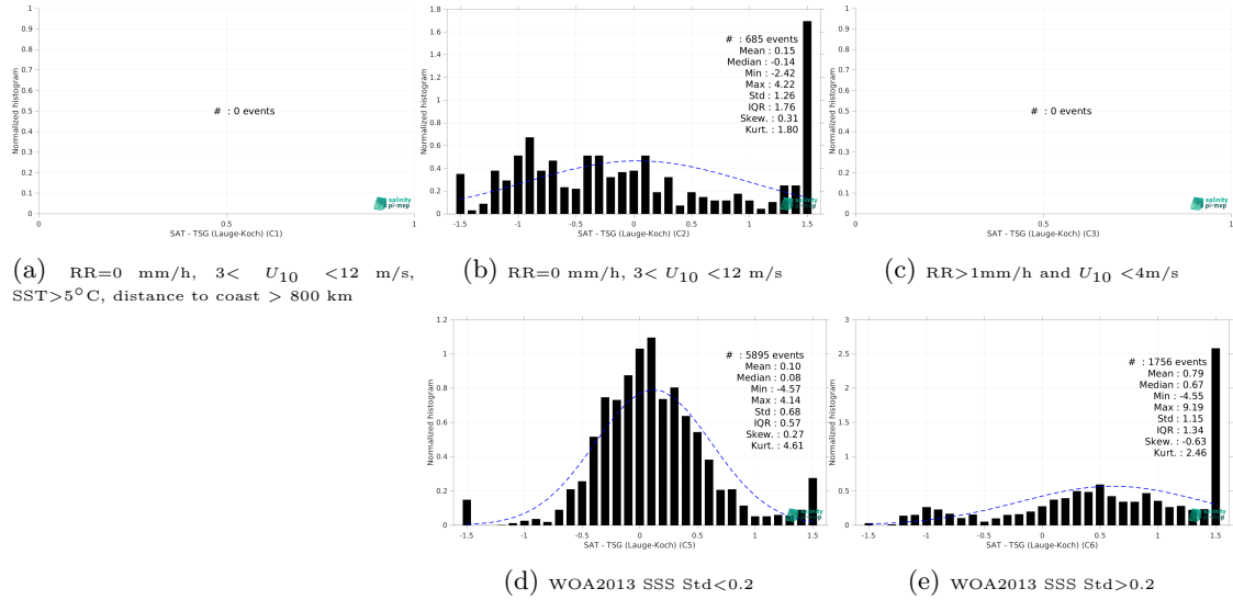
Figure 13: Normalized histogram of \Delta SSS (SMOS SSS L3 v8 - 9 Days (CATDS-CEC-LOCEAN) - TSG (Lauge-Koch)) for 5 different subdatasets corresponding to: RR=0 mm/h, 3 < U_{10} < 12 m/s, SST>5°C, distance to coast > 800 km (a), RR=0 mm/h, 3 < U_{10} < 12 m/s (b), RR>1mm/h and U_{10} < 4 m/s (c), WOA2013 SSS Std<0.2 (d), WOA2013 SSS Std>0.2 (e).
