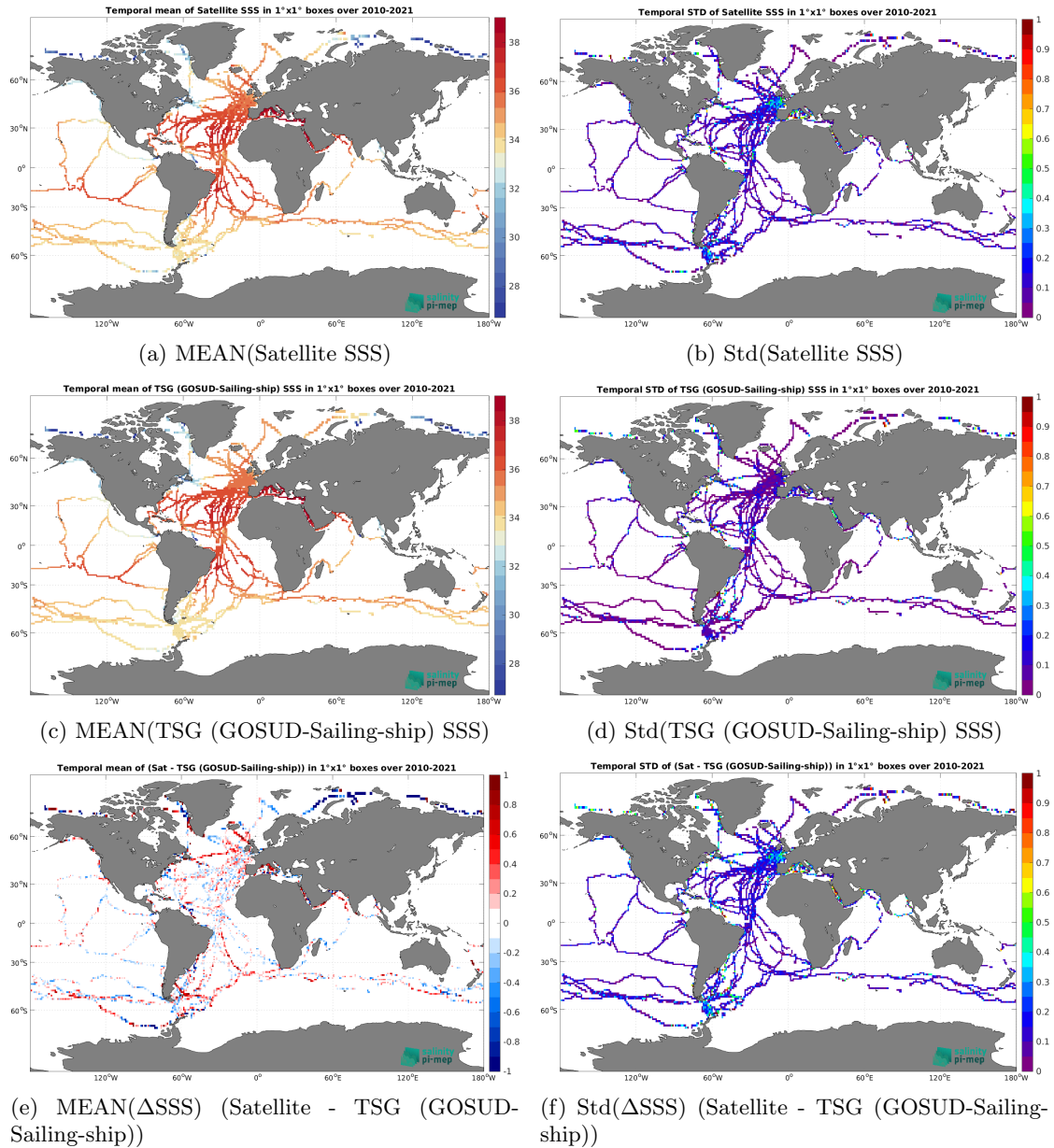
Figure 6: Temporal mean (left) and Std (right) of SSS from SMOS SSS L3 v8 - 9 Days (CATDS-CEC-LOCEAN) (top), TSG (GOSUD-Sailing-ship) (middle), and of \Delta SSS (Satellite - TSG (GOSUD-Sailing-ship)). Only match-up pairs are used to generate these maps.
