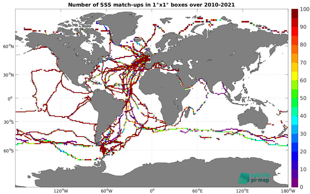
Figure 4: Number of SSS match-ups between TSG (GOSUD-Sailing-ship) SSS and the SMOS SSS L3 v8 - 9 Days (CATDS-CEC-LOCEAN) SSS product for the Global Ocean Pi-MEP region over 1^\circ \times 1^\circ boxes and for the full satellite product period.
