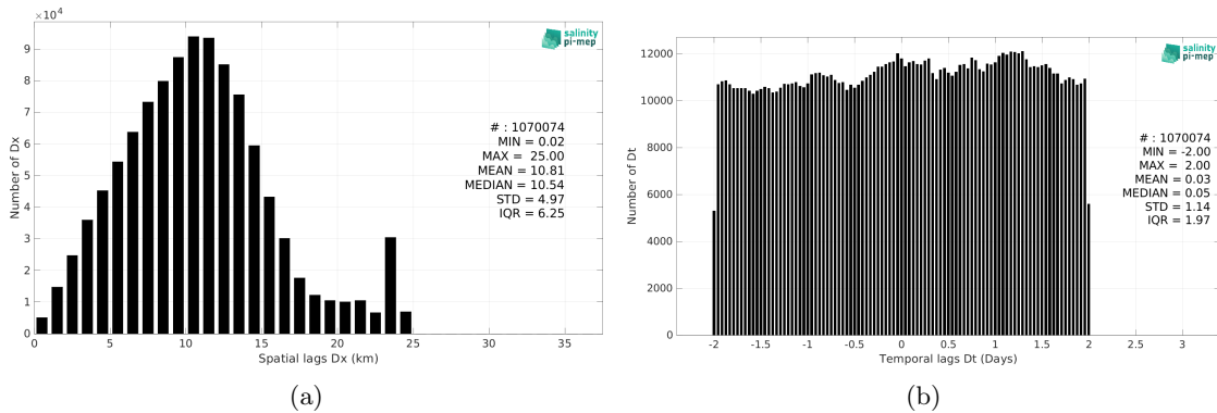
Figure 5: Histograms of the spatial (a) and temporal (b) lags between the location/time of the TSG (GOSUD-Sailing-ship) measurement and the date of the corresponding SMOS SSS L3 v8 - 9 Days (CATDS-CEC-LOCEAN) SSS pixel.
