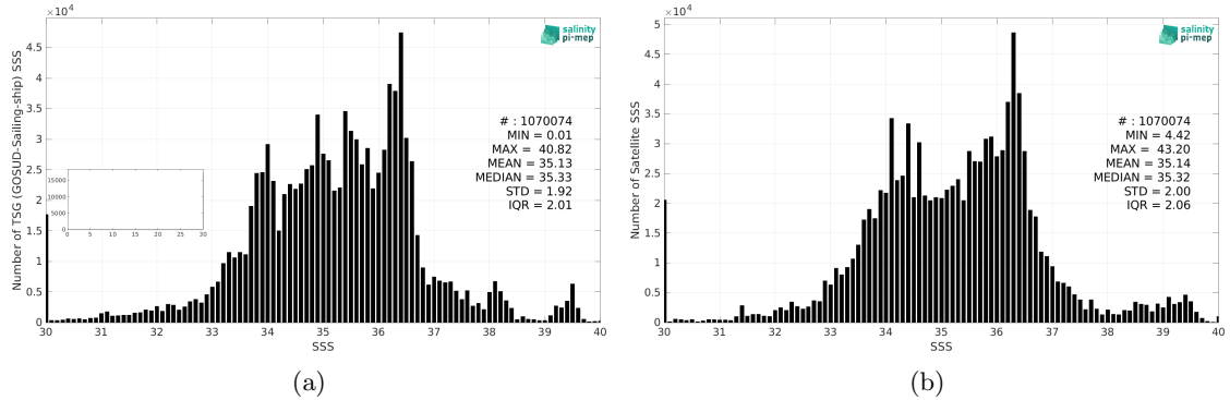
Figure 2: Histograms of SSS from TSG (GOSUD-Sailing-ship) (a) and SMOS SSS L3 v8 - 9 Days (CATDS-CEC-LOCEAN) (b) considering all match-up pairs per bins of 0.1 over the Global Ocean Pi-MEP region and for the full satellite product period.
