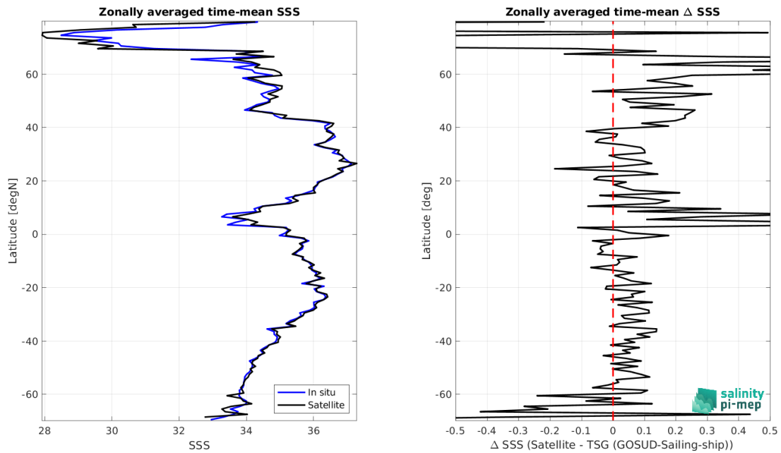
Figure 8: Left panel: Zonal mean SSS from SMOS SSS L3 v8 - 9 Days (CATDS-CEC-LOCEAN) satellite product (black) and from TSG (GOSUD-Sailing-ship) (blue). Right panel: Zonal mean of \Delta SSS (Satellite - TSG (GOSUD-Sailing-ship)) for all the collected Pi-MEP match-up pairs estimated over the full satellite product period.
