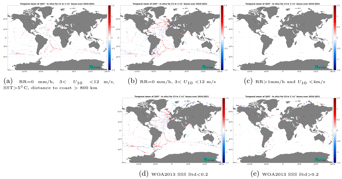
Figure 12: Temporal mean gridded over spatial boxes of size 1^\circ \times 1^\circ of \Delta SSS (SMOS SSS L3 v8 - 9 Days (CATDS-CEC-LOCEAN) - TSG (GOSUD-Sailing-ship)) for 5 different subdatasets corresponding to: RR=0 mm/h, 3 < U_{10} < 12 m/s, SST > 5°C, distance to coast > 800 km (a), RR=0 mm/h, 3 < U_{10} < 12 m/s (b), RR > 1mm/h and U_{10} < 4 m/s (c), WOA2013 SSS Std < 0.2 (d), WOA2013 SSS Std > 0.2 (e).
