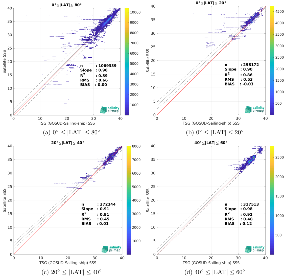
Figure 9: Contour maps of the concentration of SMOS SSS L3 v8 - 9 Days (CATDS-CEC-LOCEAN) SSS (y-axis) versus TSG (GOSUD-Sailing-ship) SSS (x-axis) at match-up pairs for different latitude bands. For each plot, the red line shows x=y . The black thin and dashed lines indicate a linear fit through the data cloud and the \pm 95\% confidence levels, respectively. The number match-up pairs n , the slope and R^2 coefficient of the linear fit, the root mean square (RMS) and the mean bias between satellite and in situ data are indicated for each latitude band in each plots.
