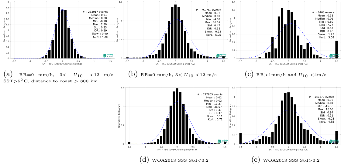
Figure 13: Normalized histogram of \Delta SSS (SMOS SSS L3 v8 - 9 Days (CATDS-CEC-LOCEAN) - TSG (GOSUD-Sailing-ship)) for 5 different subdatasets corresponding to: RR=0 mm/h, 3 < U_{10} < 12 m/s, SST > 5°C, distance to coast > 800 km (a), RR=0 mm/h, 3 < U_{10} < 12 m/s (b), RR > 1mm/h and U_{10} < 4 m/s (c), WOA2013 SSS Std < 0.2 (d), WOA2013 SSS Std > 0.2 (e).
