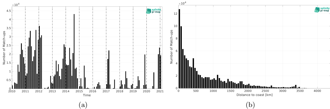
Figure 1: Number of match-ups between TSG (GOSUD-Sailing-ship) and SMOS SSS L3 v8 - 9 Days (CATDS-CEC-LOCEAN) SSS as a function of time (a) and as function of the distance to coast (b) over the Global Ocean Pi-MEP region and for the full satellite product period.
