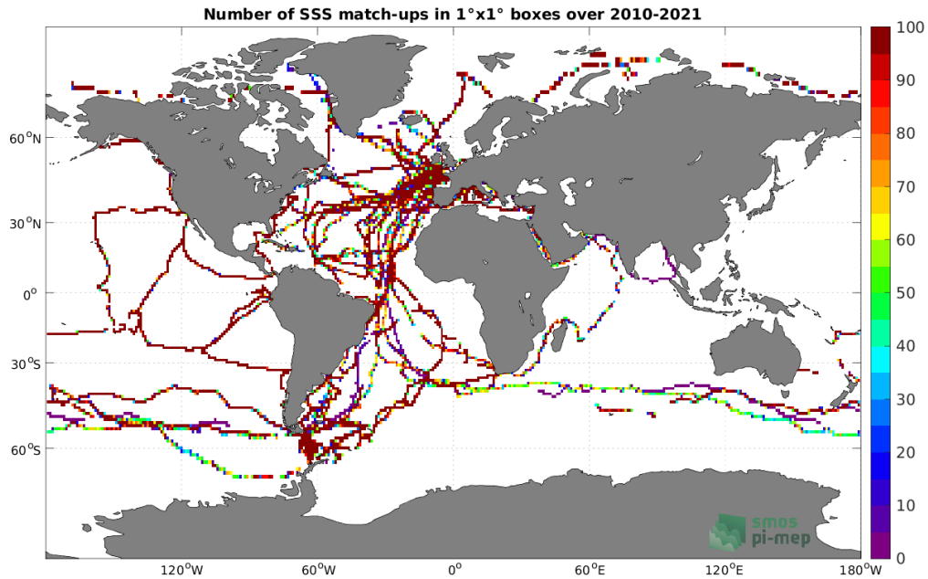
Figure 4: Number of SSS match-ups between TSG (GOSUD-Sailing-ship) SSS and the SMOS SSS L3 v8 - 9 Days (CATDS-CECOS-LOCEAN) SSS product for the Global Ocean Pi-MEP region over 1^\circ \times 1^\circ boxes and for the full satellite product period.
