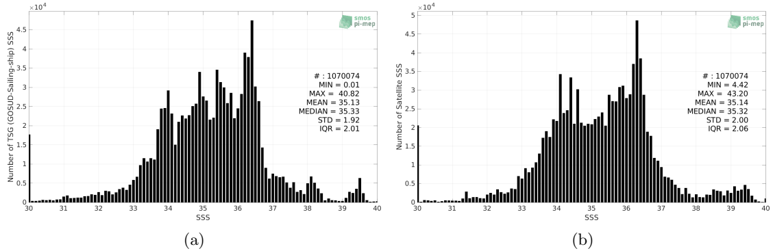
Figure 2: Histograms of SSS from TSG (GOSUD-Sailing-ship) (a) and SMOS SSS L3 v8 - 9 Days (CATDS-CECOS-LOCEAN) (b) considering all match-up pairs per bins of 0.1 over the Global Ocean Pi-MEP region and for the full satellite product period.
