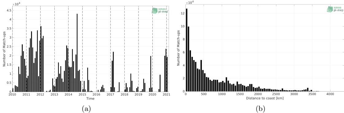
Figure 1: Number of match-ups between TSG (GOSUD-Sailing-ship) and SMOS SSS L3 v8 - 9 Days (CATDS-CECOS-LOCEAN) SSS as a function of time (a) and as function of the distance to coast (b) over the Global Ocean Pi-MEP region and for the full satellite product period.
