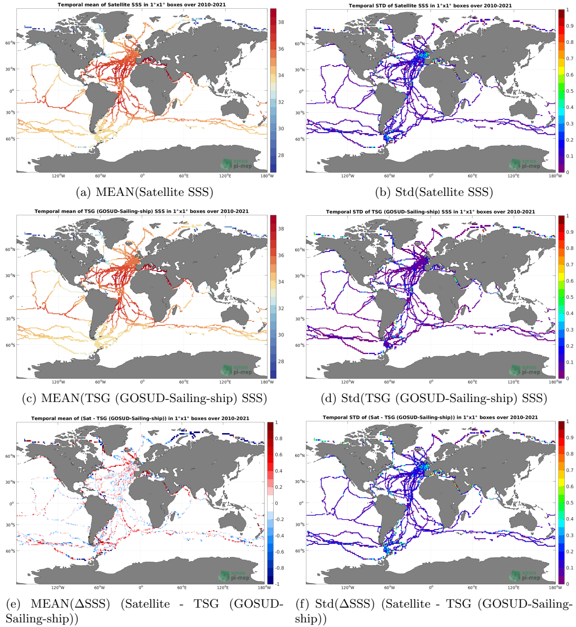
Figure 6: Temporal mean (left) and Std (right) of SSS from SMOS SSS L3 v8 - 9 Days (CATDS-CECOS-LOCEAN) (top), TSG (GOSUD-Sailing-ship) (middle), and of \Delta SSS (Satellite - TSG (GOSUD-Sailing-ship)). Only match-up pairs are used to generate these maps.
