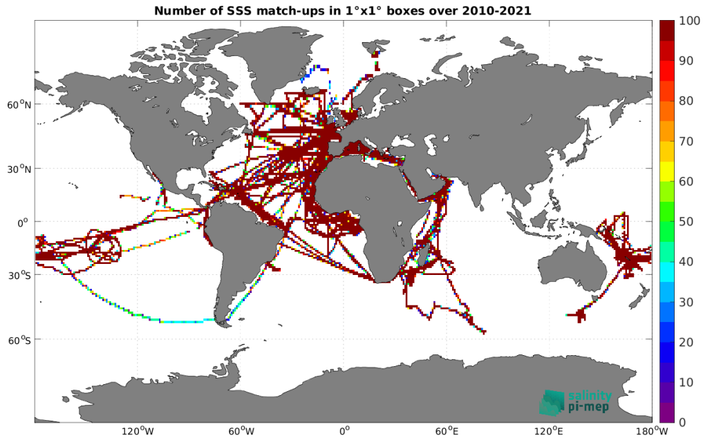
Figure 4: Number of SSS match-ups between TSG (GOSUD-Research-vessel) SSS and the SMOS SSS L3 v8 - 9 Days (CATDS-CEC-LOCEAN) SSS product for the Global Ocean Pi-MEP region over 1^\circ \times 1^\circ boxes and for the full satellite product period.
