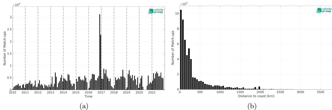
Figure 1: Number of match-ups between TSG (GOSUD-Research-vessel) and SMOS SSS L3 v8 - 9 Days (CATDS-CEC-LOCEAN) SSS as a function of time (a) and as function of the distance to coast (b) over the Global Ocean Pi-MEP region and for the full satellite product period.
