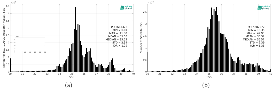
Figure 2: Histograms of SSS from TSG (GOSUD-Research-vessel) (a) and SMOS SSS L3 v8 - 9 Days (CATDS-CEC-LOCEAN) (b) considering all match-up pairs per bins of 0.1 over the Global Ocean Pi-MEP region and for the full satellite product period.
