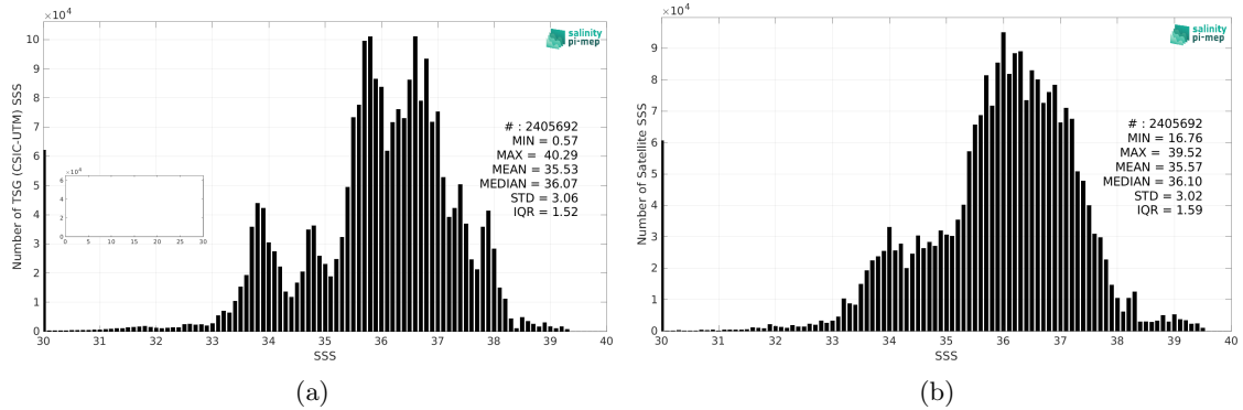
Figure 2: Histograms of SSS from TSG (CSIC-UTM) (a) and SMOS SSS L3 v8 - 9 Days (CATDS-CEC-LOCEAN) (b) considering all match-up pairs per bins of 0.1 over the Global Ocean Pi-MEP region and for the full satellite product period.
