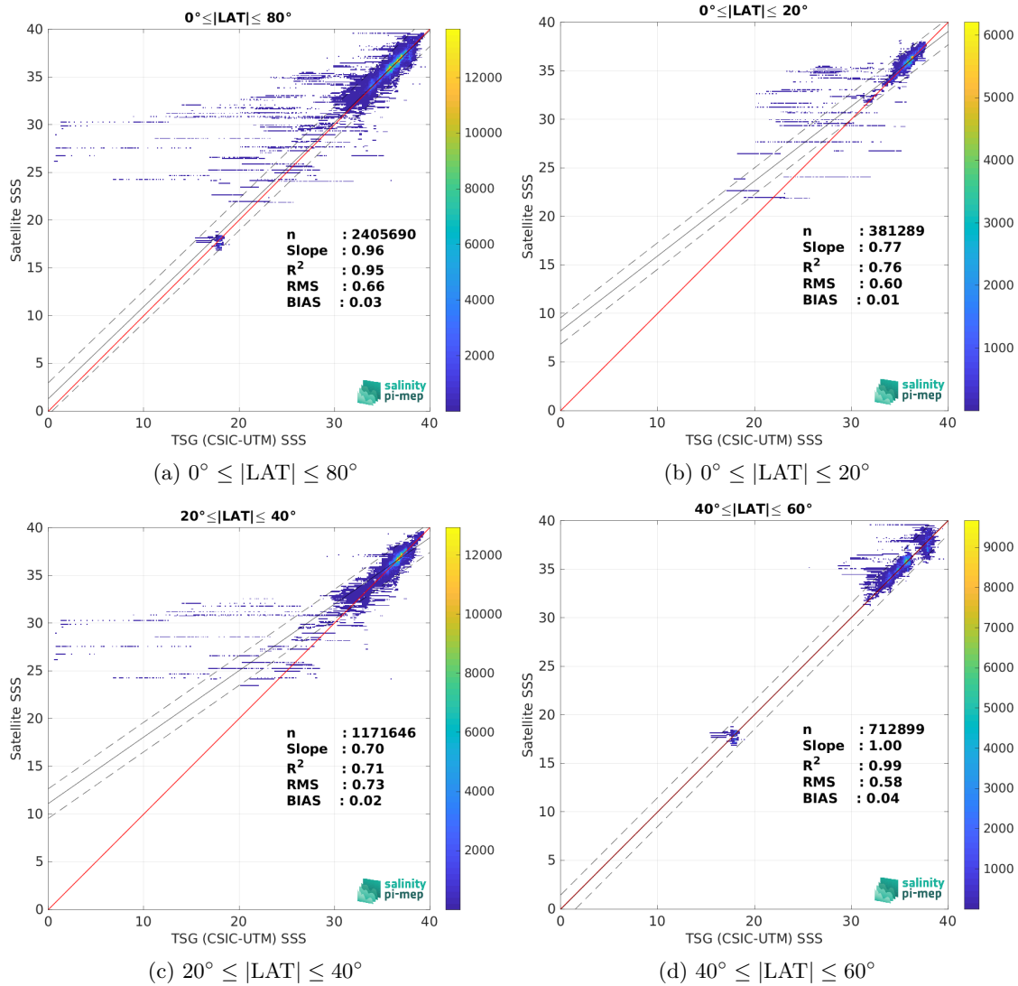
Figure 9: Contour maps of the concentration of SMOS SSS L3 v8 - 9 Days (CATDS-CEC-LOCEAN) SSS (y-axis) versus TSG (CSIC-UTM) SSS (x-axis) at match-up pairs for different latitude bands. For each plot, the red line shows x=y . The black thin and dashed lines indicate a linear fit through the data cloud and the \pm 95\% confidence levels, respectively. The number match-up pairs n , the slope and R^2 coefficient of the linear fit, the root mean square (RMS) and the mean bias between satellite and in situ data are indicated for each latitude band in each plots.
