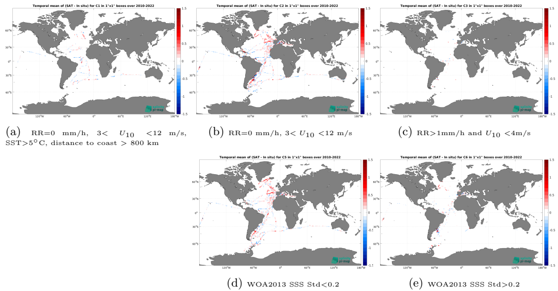
Figure 12: Temporal mean gridded over spatial boxes of size 1^\circ \times 1^\circ of \Delta SSS (SMOS SSS L3 v8 - 9 Days (CATDS-CEC-LOCEAN) - TSG (CSIC-UTM)) for 5 different subdatasets corresponding to:RR=0 mm/h, 3 < U_{10} < 12 m/s, SST >5^\circ C, distance to coast > 800 km (a), RR=0 mm/h, 3 < U_{10} < 12 m/s (b), RR >1 mm/h and U_{10} < 4 m/s (c), WOA2013 SSS Std <0.2 (d), WOA2013 SSS Std >0.2 (e).
