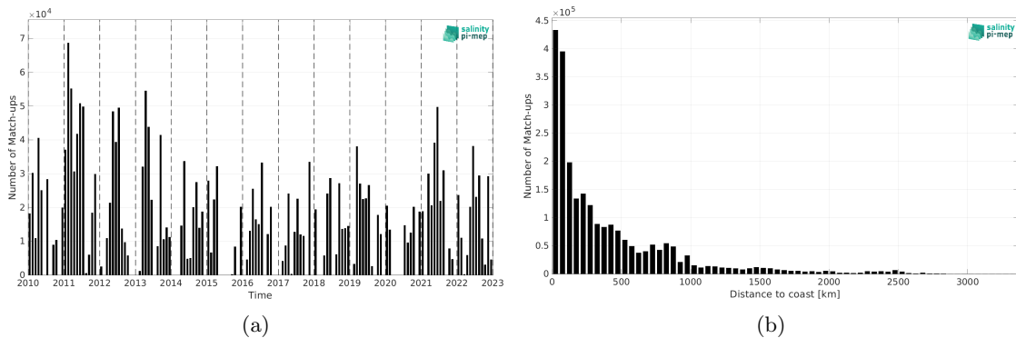
Figure 1: Number of match-ups between TSG (CSIC-UTM) and SMOS SSS L3 v8 - 9 Days (CATDS-CEC-LOCEAN) SSS as a function of time (a) and as function of the distance to coast (b) over the Global Ocean Pi-MEP region and for the full satellite product period.
