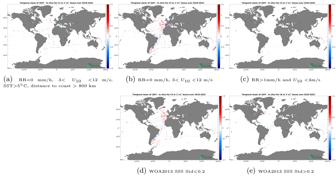
Figure 12: Temporal mean gridded over spatial boxes of size 1^\circ \times 1^\circ of \Delta SSS (SMOS SSS L3 v8 - 9 Days (CATDS-CECOS-LOCEAN) - TSG (CSIC-UTM)) for 5 different subdatasets corresponding to:RR=0 mm/h, 3 < U_{10} < 12 m/s, SST >5^\circ C, distance to coast > 800 km (a), RR=0 mm/h, 3 < U_{10} < 12 m/s (b), RR >1 mm/h and U_{10} < 4 m/s (c), WOA2013 SSS Std <0.2 (d), WOA2013 SSS Std >0.2 (e).
