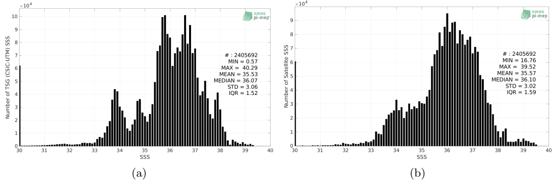
Figure 2: Histograms of SSS from TSG (CSIC-UTM) (a) and SMOS SSS L3 v8 - 9 Days (CATDS-CECOS-LOCEAN) (b) considering all match-up pairs per bins of 0.1 over the Global Ocean Pi-MEP region and for the full satellite product period.
