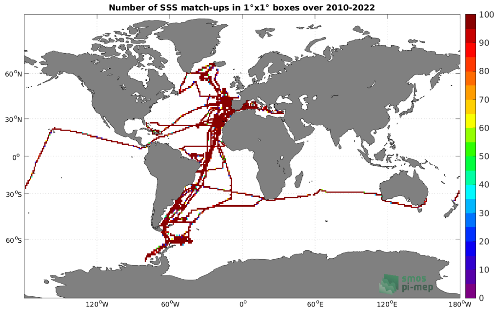
Figure 4: Number of SSS match-ups between TSG (CSIC-UTM) SSS and the SMOS SSS L3 v8 - 9 Days (CATDS-CECOS-LOCEAN) SSS product for the Global Ocean Pi-MEP region over 1^\circ \times 1^\circ boxes and for the full satellite product period.
