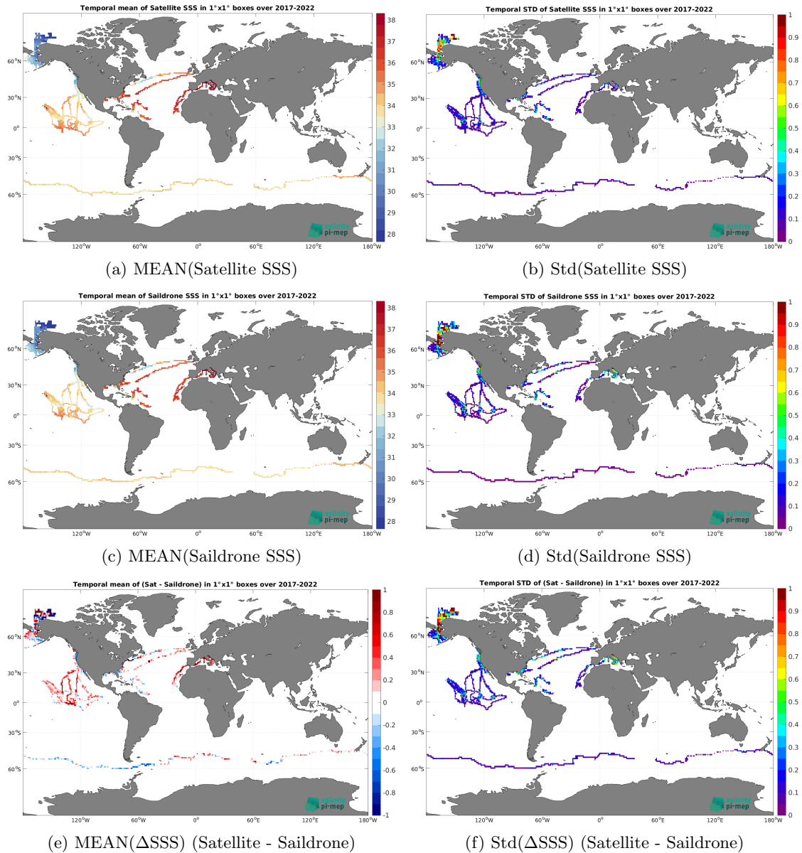
Figure 6: Temporal mean (left) and Std (right) of SSS from SMOS SSS L3 v8 - 9 Days (CATDS-CEC-LOCEAN) (top), Saildrone (middle), and of \Delta SSS (Satellite - Saildrone). Only match-up pairs are used to generate these maps.
