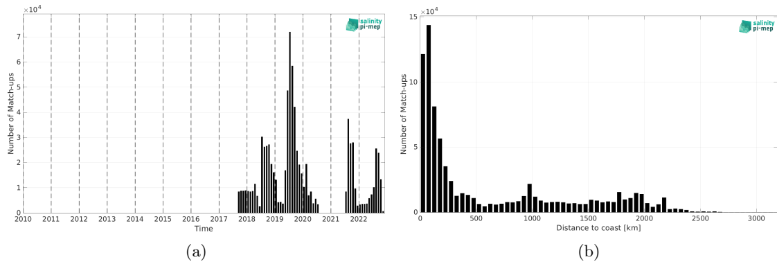
Figure 1: Number of match-ups between Saildrone and SMOS SSS L3 v8 - 9 Days (CATDS-CEC-LOCEAN) SSS as a function of time (a) and as function of the distance to coast (b) over the Global Ocean Pi-MEP region and for the full satellite product period.
