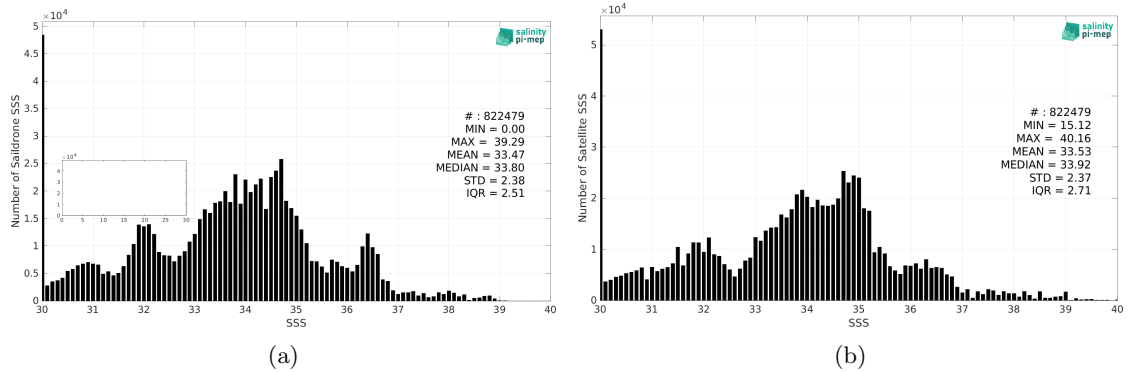
Figure 2: Histograms of SSS from Saildrone (a) and SMOS SSS L3 v8 - 9 Days (CATDS-CEC-LOCEAN) (b) considering all match-up pairs per bins of 0.1 over the Global Ocean Pi-MEP region and for the full satellite product period.
