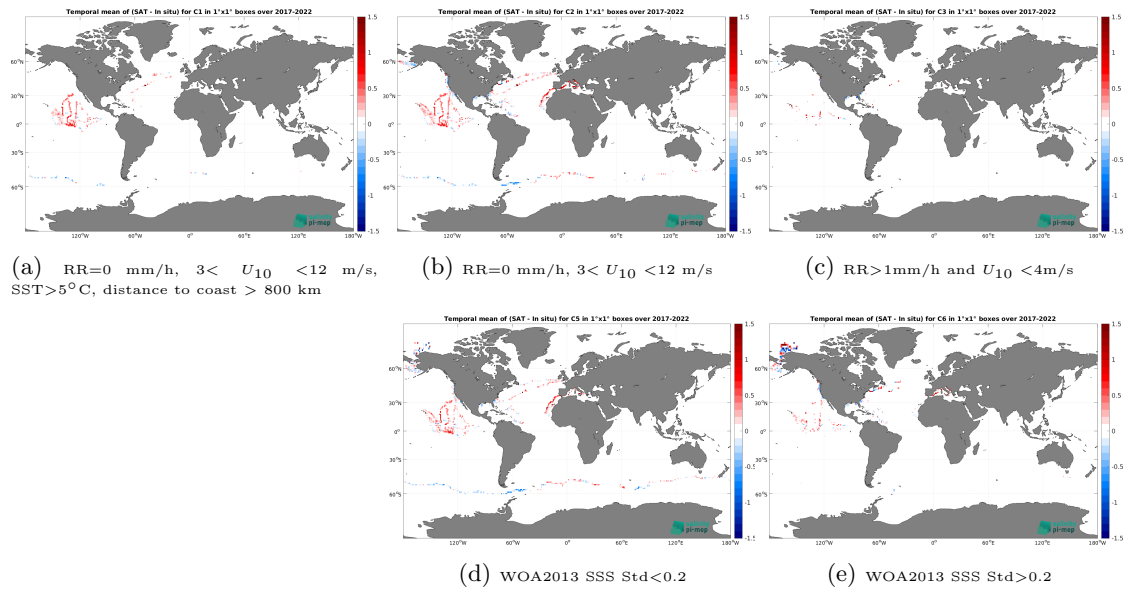
Figure 12: Temporal mean gridded over spatial boxes of size 1^\circ \times 1^\circ of \Delta SSS (SMOS SSS L3 v8 - 9 Days (CATDS-CEC-LOCEAN) - Saildrone) for 5 different subdatasets corresponding to:RR=0 mm/h, 3 < U_{10} < 12 m/s, SST > 5^\circ\text{C} , distance to coast > 800 km (a), RR=0 mm/h, 3 < U_{10} < 12 m/s (b), RR > 1 mm/h and U_{10} < 4 m/s (c), WOA2013 SSS Std < 0.2 (d), WOA2013 SSS Std > 0.2 (e).
