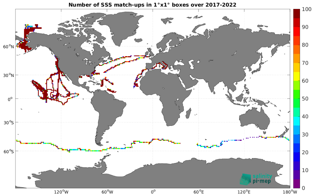
Figure 4: Number of SSS match-ups between Saildrone SSS and the SMOS SSS L3 v8 - 9 Days (CATDS-CEC-LOCEAN) SSS product for the Global Ocean Pi-MEP region over 1^\circ \times 1^\circ boxes and for the full satellite product period.
