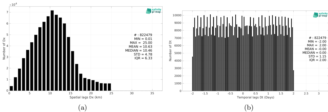
Figure 5: Histograms of the spatial (a) and temporal (b) lags between the location/time of the Saildrone measurement and the date of the corresponding SMOS SSS L3 v8 - 9 Days (CATDS-CEC-LOCEAN) SSS pixel.
