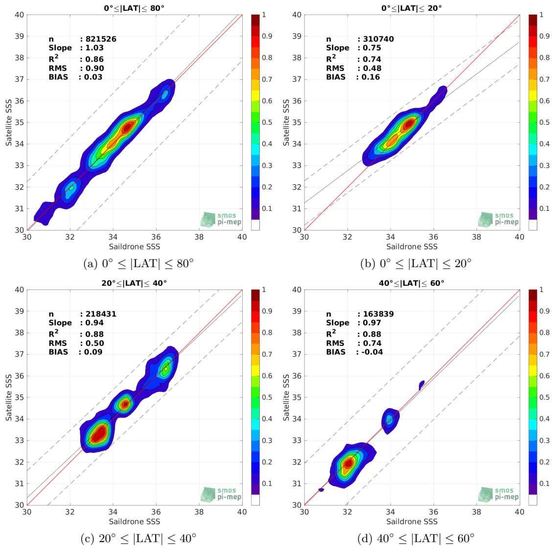
Figure 9: Contour maps of the concentration of SMOS SSS L3 v8 - 9 Days (CATDS-CECOS-LOCEAN) SSS (y-axis) versus Saildrone SSS (x-axis) at match-up pairs for different latitude bands. For each plot, the red line shows x=y . The black thin and dashed lines indicate a linear fit through the data cloud and the \pm 95\% confidence levels, respectively. The number match-up pairs n , the slope and R^2 coefficient of the linear fit, the root mean square (RMS) and the mean bias between satellite and in situ data are indicated for each latitude band in each plots.
