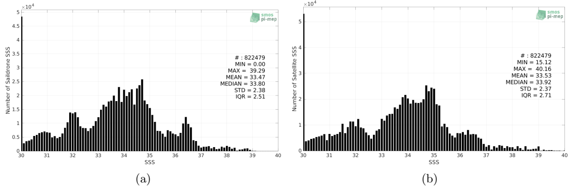
Figure 2: Histograms of SSS from Saildrone (a) and SMOS SSS L3 v8 - 9 Days (CATDS-CECOS-LOCEAN) (b) considering all match-up pairs per bins of 0.1 over the Global Ocean Pi-MEP region and for the full satellite product period.
