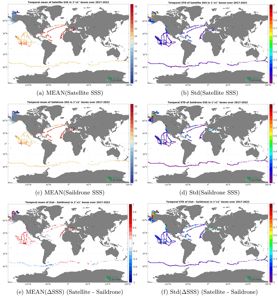
Figure 6: Temporal mean (left) and Std (right) of SSS from SMOS SSS L3 v8 - 9 Days (CATDS-CECOS-LOCEAN) (top), Saildrone (middle), and of \Delta SSS (Satellite - Saildrone). Only match-up pairs are used to generate these maps.
