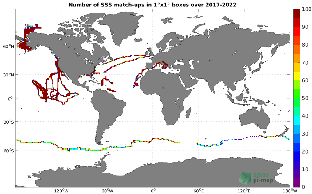
Figure 4: Number of SSS match-ups between Saildrone SSS and the SMOS SSS L3 v8 - 9 Days (CATDS-CECOS-LOCEAN) SSS product for the Global Ocean Pi-MEP region over 1^\circ \times 1^\circ boxes and for the full satellite product period.
