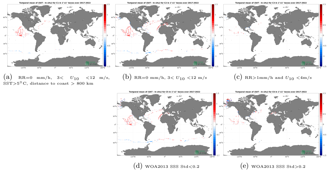
Figure 12: Temporal mean gridded over spatial boxes of size 1^\circ \times 1^\circ of \Delta SSS (SMOS SSS L3 v8 - 9 Days (CATDS-CECOS-LOCEAN) - Saildrone) for 5 different subdatasets corresponding to:RR=0 mm/h, 3 < U_{10} < 12 m/s, SST > 5^\circ\text{C} , distance to coast > 800 km (a), RR=0 mm/h, 3 < U_{10} < 12 m/s (b), RR > 1 mm/h and U_{10} < 4 m/s (c), WOA2013 SSS Std < 0.2 (d), WOA2013 SSS Std > 0.2 (e).
