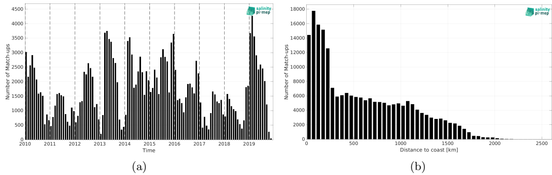
Figure 1: Number of match-ups between Marine mammals and SMOS SSS L3 v8 - 9 Days (CATDS-CEC-LOCEAN) SSS as a function of time (a) and as function of the distance to coast (b) over the Global Ocean Pi-MEP region and for the full satellite product period.
