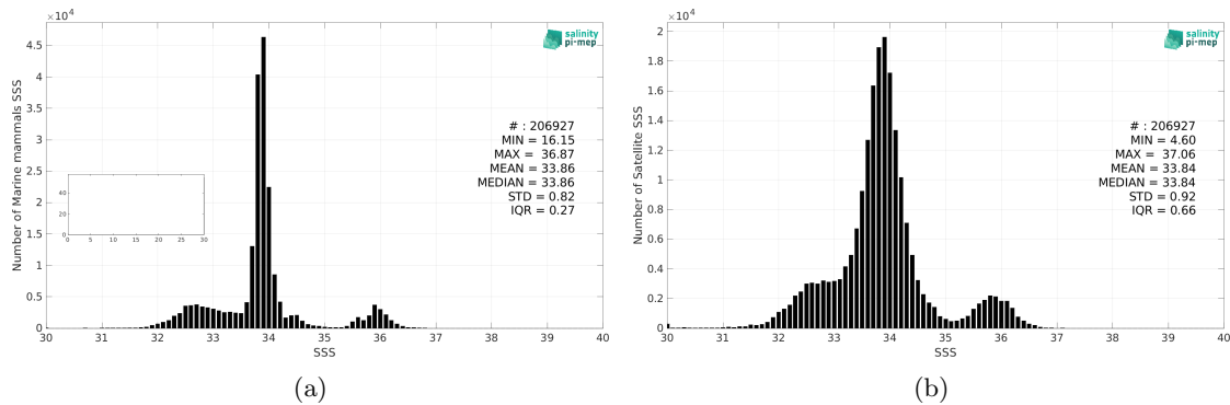
Figure 2: Histograms of SSS from Marine mammals (a) and SMOS SSS L3 v8 - 9 Days (CATDS-CEC-LOCEAN) (b) considering all match-up pairs per bins of 0.1 over the Global Ocean Pi-MEP region and for the full satellite product period.
