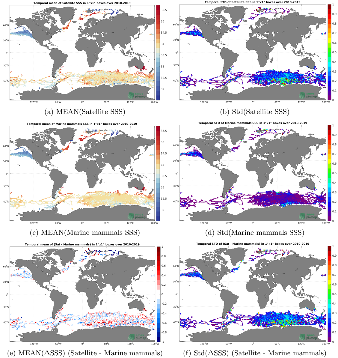
Figure 6: Temporal mean (left) and Std (right) of SSS from SMOS SSS L3 v8 - 9 Days (CATDS-CECOS-LOCEAN) (top), Marine mammals (middle), and of \Delta SSS (Satellite - Marine mammals). Only match-up pairs are used to generate these maps.
