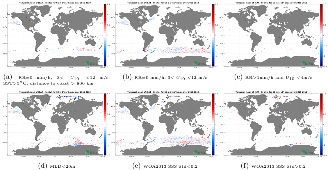
Figure 12: Temporal mean gridded over spatial boxes of size 1^{\circ}\times 1^{\circ} of \Delta\text{SSS} (SMOS SSS L3 v8 - 9 Days (CATDS-CECOS-LOCEAN) - Marine mammals) for 6 different subdatasets corresponding to:RR=0 mm/h, 3 < U_{10} < 12 m/s, SST >5^{\circ}\text{C} , distance to coast > 800 km (a), RR=0 mm/h, 3 < U_{10} < 12 m/s (b), RR >1\text{mm/h} and U_{10} < 4\text{m/s} (c),MLD <20\text{m} (d),WOA2013 SSS Std <0.2 (e),WOA2013 SSS Std >0.2 (f).
