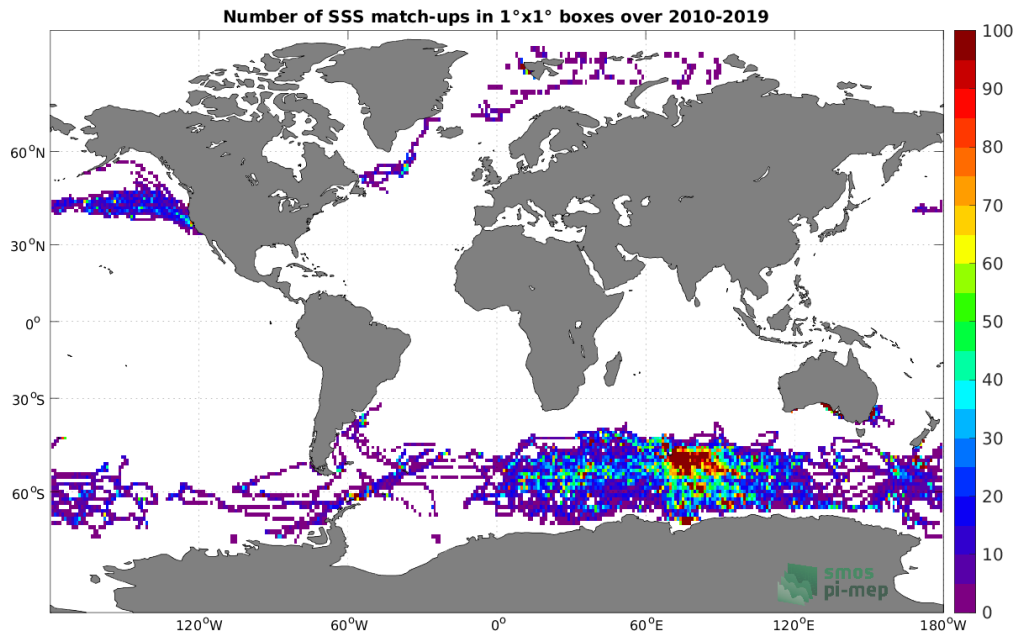
Figure 4: Number of SSS match-ups between Marine mammals SSS and the SMOS SSS L3 v8 - 9 Days (CATDS-CECOS-LOCEAN) SSS product for the Global Ocean Pi-MEP region over 1^\circ \times 1^\circ boxes and for the full satellite product period.
