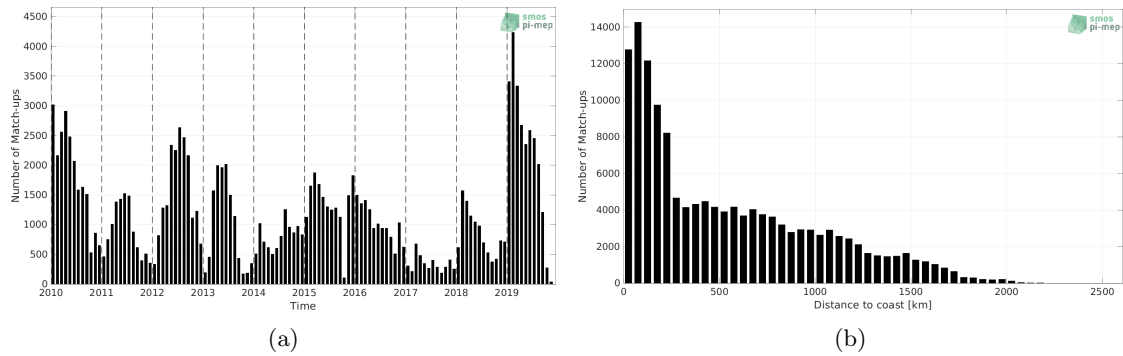
Figure 1: Number of match-ups between Marine mammals and SMOS SSS L3 v8 - 9 Days (CATDS-CECOS-LOCEAN) SSS as a function of time (a) and as function of the distance to coast (b) over the Global Ocean Pi-MEP region and for the full satellite product period.
