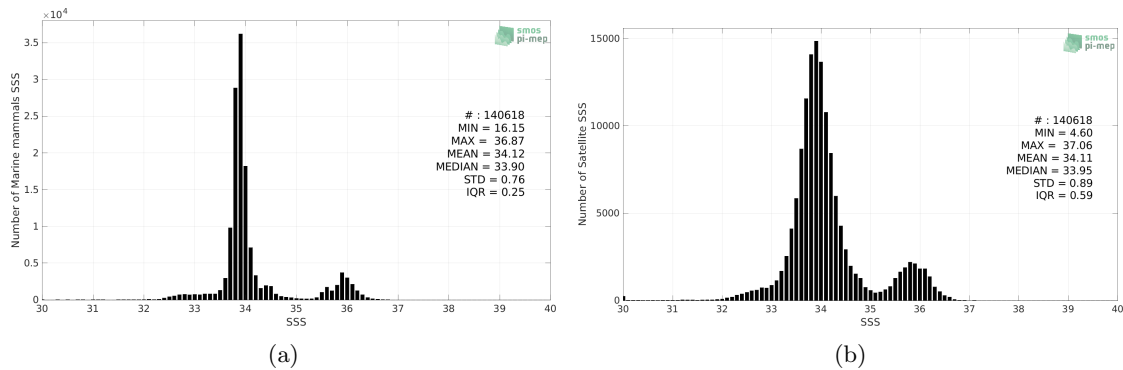
Figure 2: Histograms of SSS from Marine mammals (a) and SMOS SSS L3 v8 - 9 Days (CATDS-CECOS-LOCEAN) (b) considering all match-up pairs per bins of 0.1 over the Global Ocean Pi-MEP region and for the full satellite product period.
