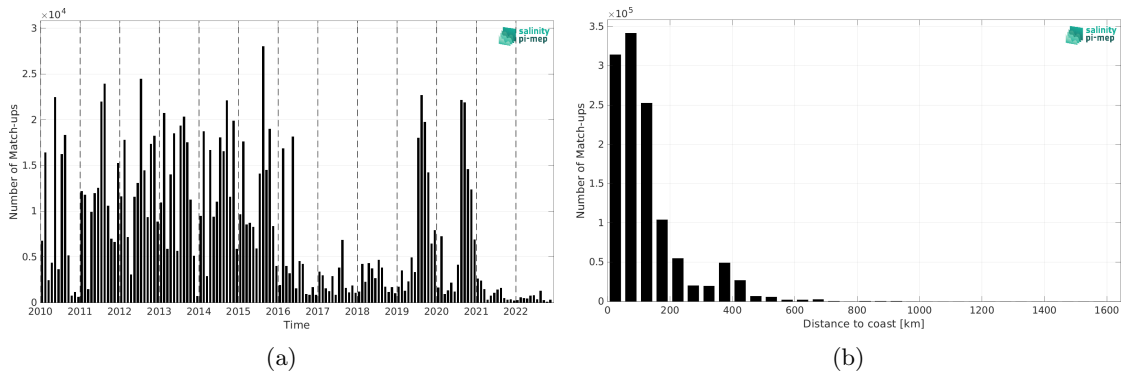
Figure 1: Number of match-ups between ICES and SMOS SSS L3 v8 - 9 Days (CATDS-CEC-LOCEAN) SSS as a function of time (a) and as function of the distance to coast (b) over the Global Ocean Pi-MEP region and for the full satellite product period.
