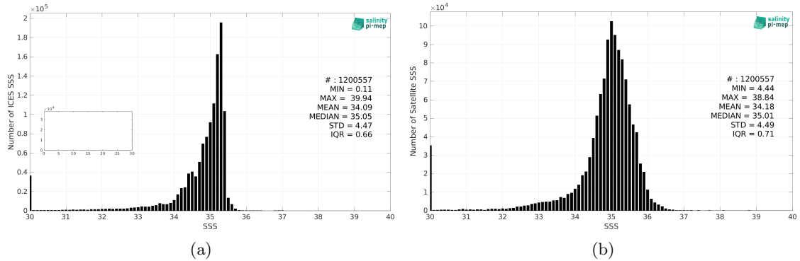
Figure 2: Histograms of SSS from ICES (a) and SMOS SSS L3 v8 - 9 Days (CATDS-CEC-LOCEAN) (b) considering all match-up pairs per bins of 0.1 over the Global Ocean Pi-MEP region and for the full satellite product period.
