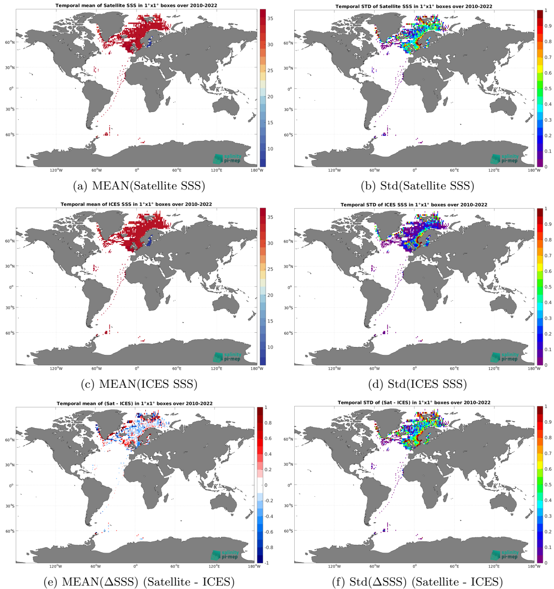
Figure 6: Temporal mean (left) and Std (right) of SSS from SMOS SSS L3 v8 - 9 Days (CATDS-CEC-LOCEAN) (top), ICES (middle), and of \Delta SSS (Satellite - ICES). Only match-up pairs are used to generate these maps.
