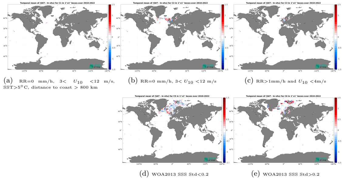
Figure 12: Temporal mean gridded over spatial boxes of size 1^\circ \times 1^\circ of \Delta SSS (SMOS SSS L3 v8 - 9 Days (CATDS-CEC-LOCEAN) - ICES) for 5 different subdatasets corresponding to:RR=0 mm/h, 3 < U_{10} < 12 m/s, SST > 5^\circ\text{C} , distance to coast > 800 km (a), RR=0 mm/h, 3 < U_{10} < 12 m/s (b), RR > 1 mm/h and U_{10} < 4 m/s (c), WOA2013 SSS Std < 0.2 (d), WOA2013 SSS Std > 0.2 (e).
